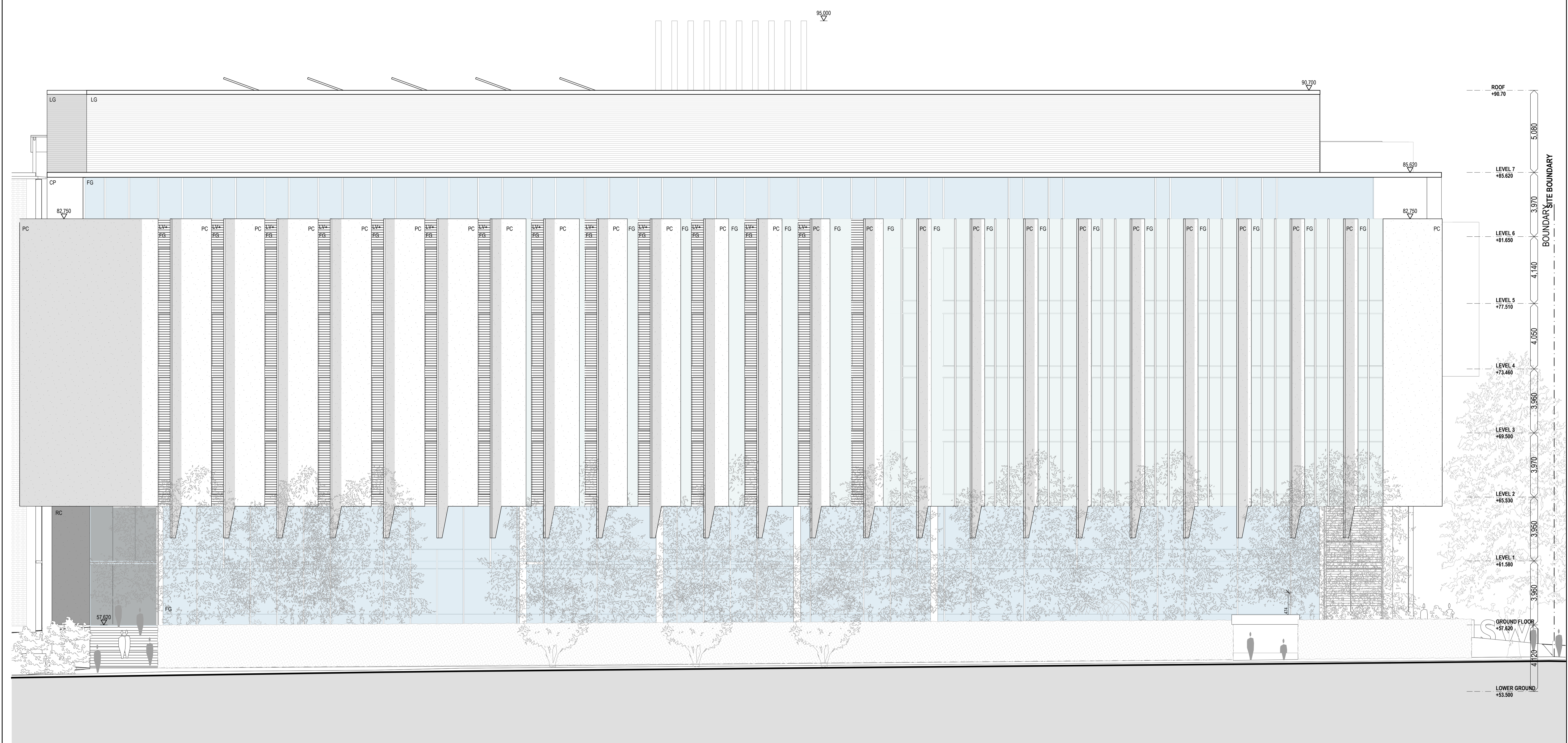
1 East Elevation - Botany Street 1:100
