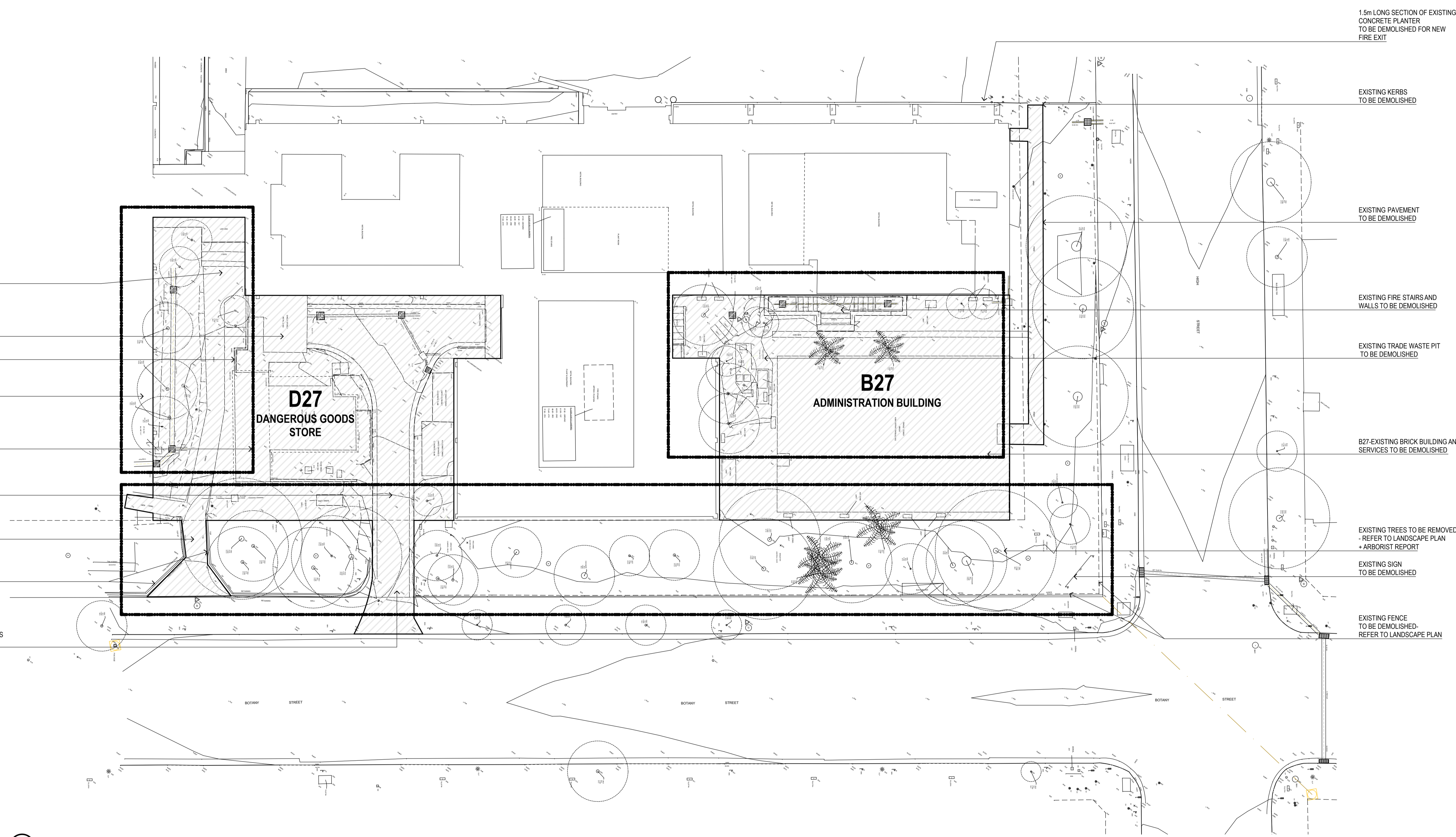
1 Demolition Plan 1:200
