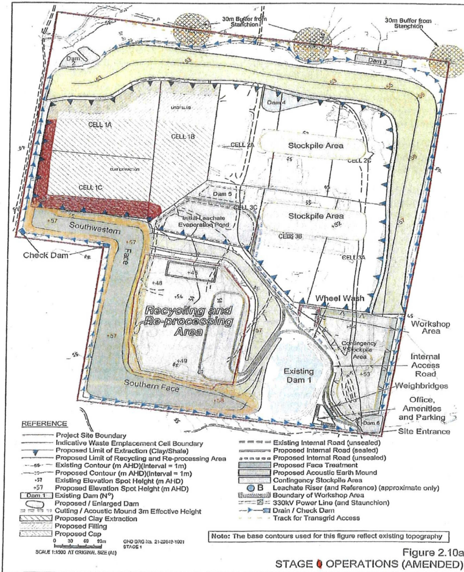
Figure 2.10a Stage 1 Operations
