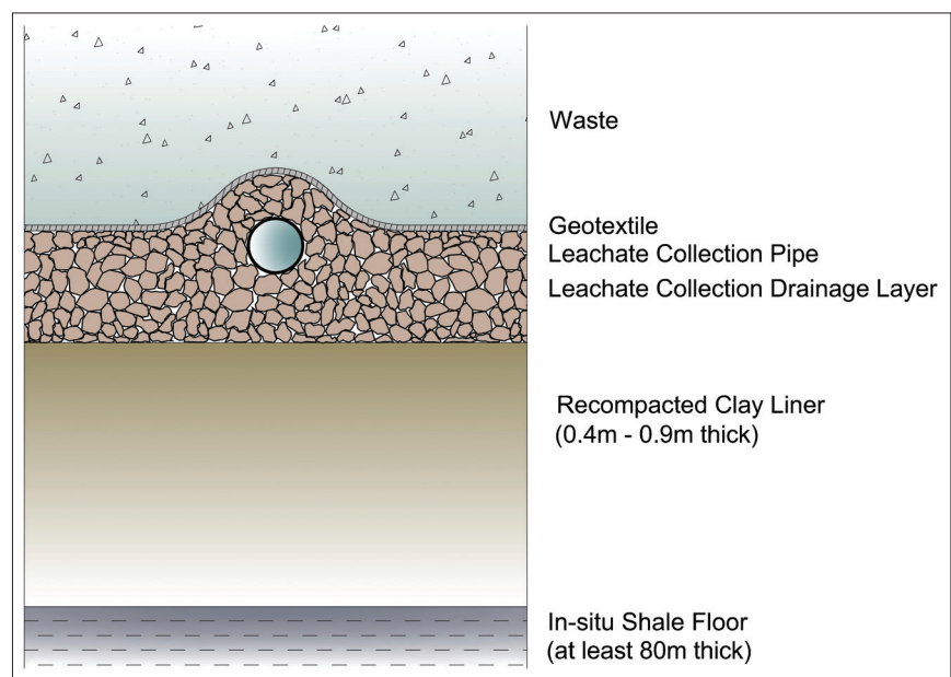
Geological cross-section of the landfill floor
