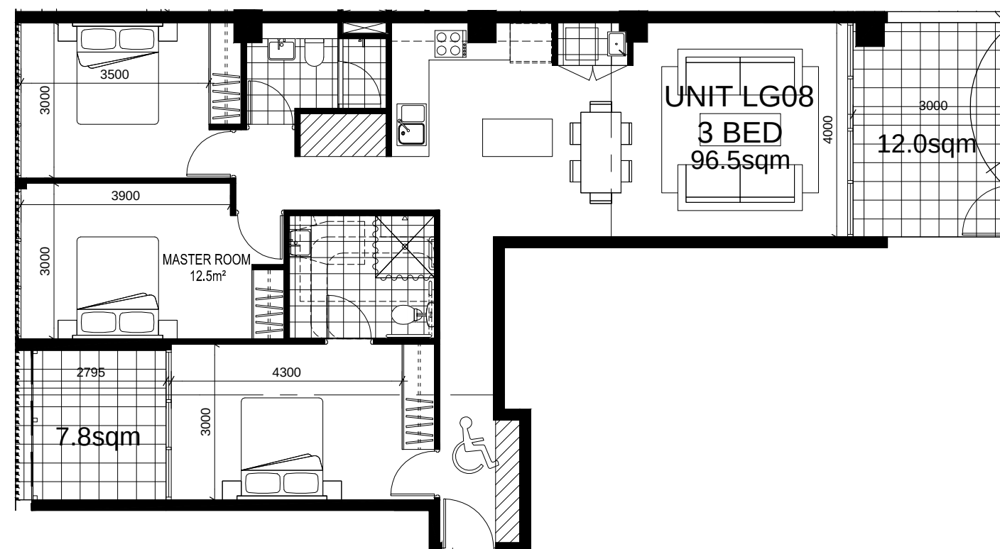
PRE-ADAPTABLE 3 BEDROOM UNIT LG08, G08
