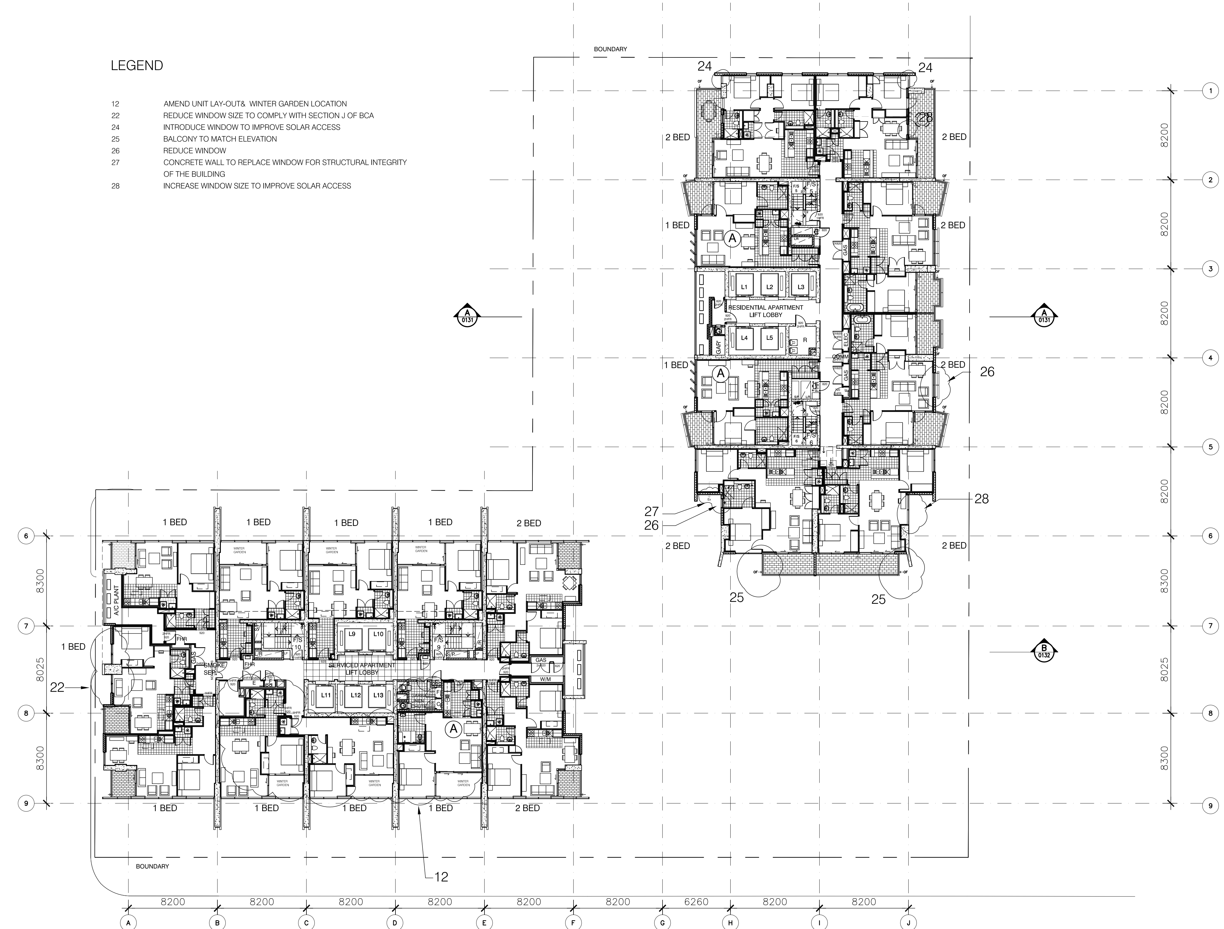
01 SERVICED APARTMENT LEVEL 5-8 PLAN 1:200
