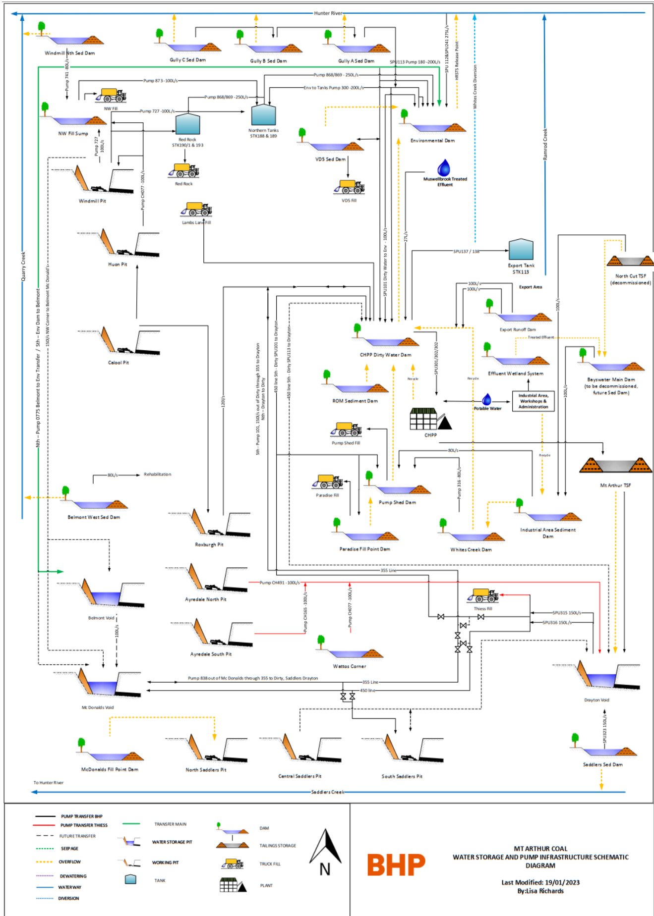
Figure 2: Water management schematic
