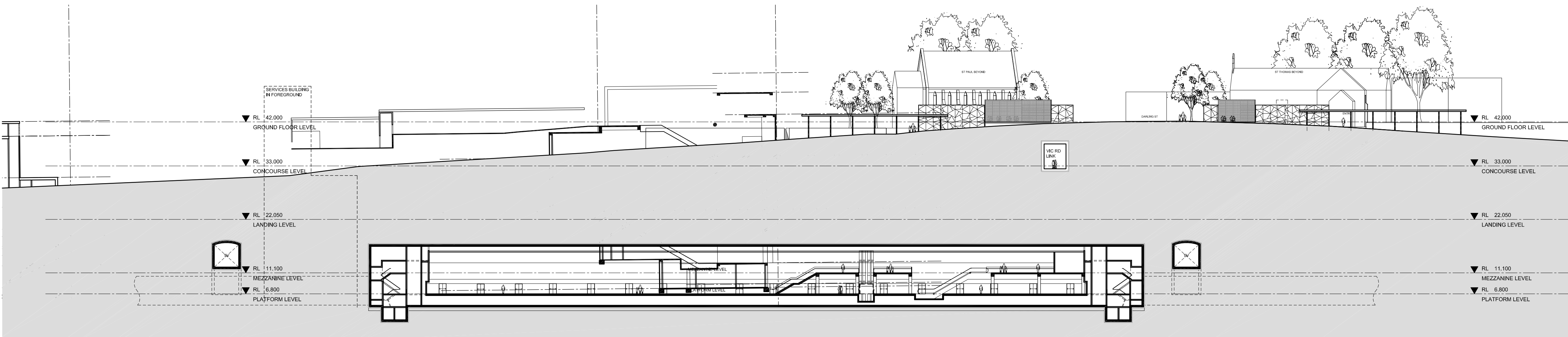
03 SECTION C-C 1:500
