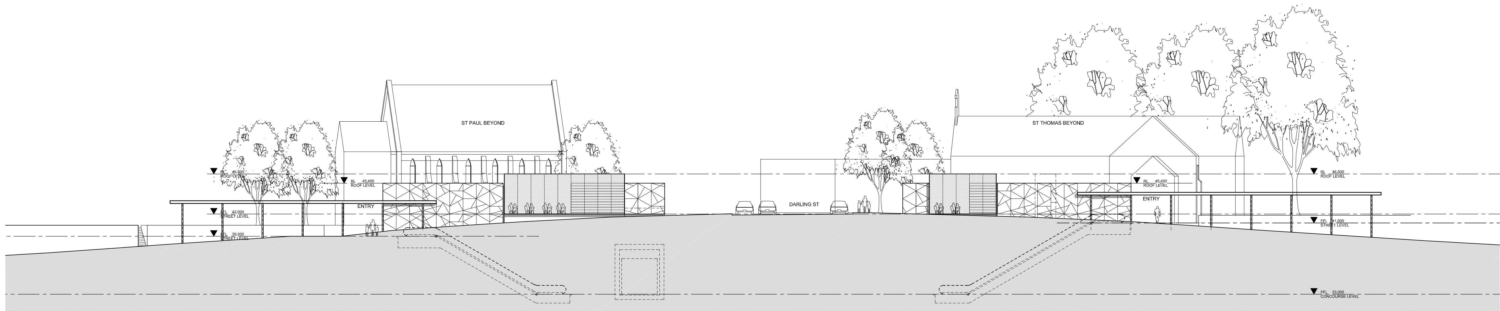
02 ELEVATION WEST - 1:250
