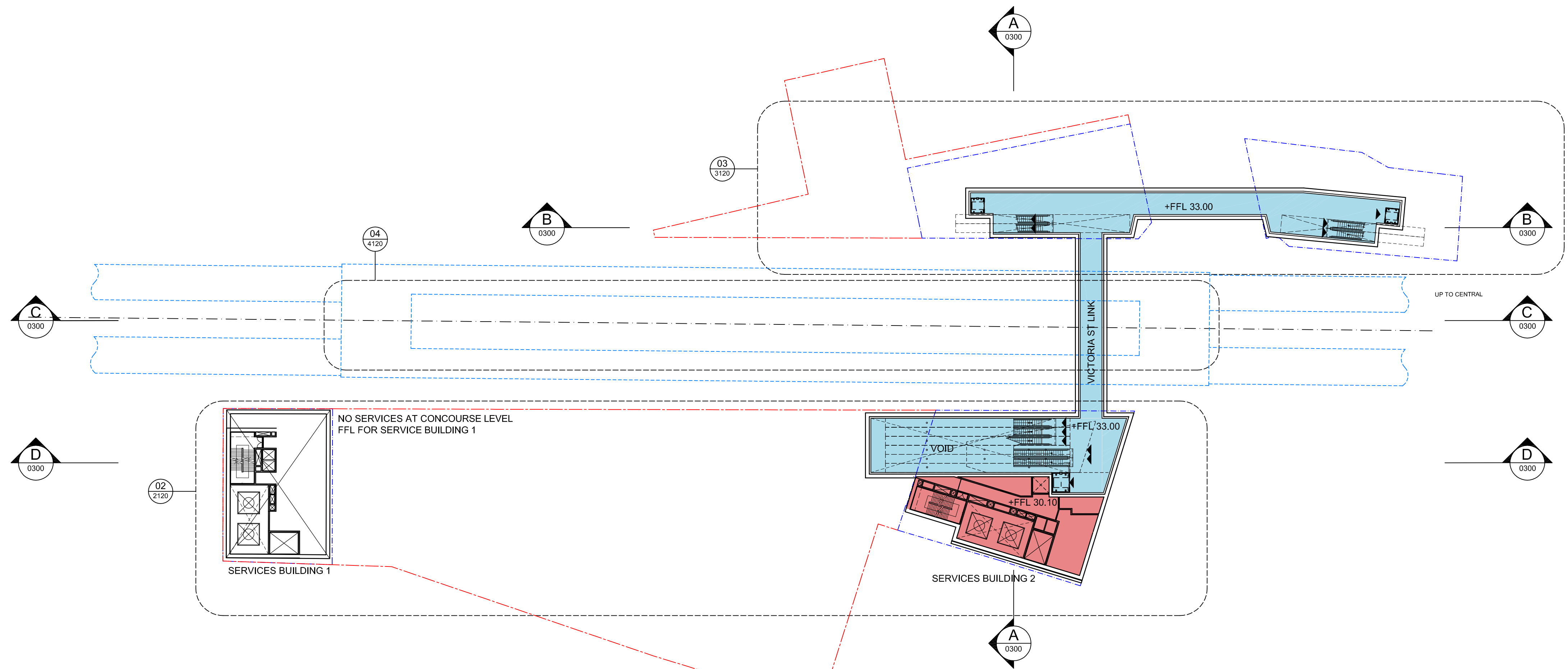
01 B1 CONCOURSE LEVEL PLAN - WEST FFL 33.0 / 30.1(PUBLIC/PLANT)
