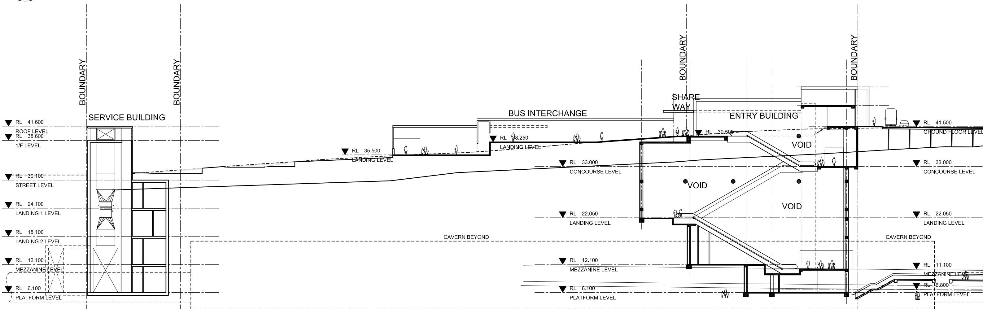
03 SECTION C-C 1:500
