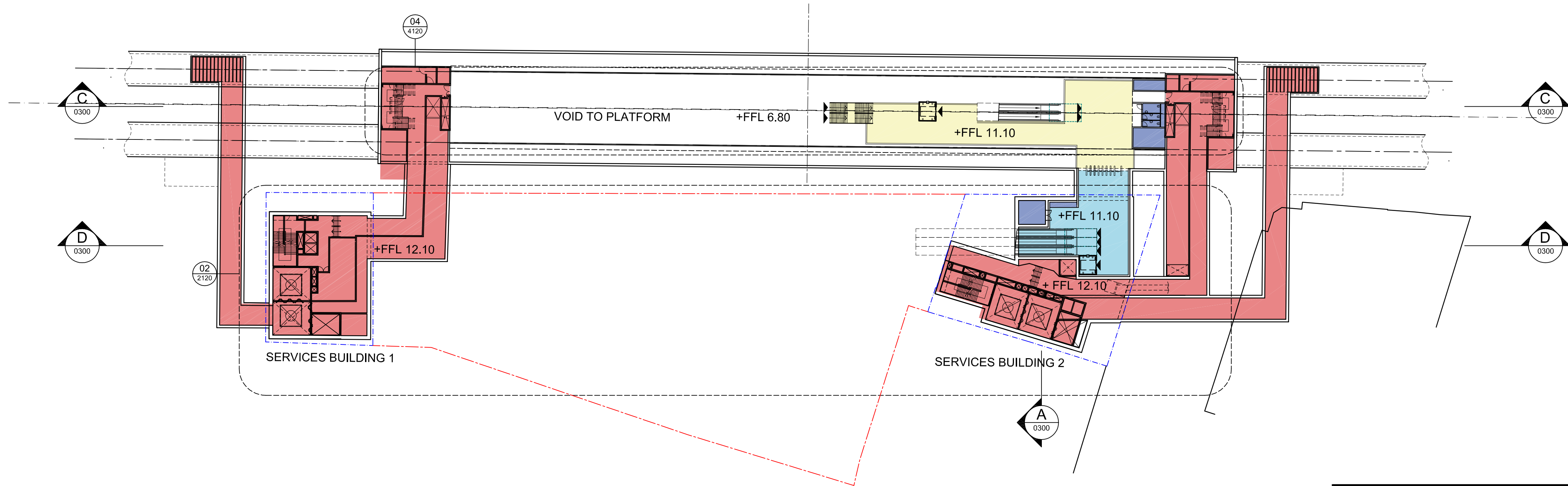
02 B4 MEZZANINE LEVEL PLAN - EAST FFL - 12.1/ 11.1 (PLANT / PUBLIC) - WEST FFL 12.1/ 11.1 (PLANT / PUBLIC)
