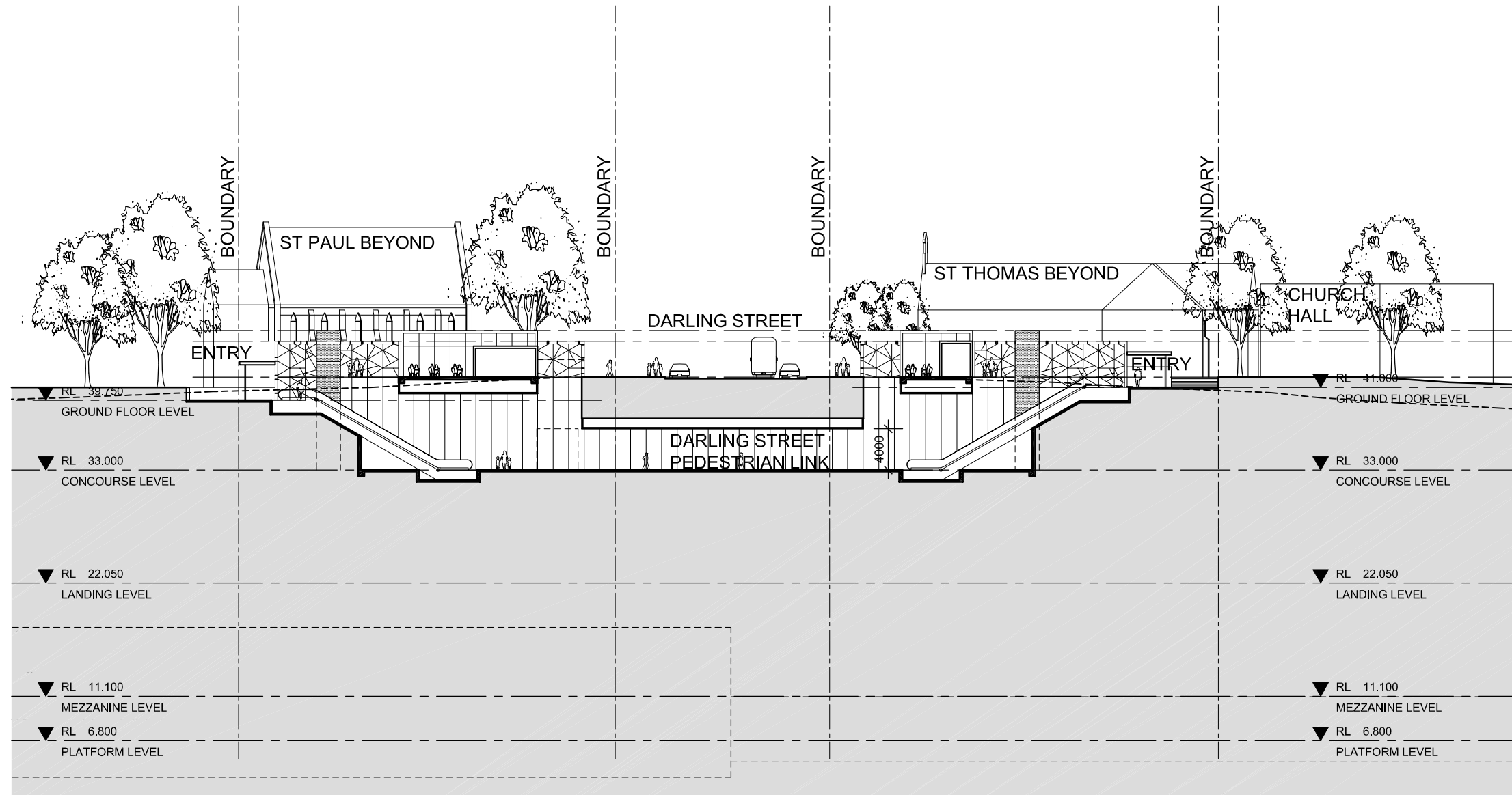
02 SECTION B-B 1:500
