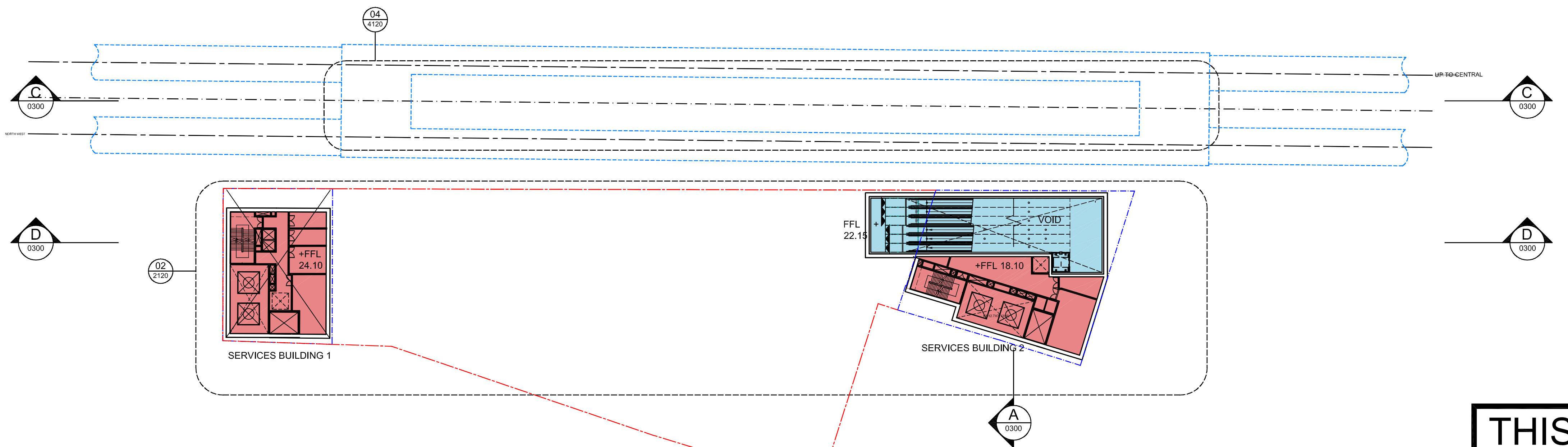
02 B2 LANDING LEVEL PLAN - EAST FFL - 24.1 (PLANT) WEST FFL 24.1 (PLANT)
