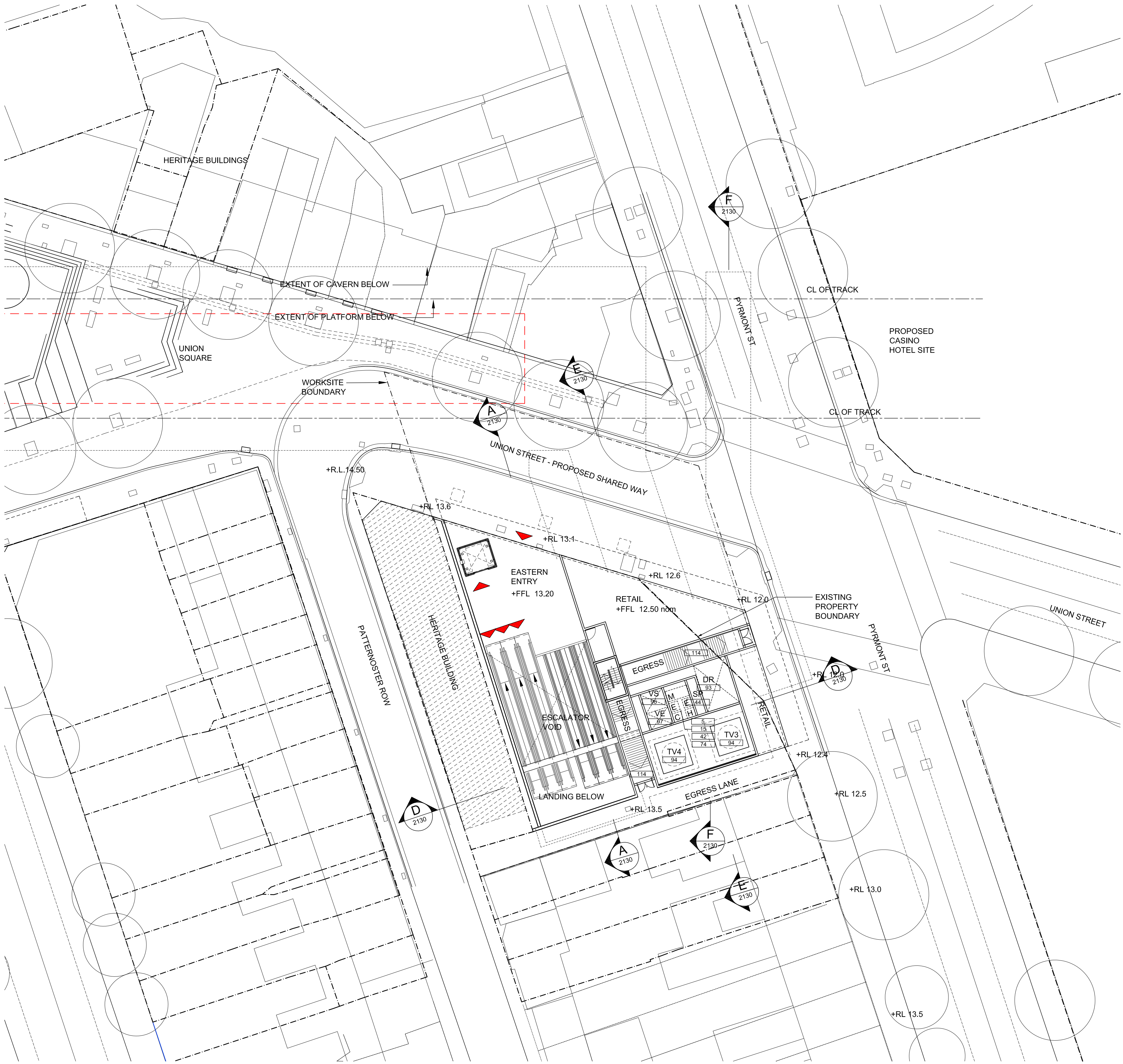
01 SERVICE BUILDING 01 - ENTRY LEVEL - RL 13.20 nom
