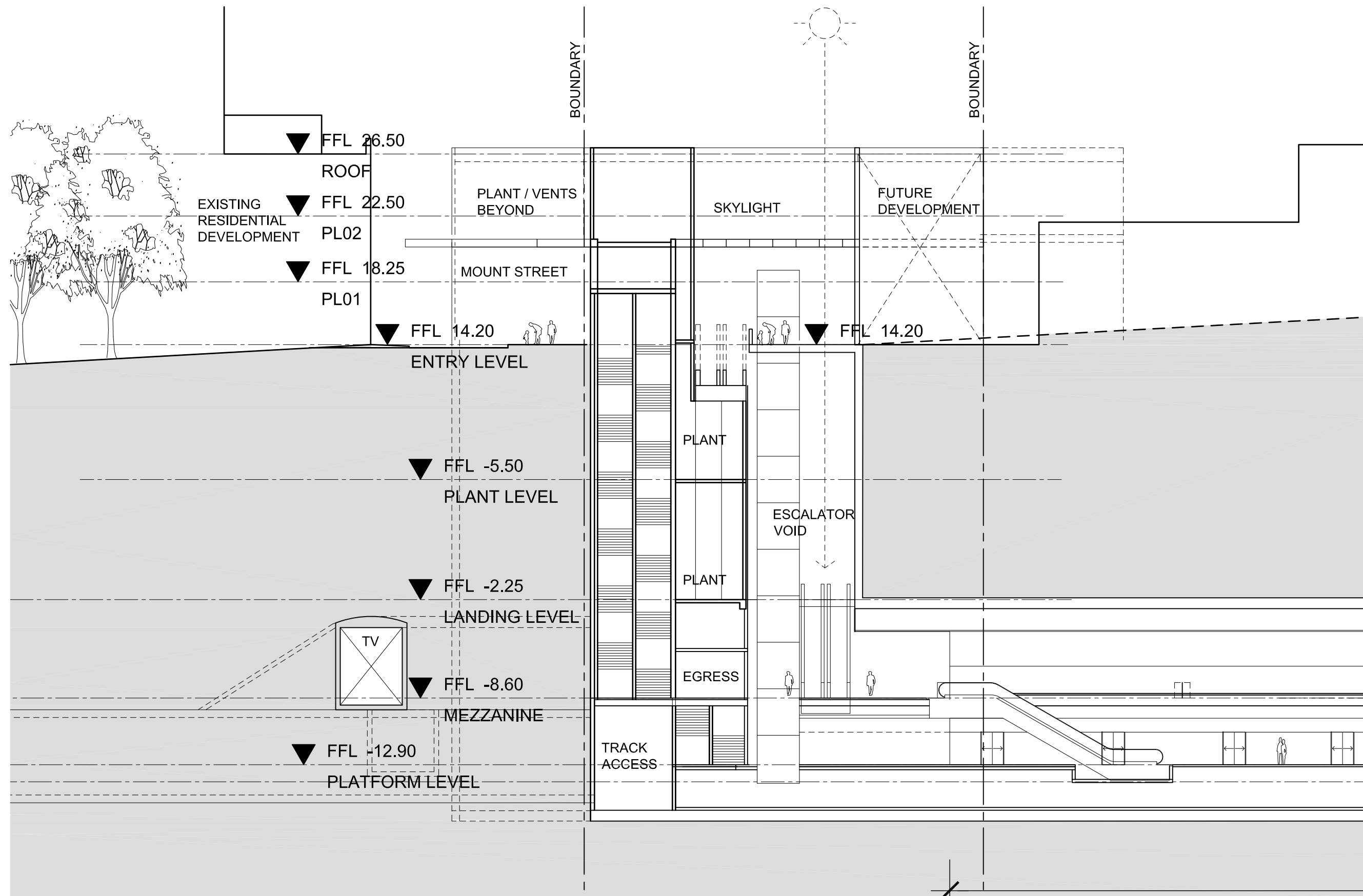
BB WESTERN ENTRY 0200
