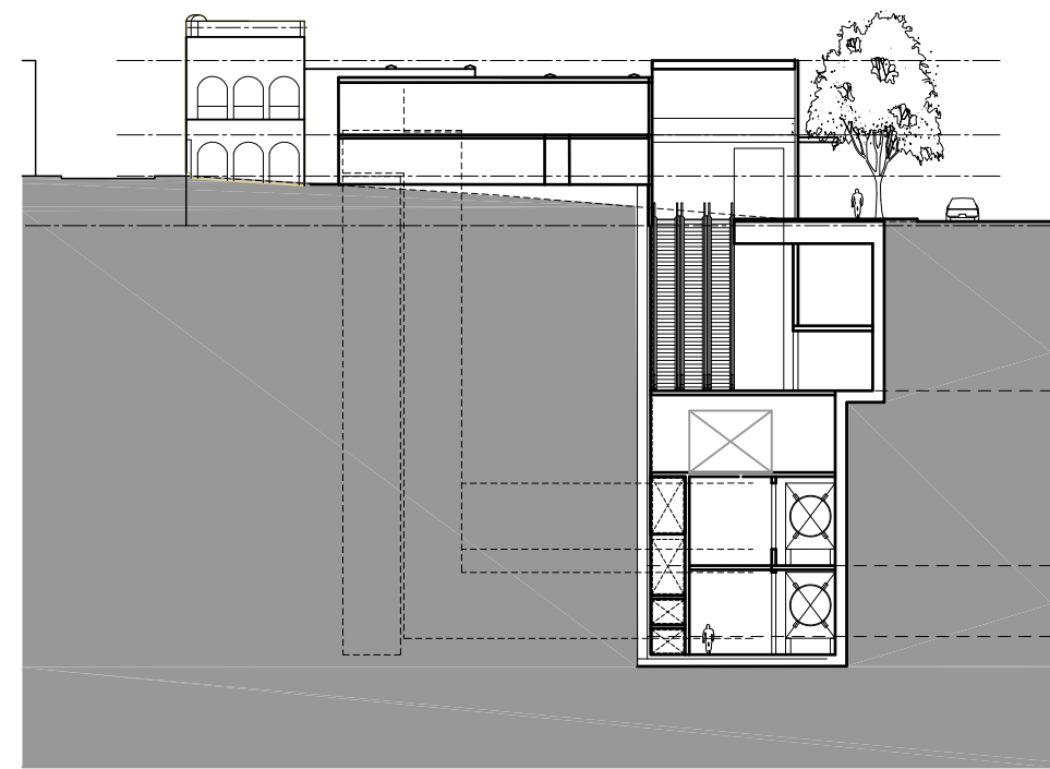
BB EASTERN ENTRY - CROSS SECTION 0200
