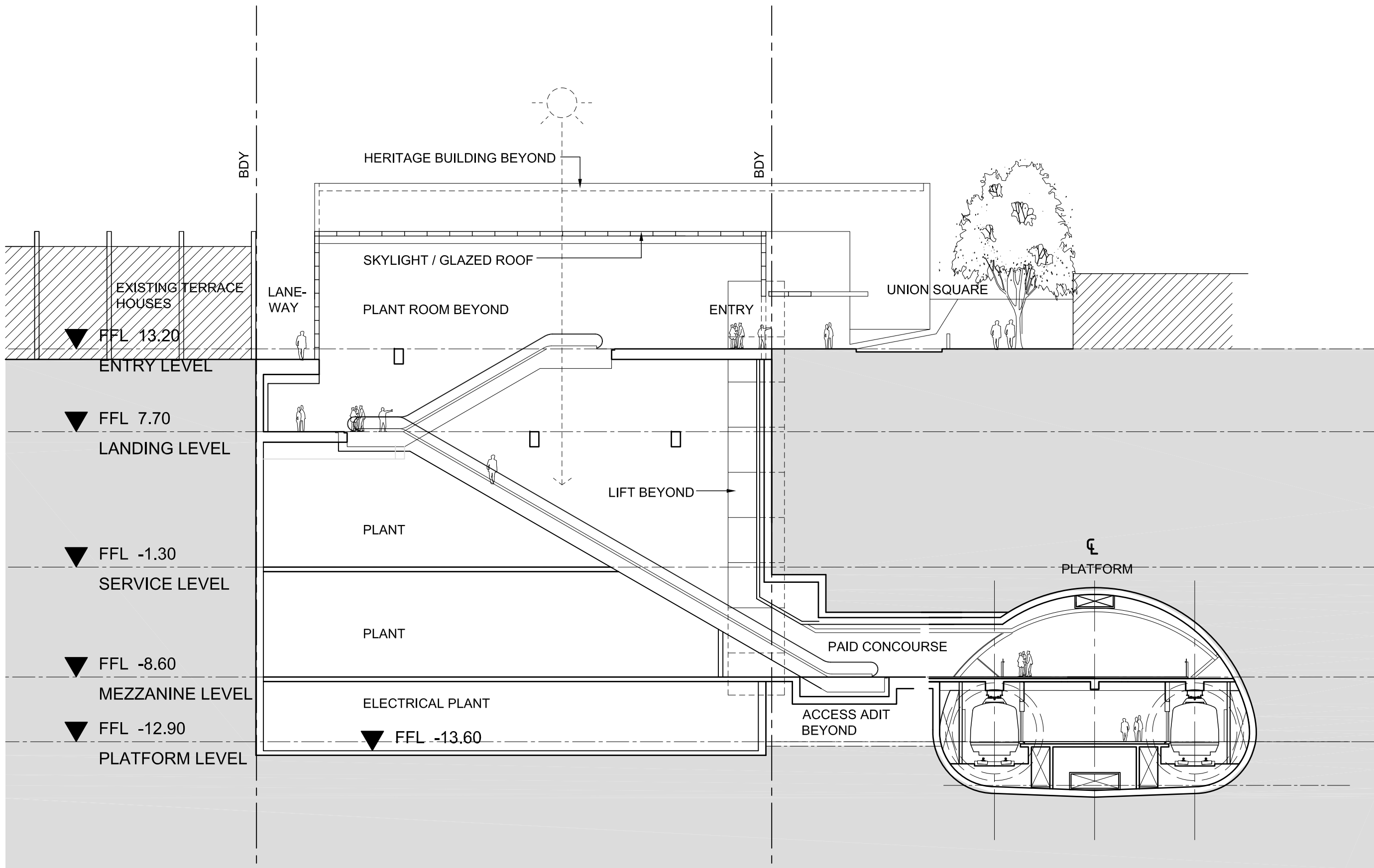
AA SERVICE BUILDING 02 - EASTERN ENTRY 0200
