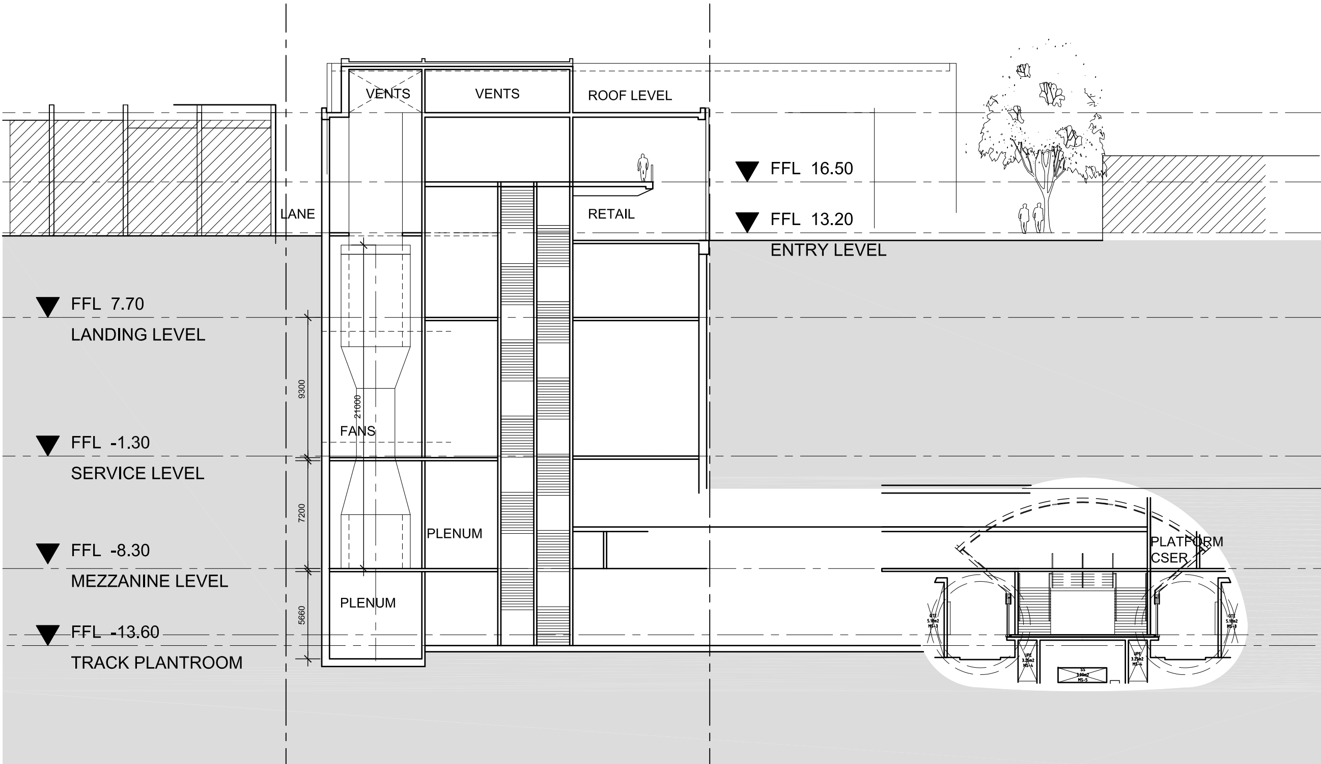
EE SERVICE BUILDING 02 0200
