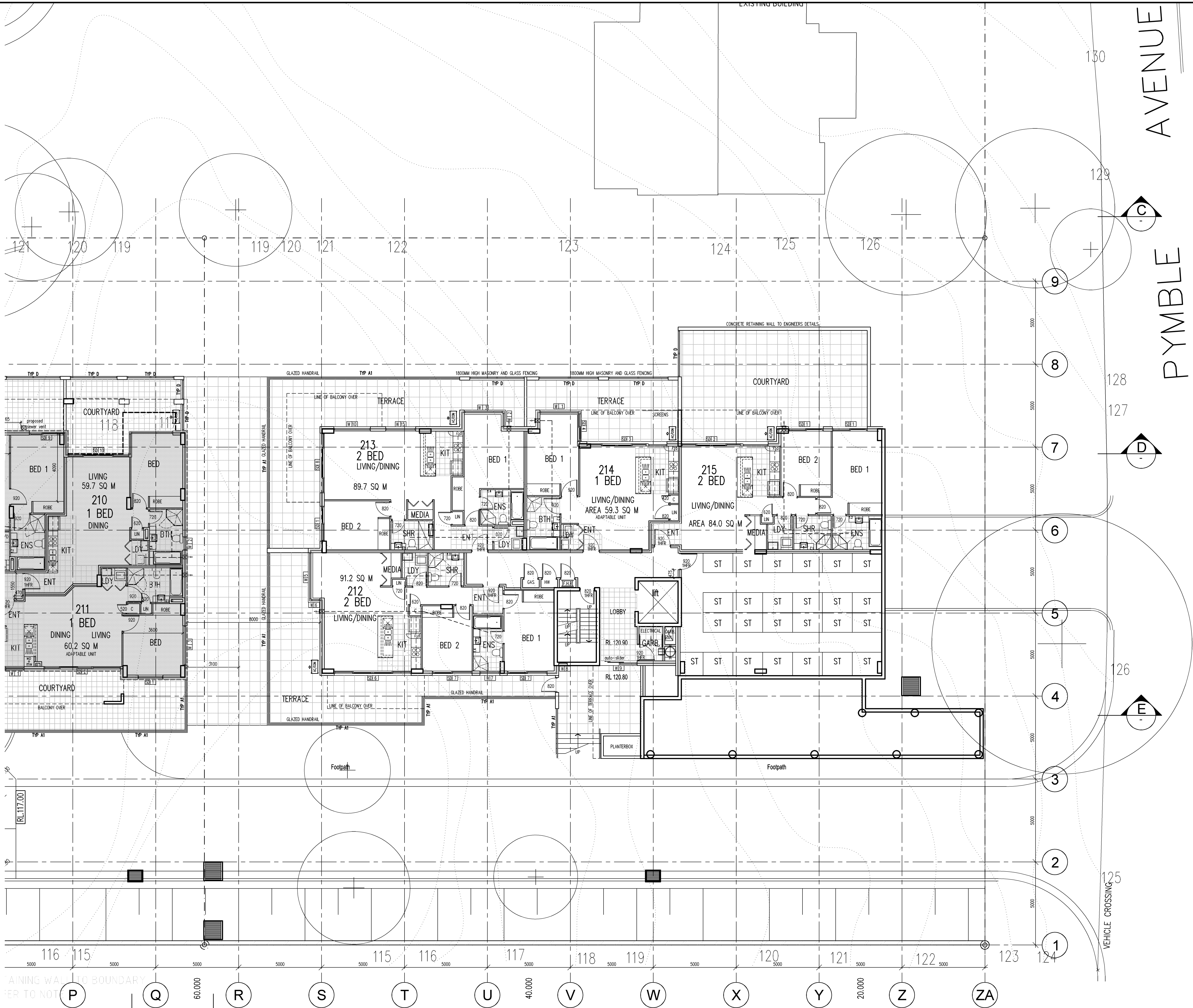
E LEVEL 02 - ARCH 100 SCALE 1:100
