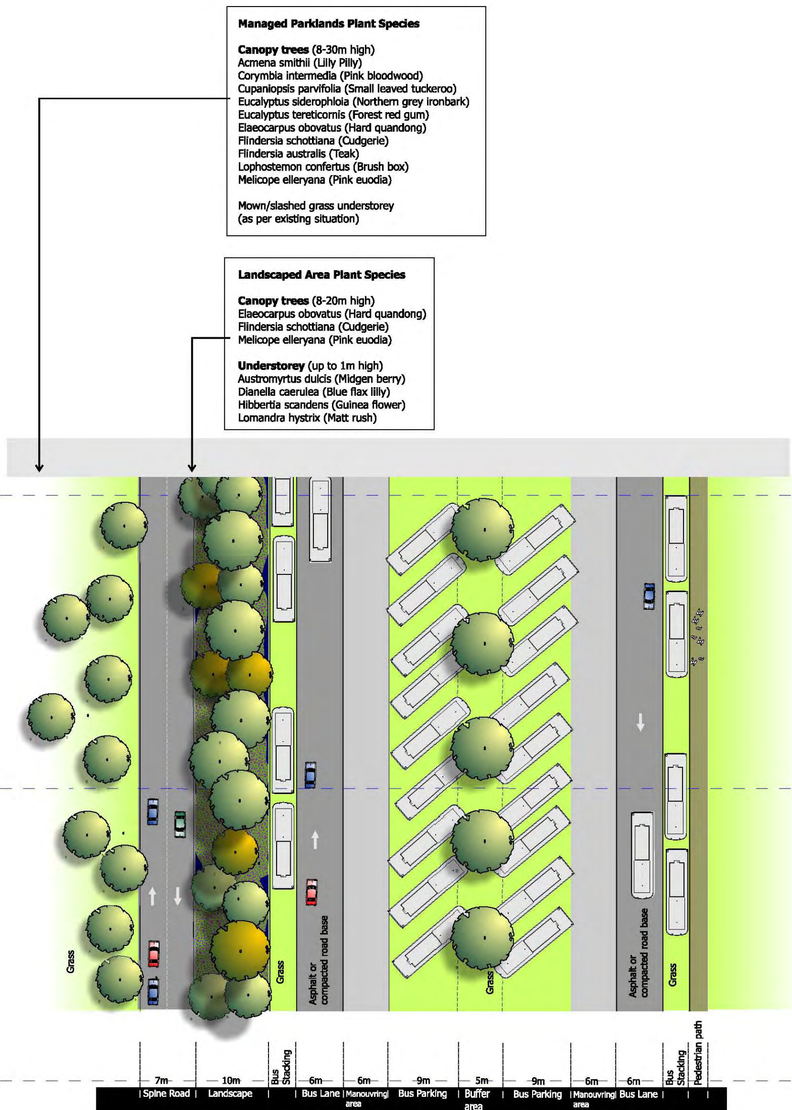
Typical Design Bus Loading Area Plan
