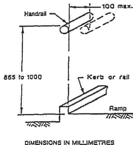
FIGURE 3 - LOCATION OF KERB IN RELATION TO HANDRAIL
