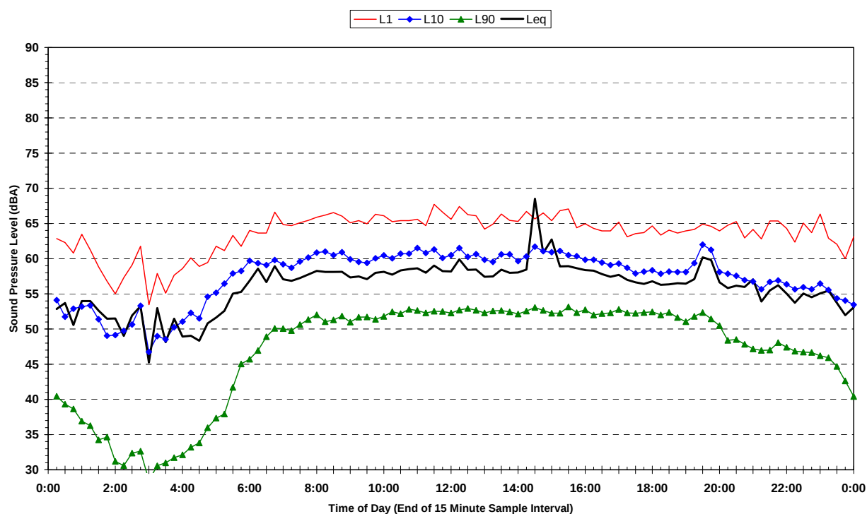
S3-2 - 4 Sommerset Street - Long-Term Statistical Noise Levels Wednesday 26 March 2008 to Thursday 3 April 2008
