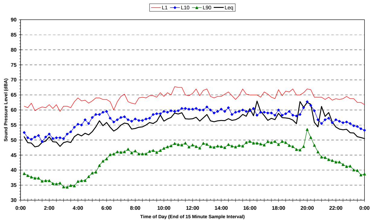
S1-6 - 17 Livingstone Avenue - Long-Term Statistical Noise Levels Tuesday 4 March 2008 to Wednesday 5 March 2008
