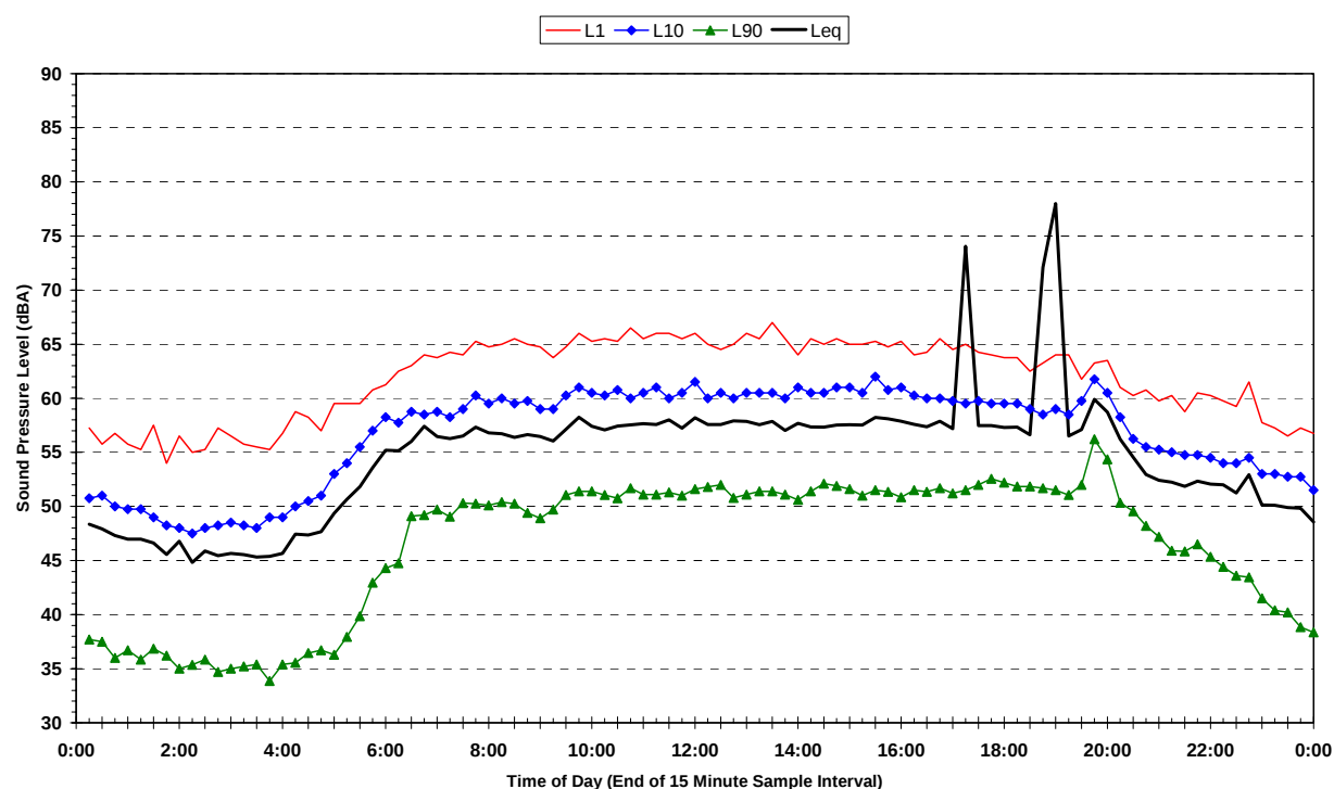
S2-7 - 5 Orchard Road - Long-Term Statistical Noise Levels Wednesday 12 March 2008 to Friday 14 March 2008
