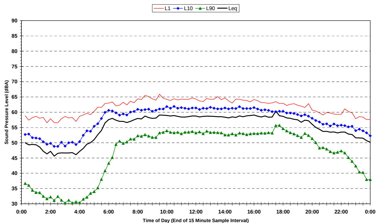
S2-8 - 24 A Castle Howard Road - Long-Term Statistical Noise Levels Wednesday 12 March 2008 to Friday 14 March 2008
