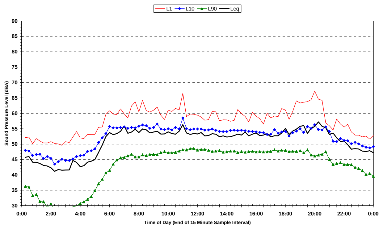
S3-12 - 8 of 150 Crimea Road - Long-Term Statistical Noise Levels Tuesday 16 December 2008 to Monday 22 December 2008
