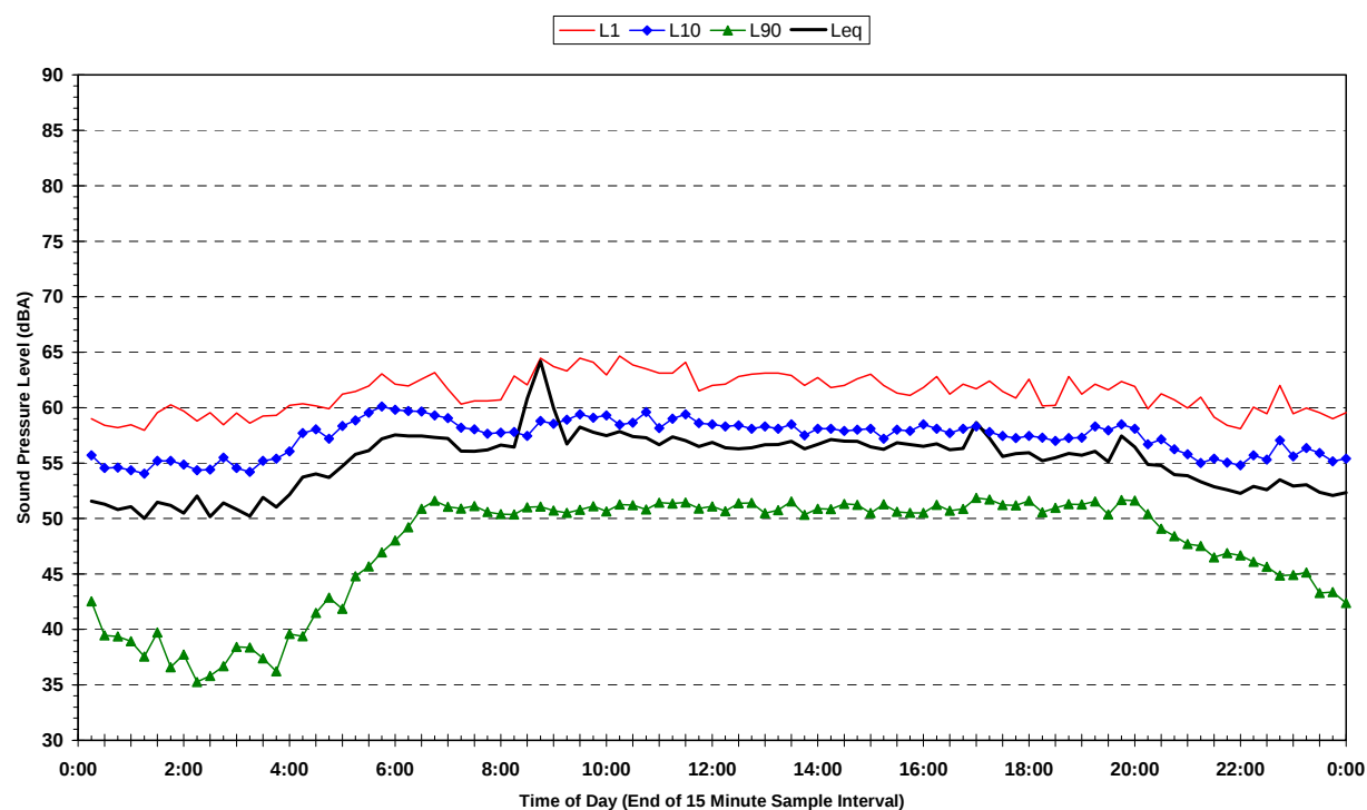
S2-2 - 10 Virginia Place - Long-Term Statistical Noise Levels Wednesday 12 March 2008 to Friday 14 March 2008
