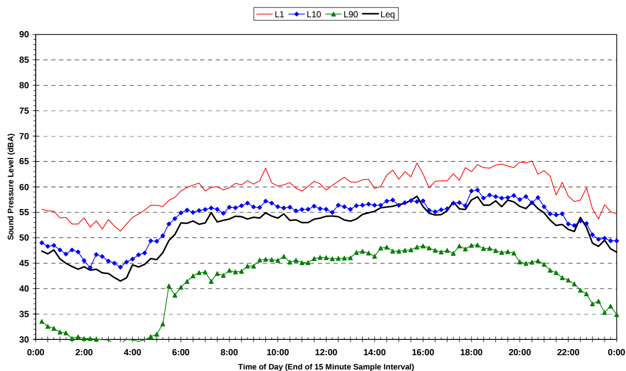
S3-13 - 24 of 2-4 Nile Close - Long-Term Statistical Noise Levels Friday 5 December 2008 to Sunday 14 December 2008
