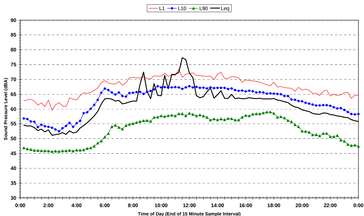
S3-1 - 30 Dunmore Road - Long-Term Statistical Noise Levels Thursday 8 May 2008 to Thursday 15 May 2008
