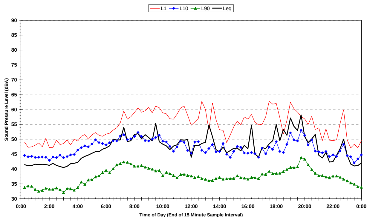
S2-1 - 12 Mill Drive - Long-Term Statistical Noise Levels Wednesday 12 March 2008 to Thursday 20 March 2008
