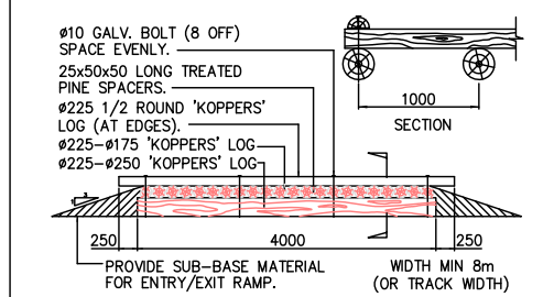
LONG TERM CONSTRUCTION SITE ENTRY/EXIT
