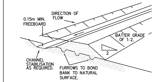
DIVERSION BANK AND SWALE 1
