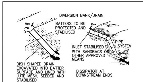
SLOPE DRAINAGE ON EMBANKMENTS / BATTERS
