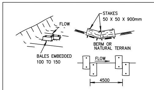
STRAW BALE CHECK DAM
