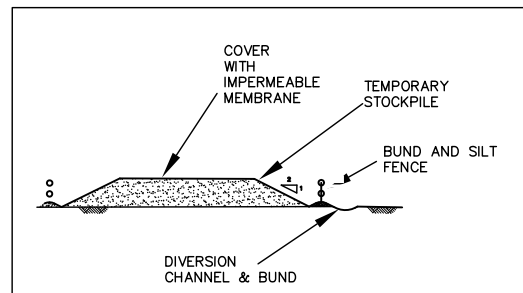
TYPICAL TEMPORARY STOCKPILE
