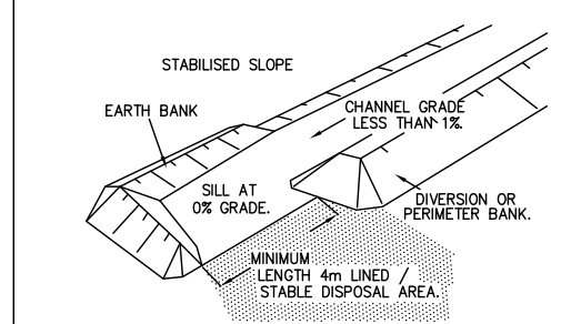
LEVEL SPREADER (OR SILL)
