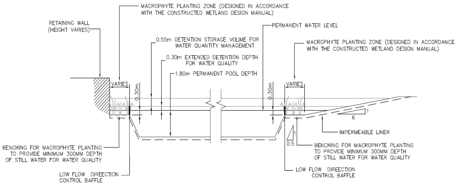
TYPICAL BASIN CROSS-SECTION
