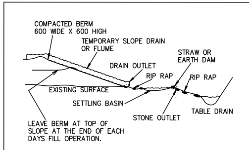
EMBANKMENT CONSTRUCTION
