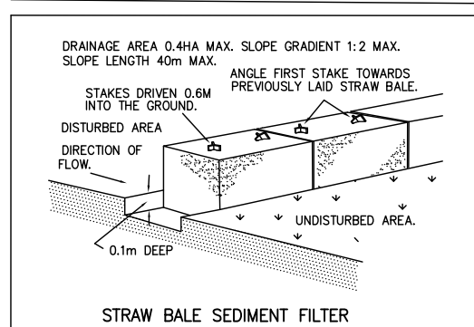
STRAW BALE SEDIMENT FILTER
