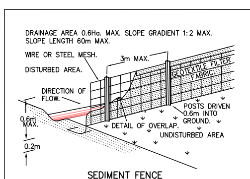
SEDIMENT FENCE
