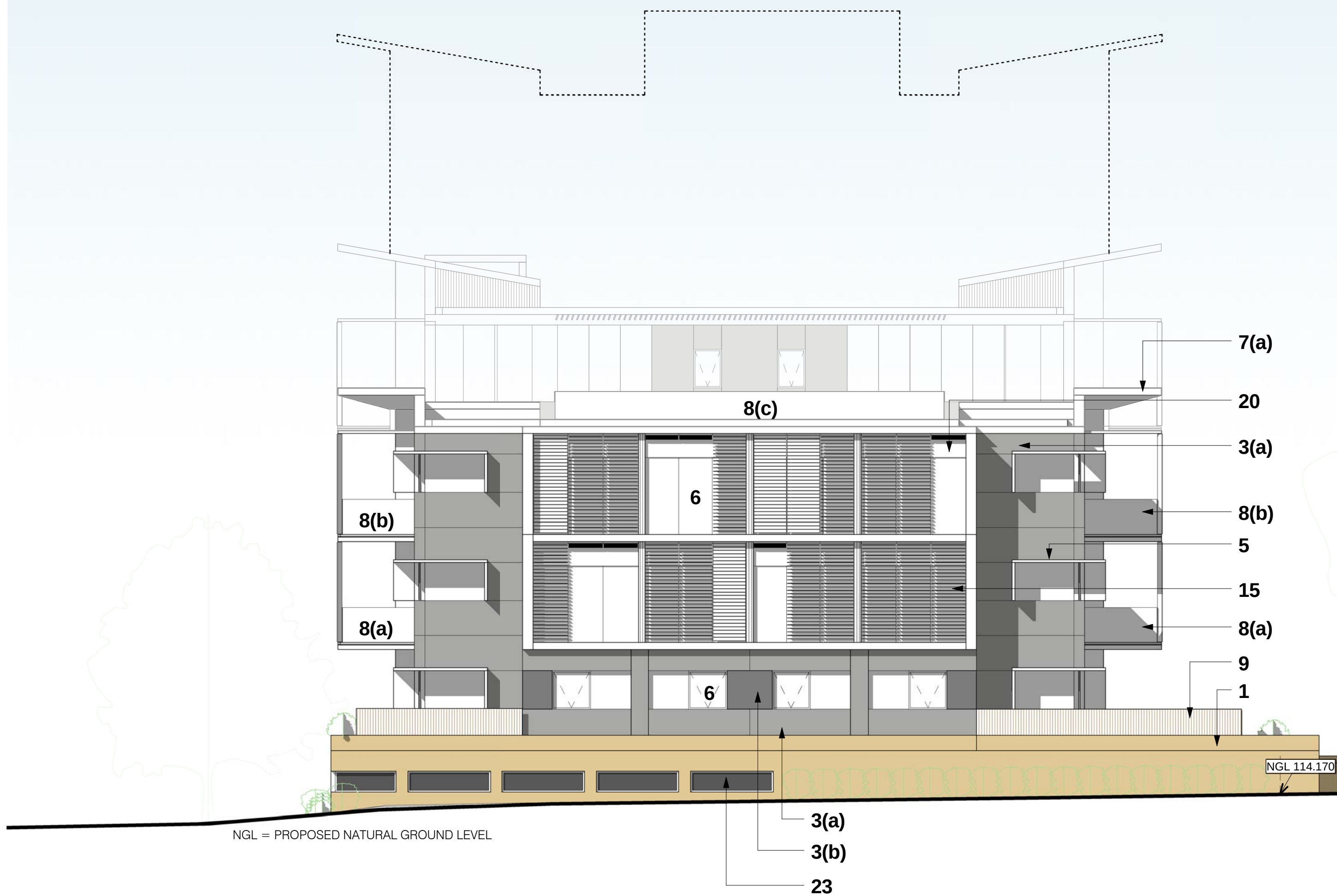
Building 5 Elevation South SHADOWS SHOWN INDICATIVELY ONLY
