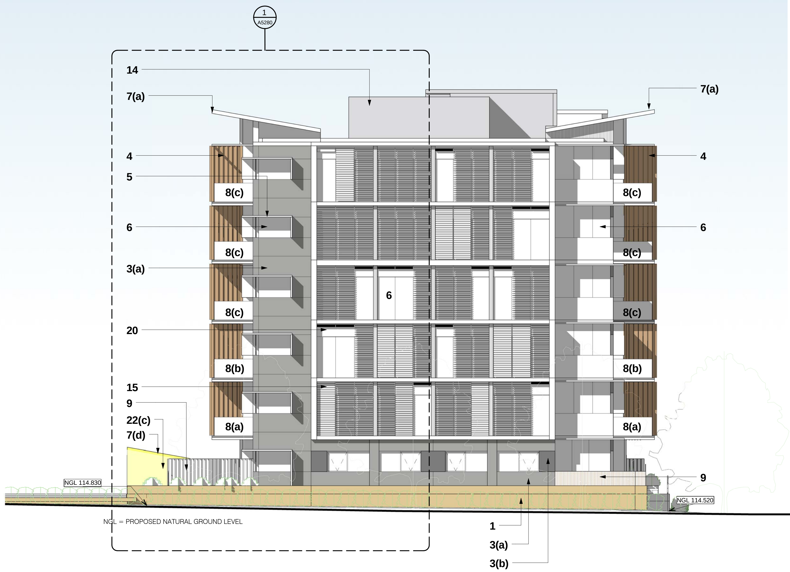
Building 5 Elevation North SHADOWS SHOWN INDICATIVELY ONLY
