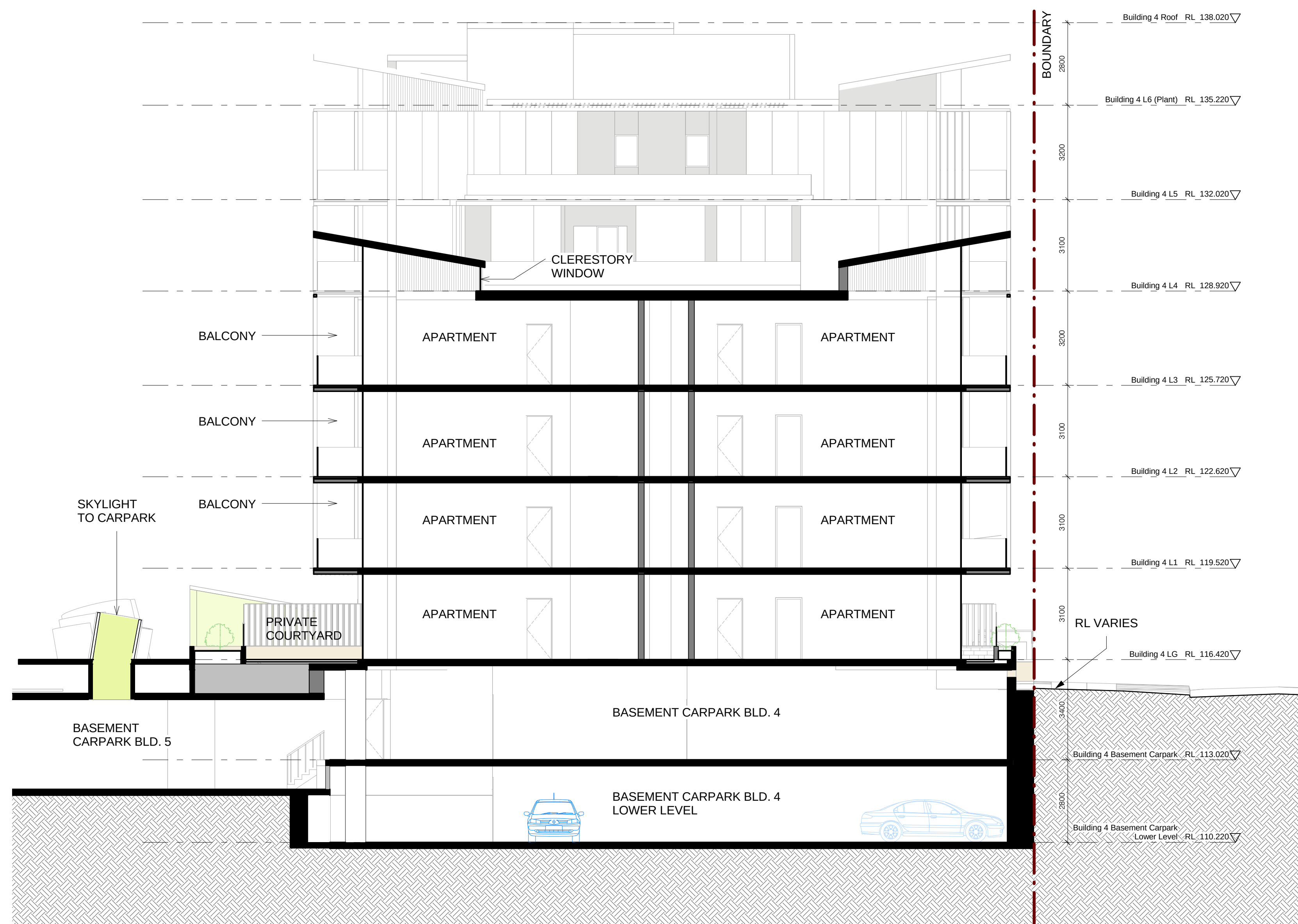
F Building 4 Section F 1 : 100@A0
