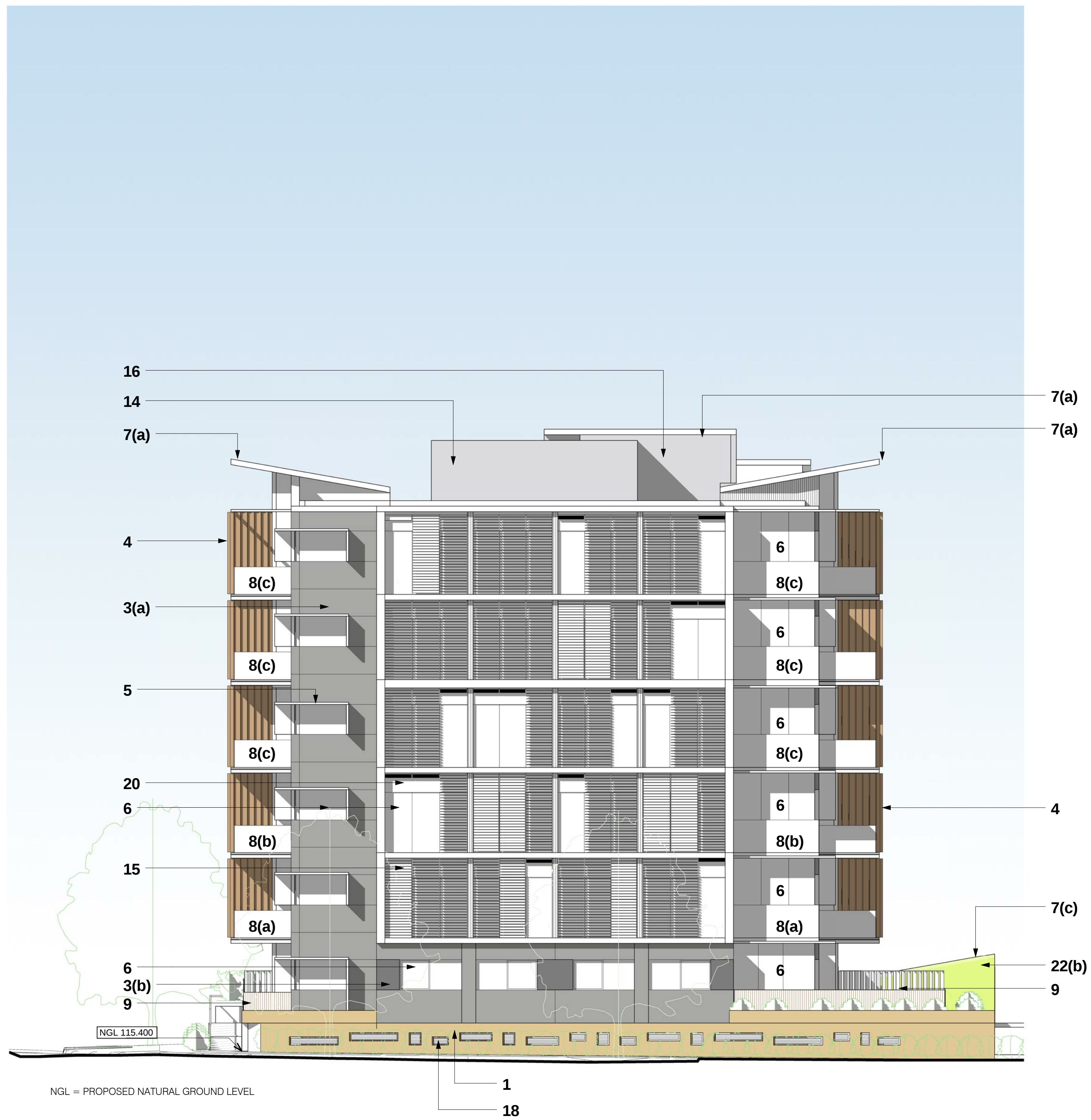
Building 4 North Elevation
