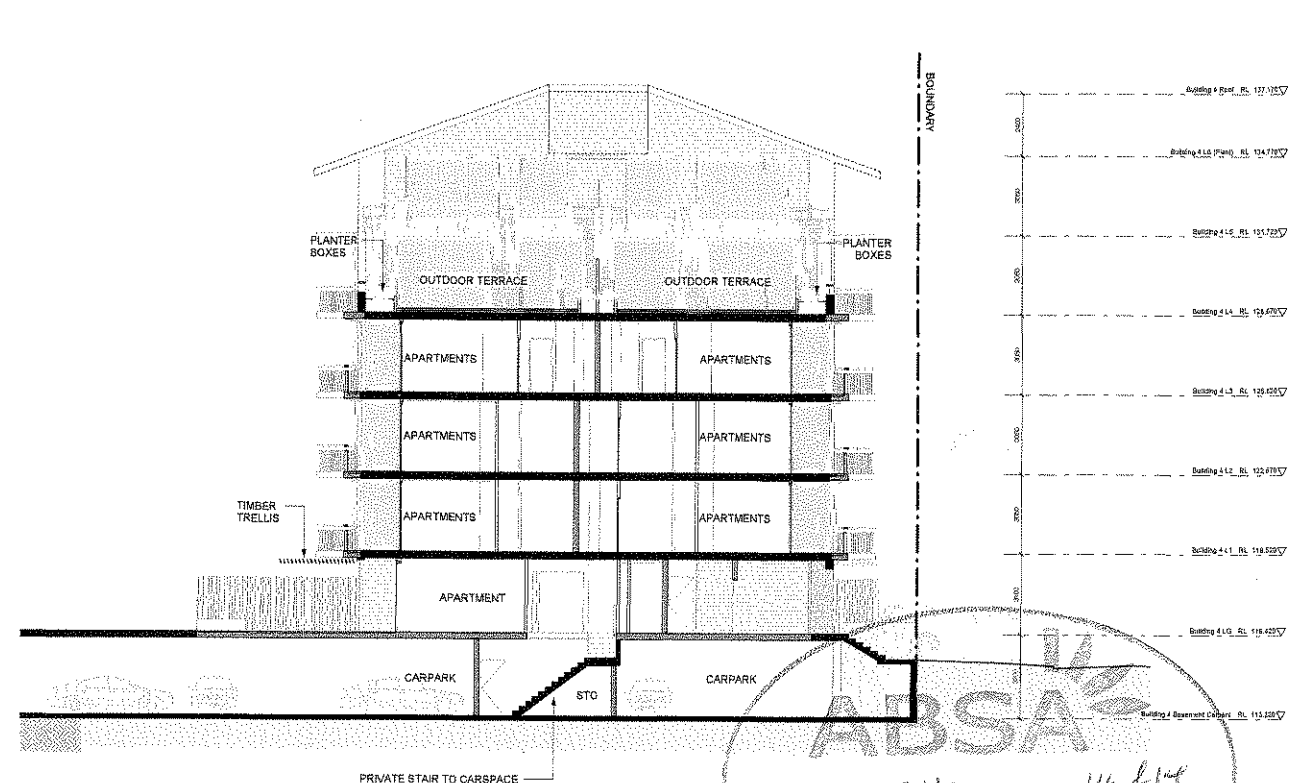
H Building 4 Section H 1: 100 @ A0
