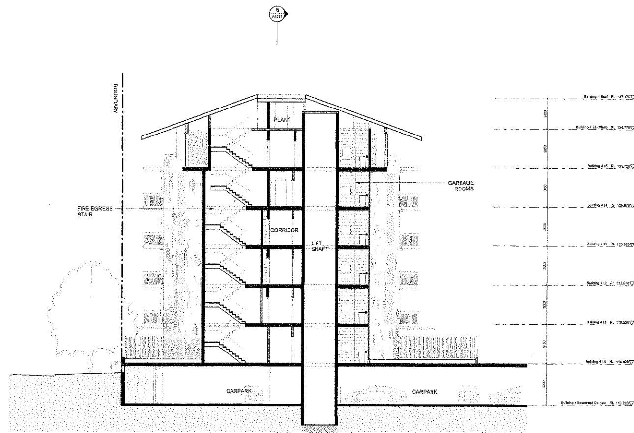
E Building 4 Section E 1: 100 @ A0
