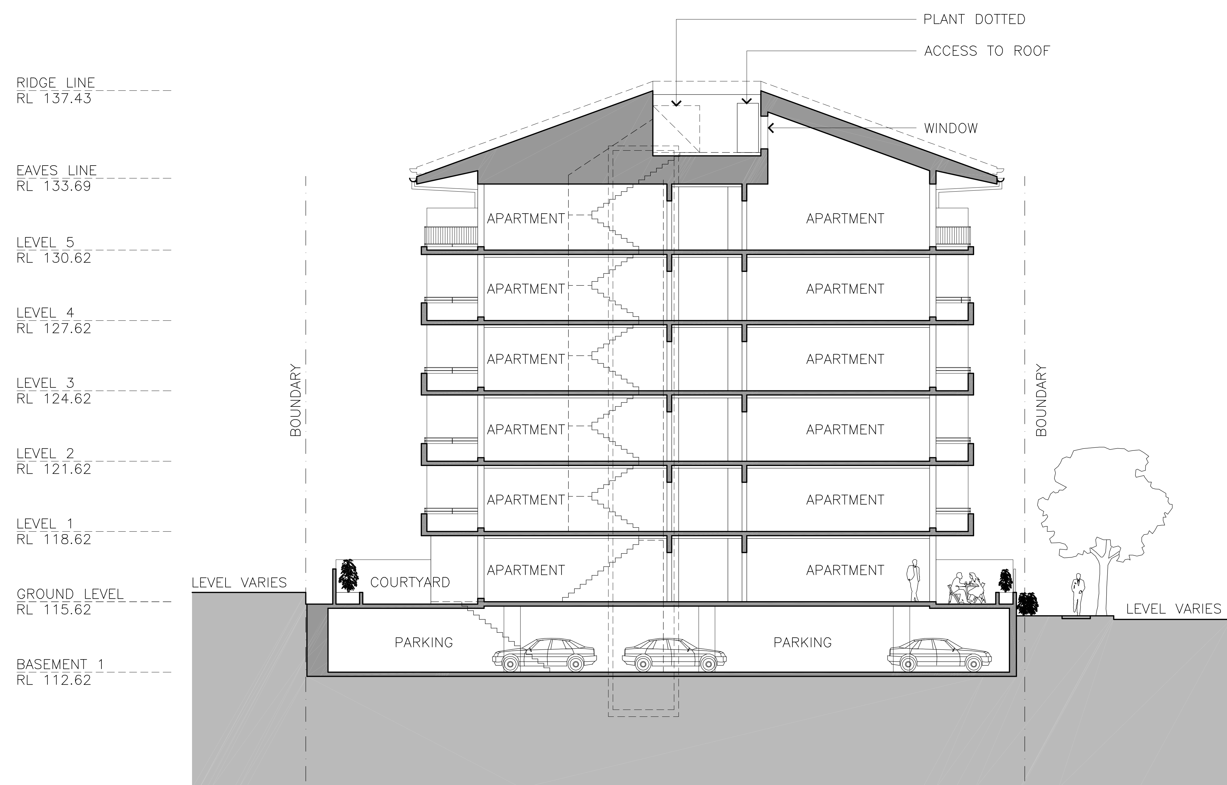
Section AA
