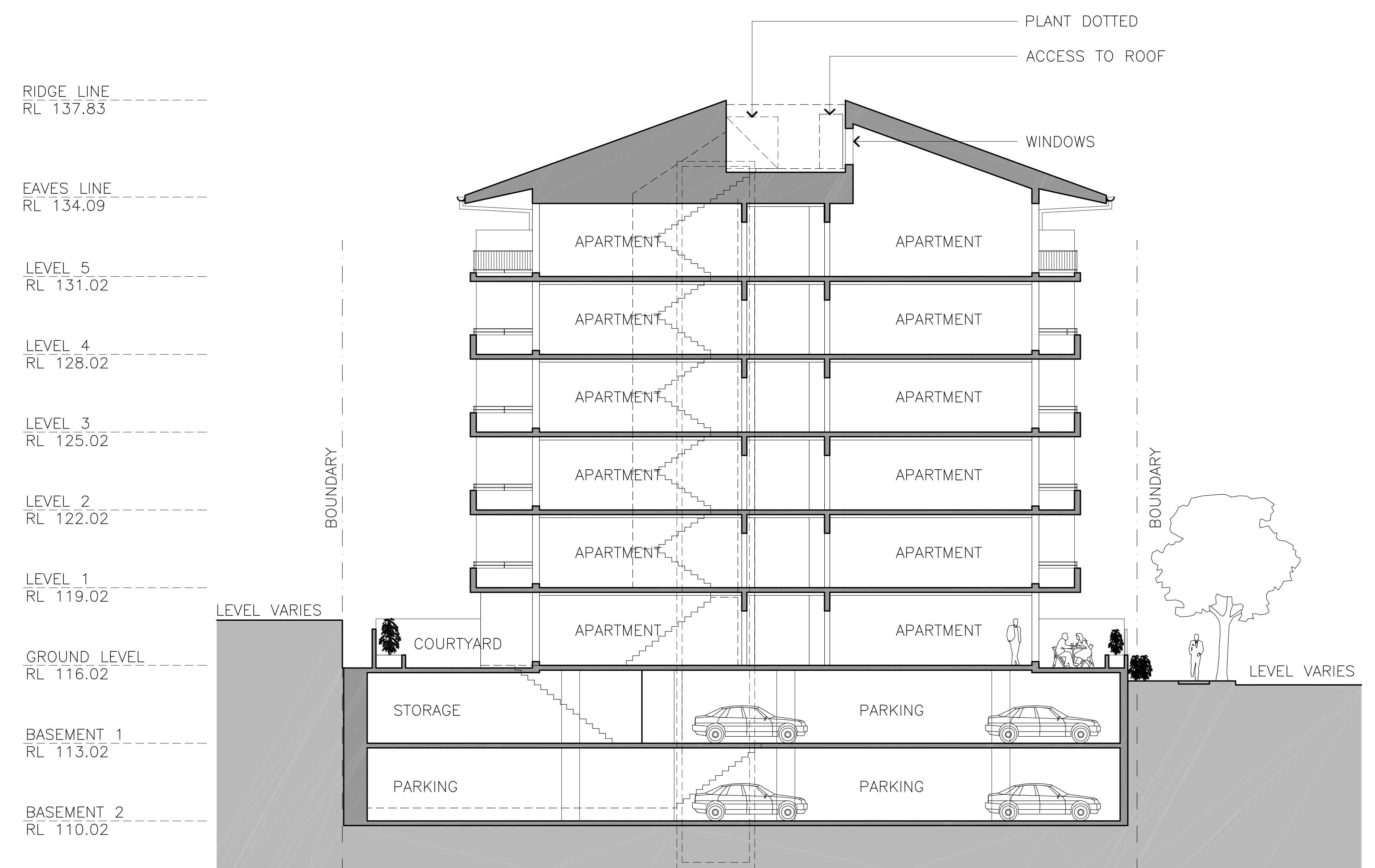
Section BB
