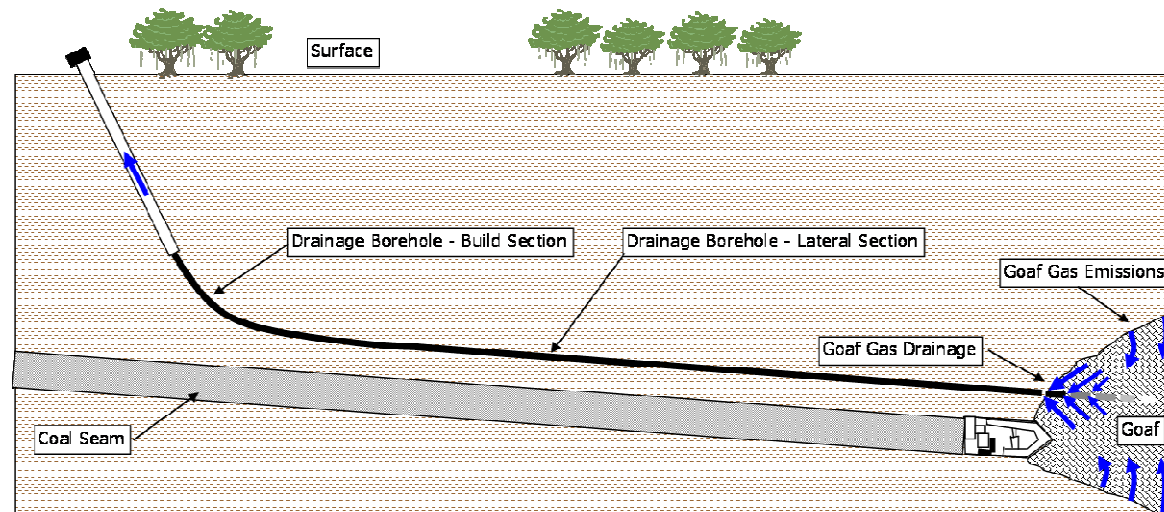
Figure 6 Schematic of Goaf Gas formation during longwall mining and MRD borehole
