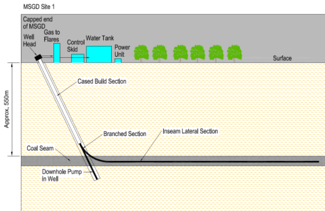
Figure 7 Schematic of MSGD Well #1
