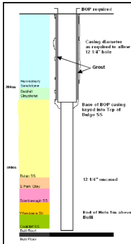
Figure 10 Example of Grout in Vertical Borehole
