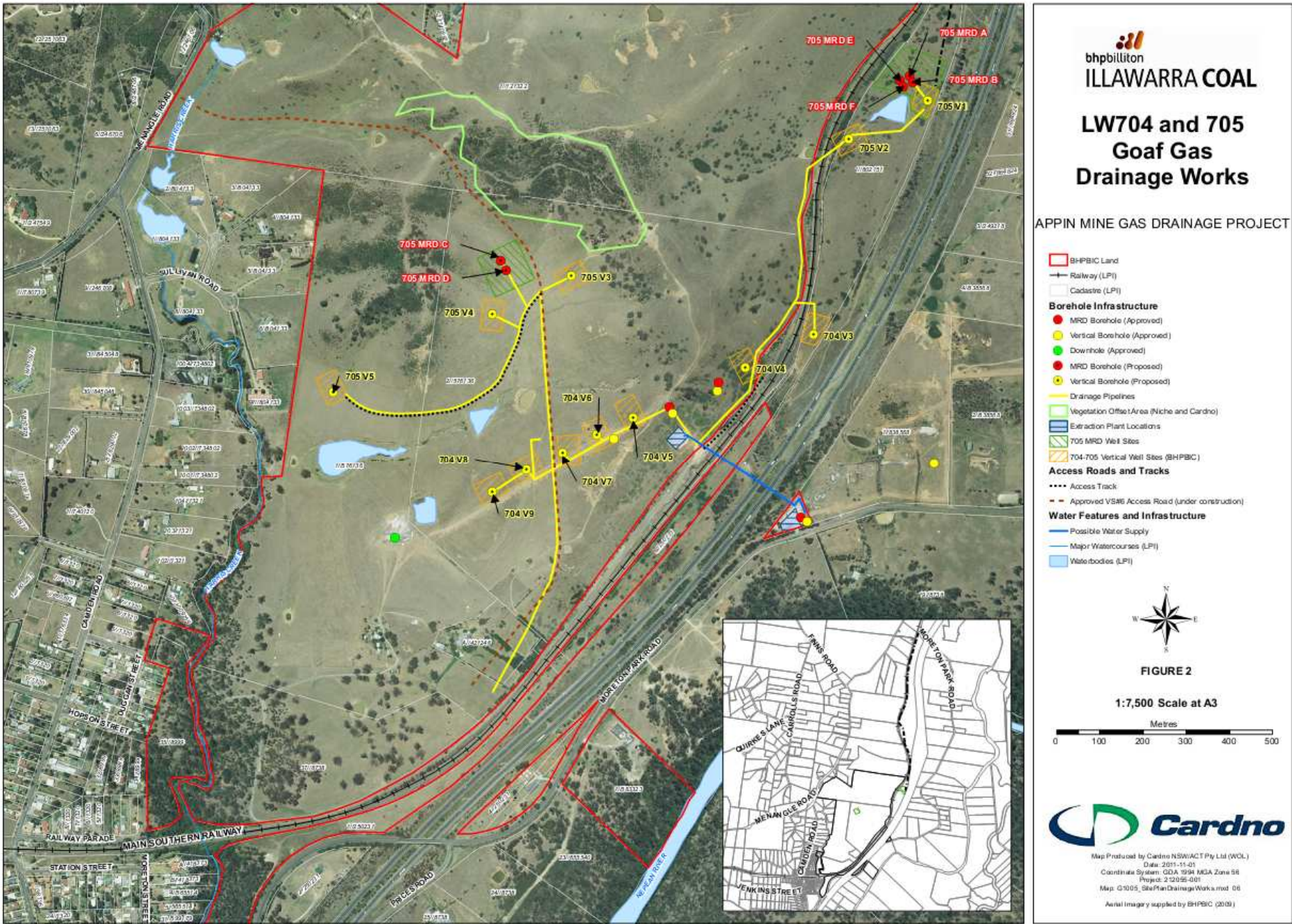
Figure 2-1 Aerial Image of the Goaf Drainage Site
