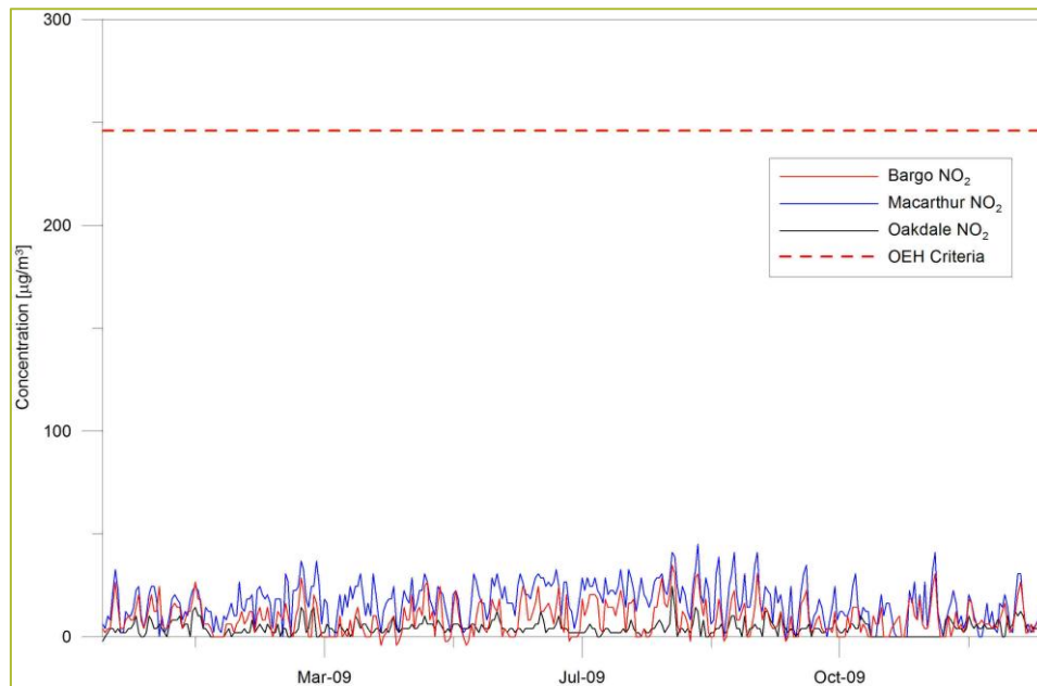
Figure 5.1: OEHL Monitoring NO 2 - 2009
