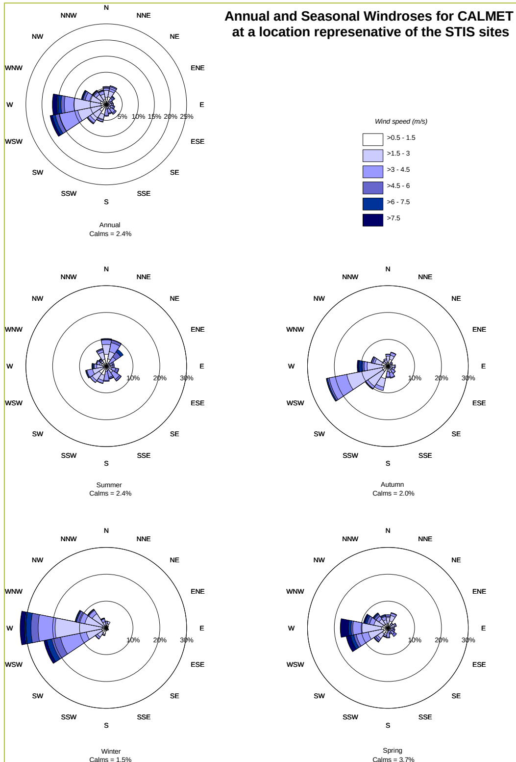
Figure 6.2: Wind Roses generated for MSGD Sites – Calmet 2009
