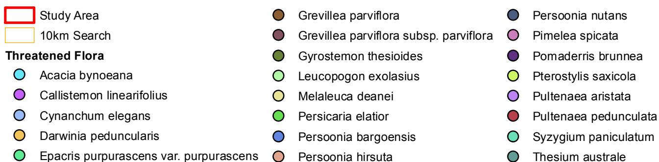
Figure 5: Threatened Flora previously found within 10km of the Study Area 1111 LW 704 - 705 Surface Gas Wells
