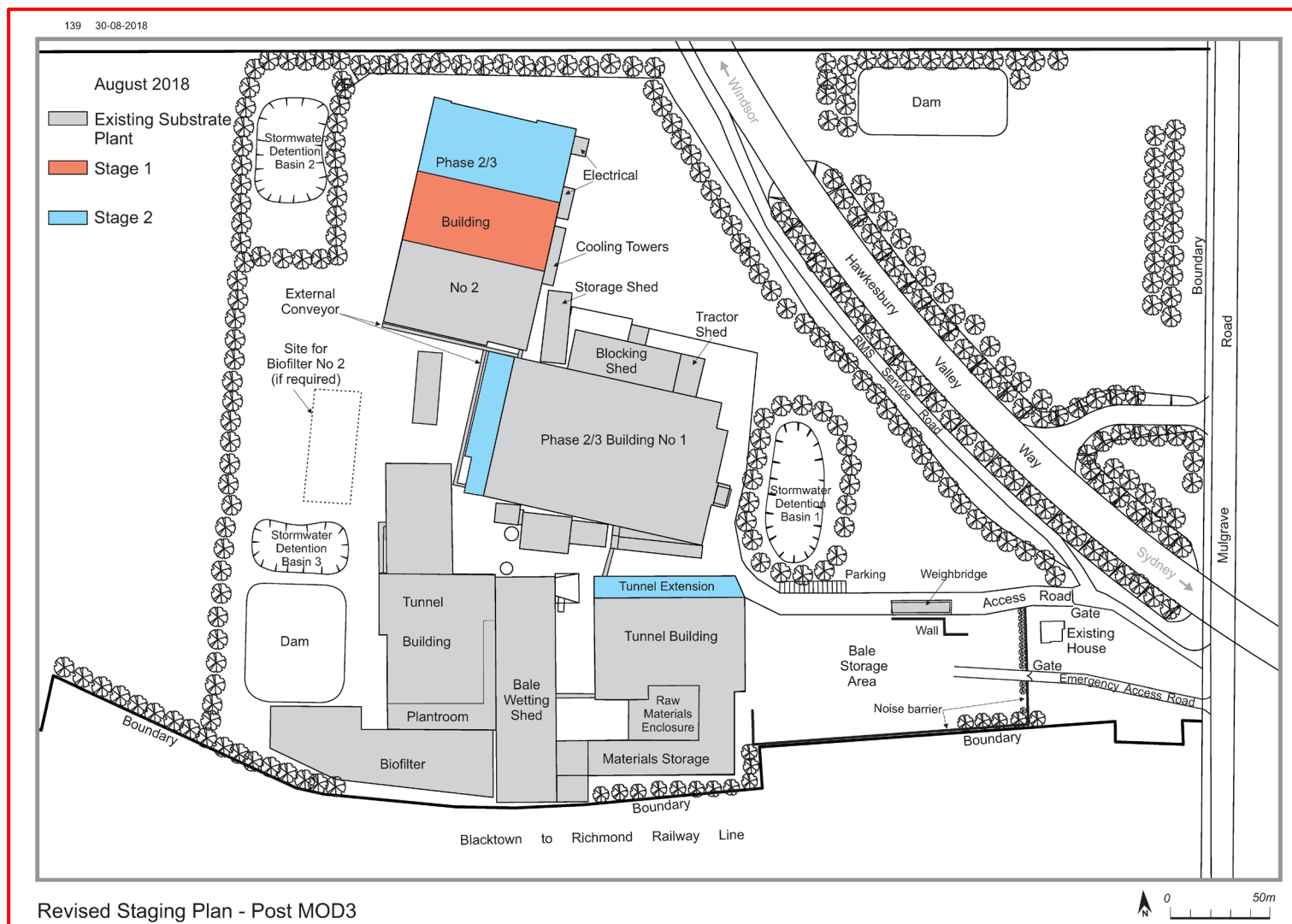
Figure 2: Substrate plant site staging following MOD 3
