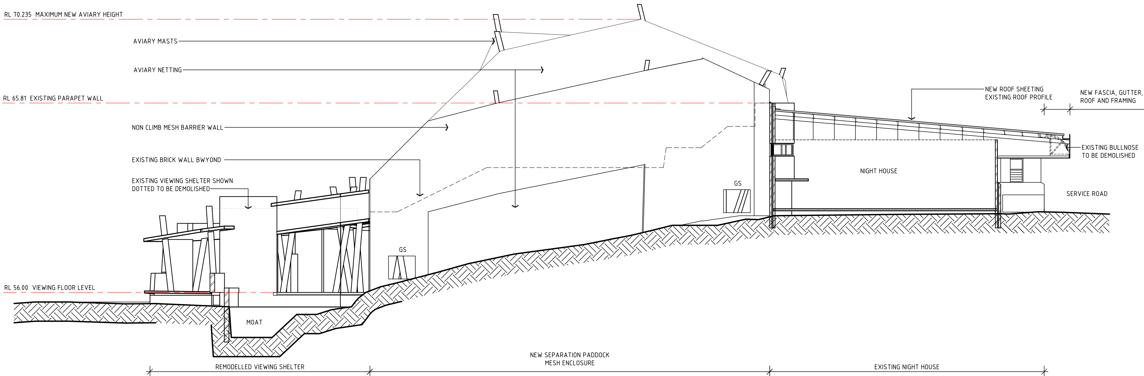
1 VIEWING SECTION AA - 1:100
