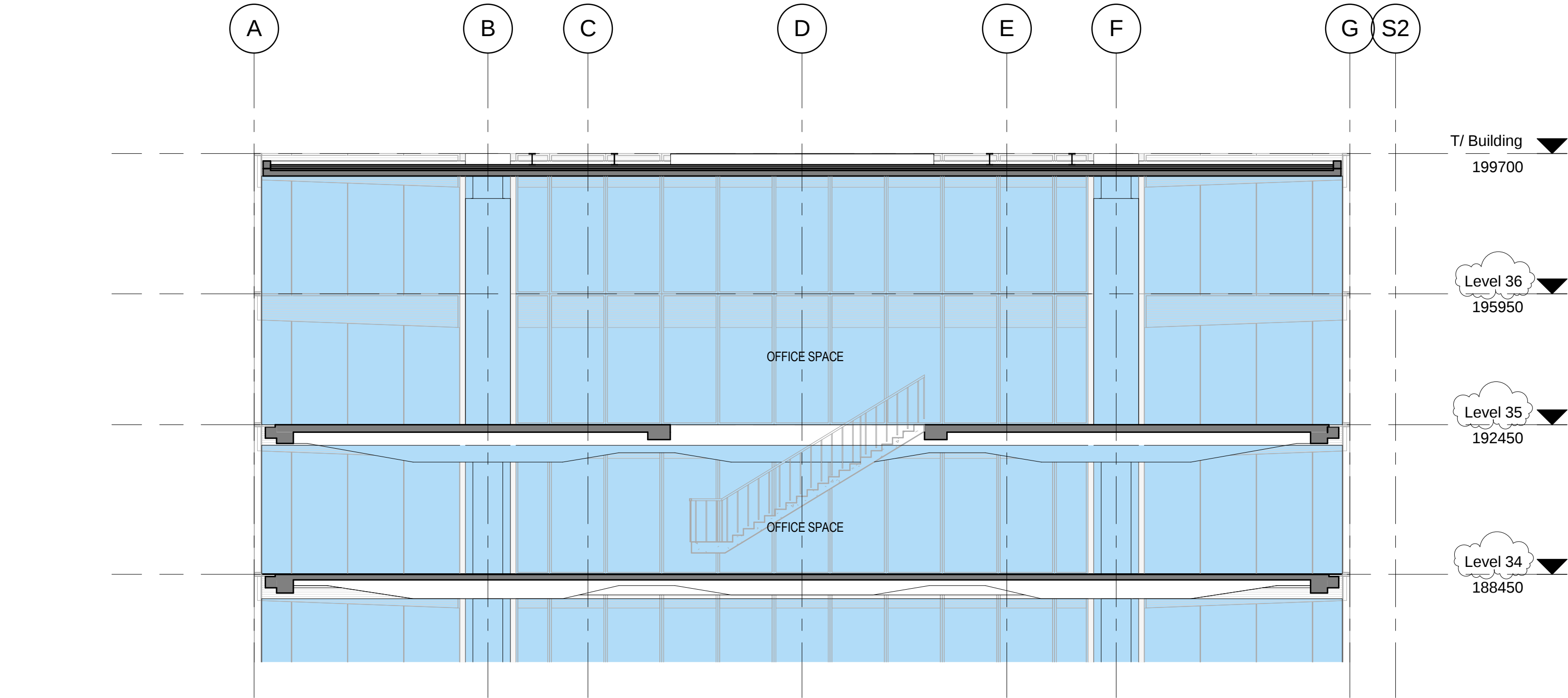
2 North-South Roof Section SCALE: 1 : 100
