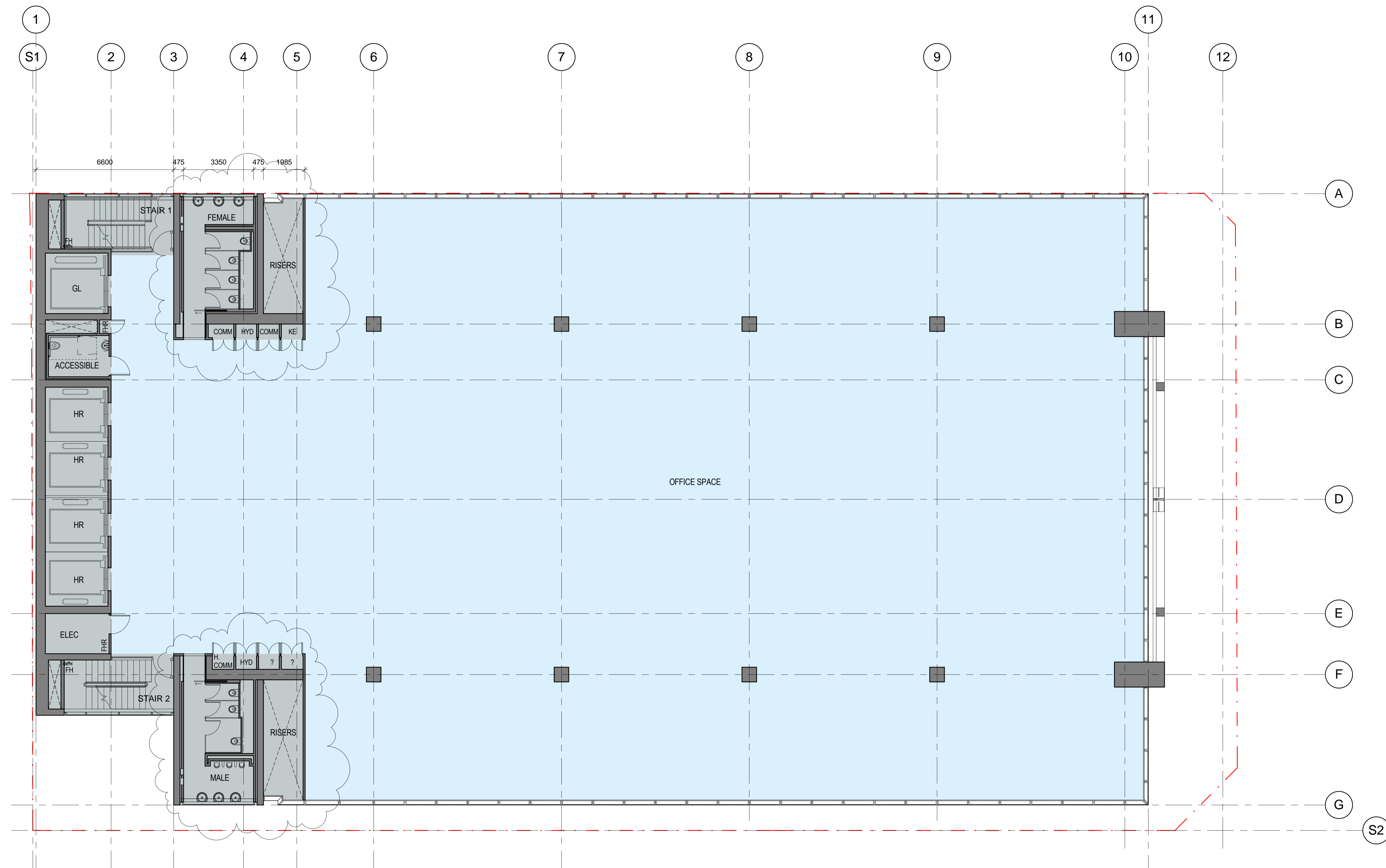
1 DA127_Typ. High Rise Level 1 : 100
