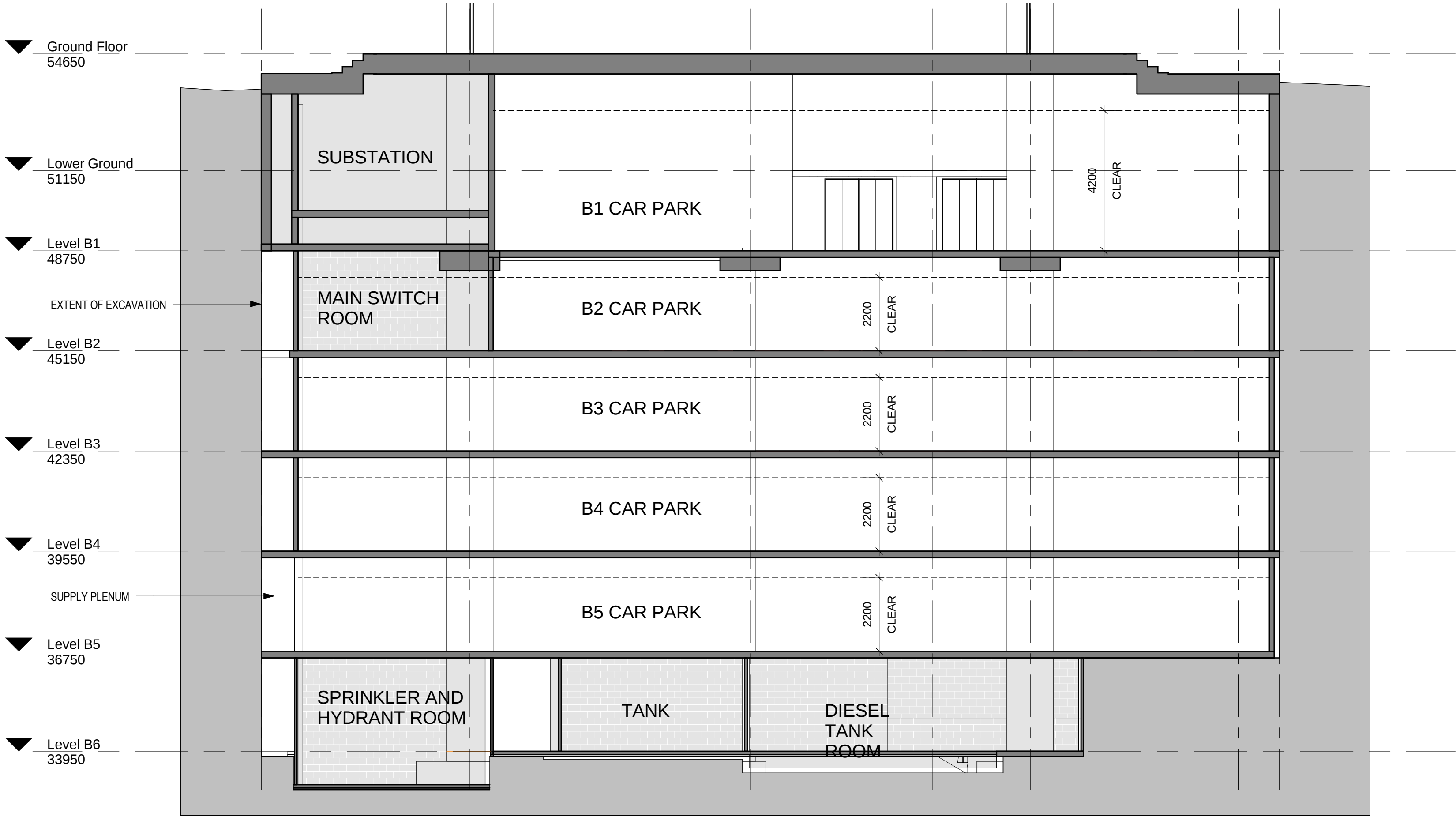
Basement Section - North South
