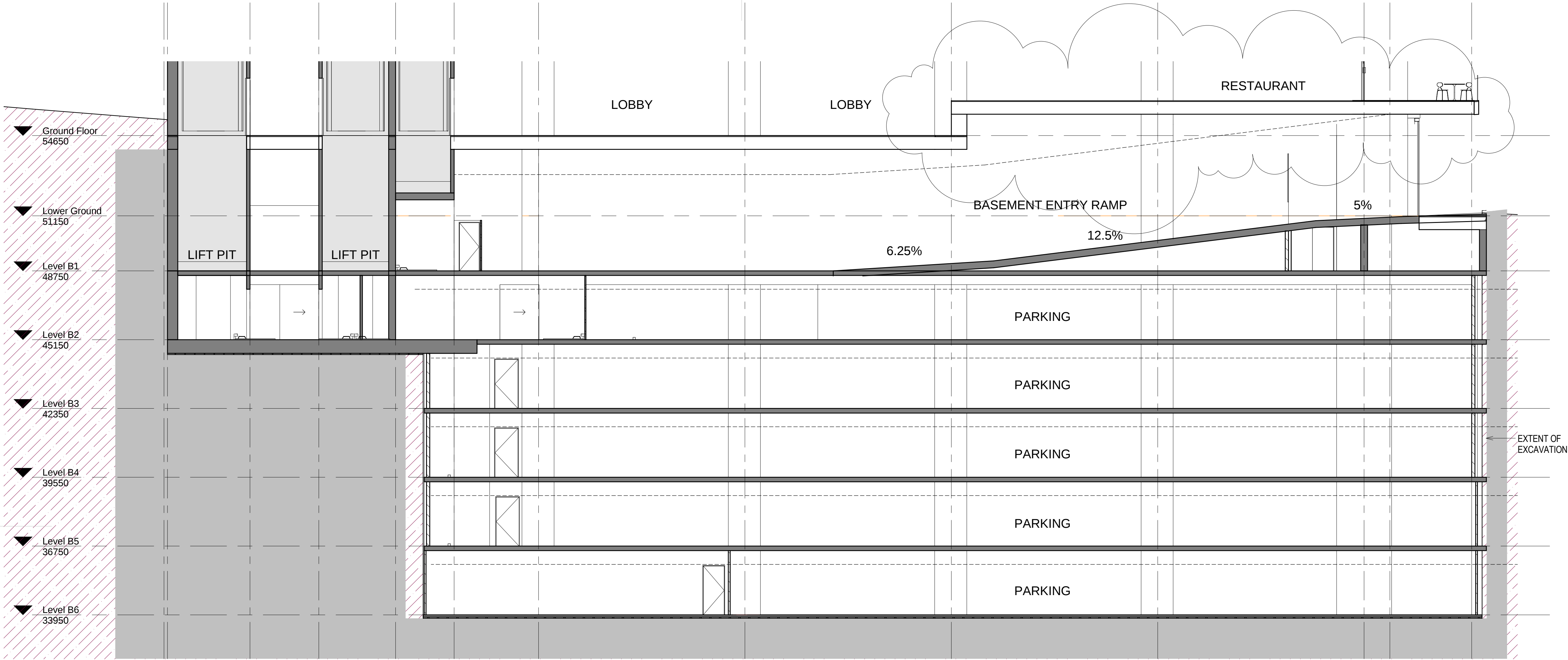
Basement Section - East West
