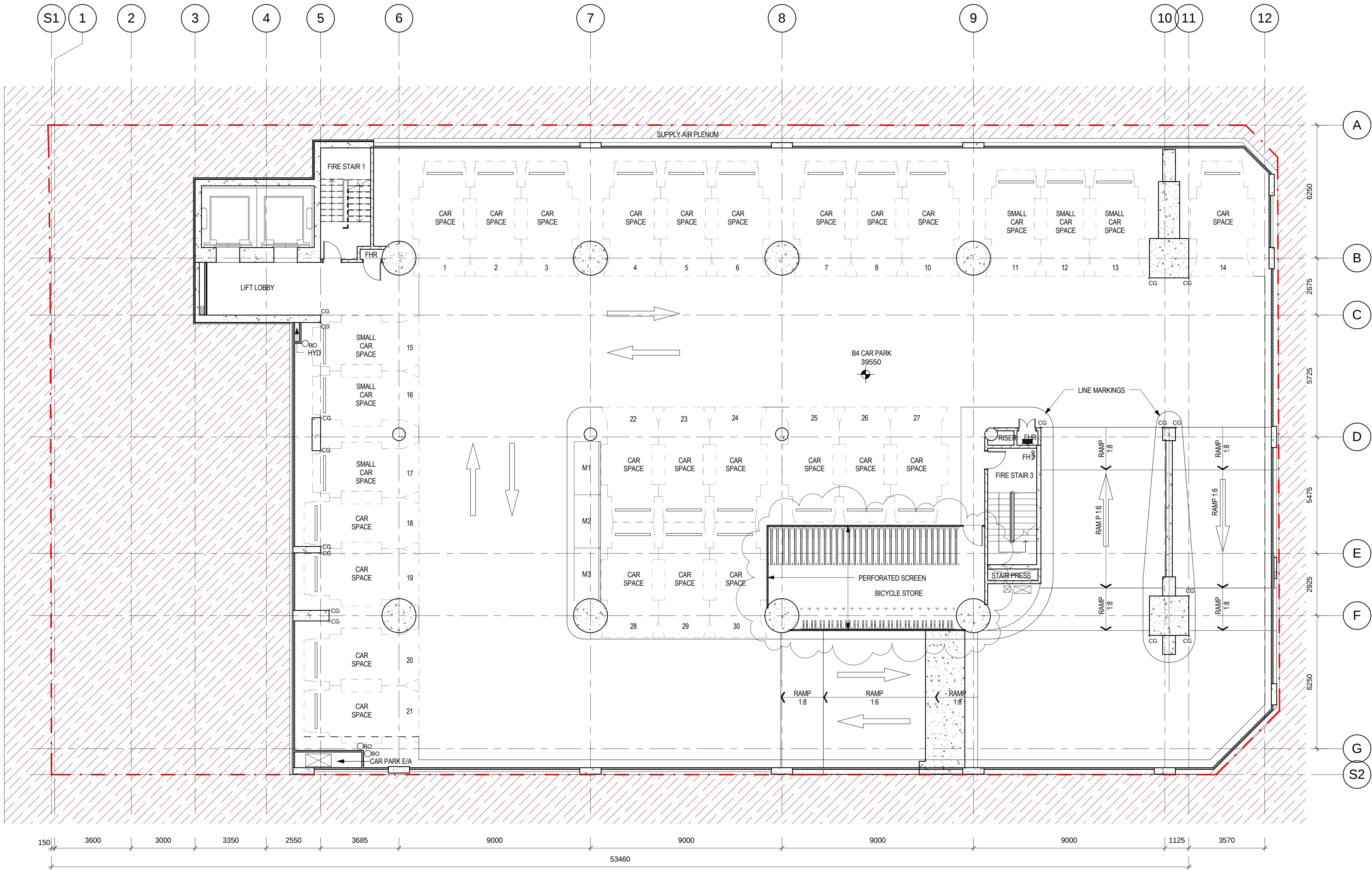
1 Level B4 Plan SCALE: 1 : 100
