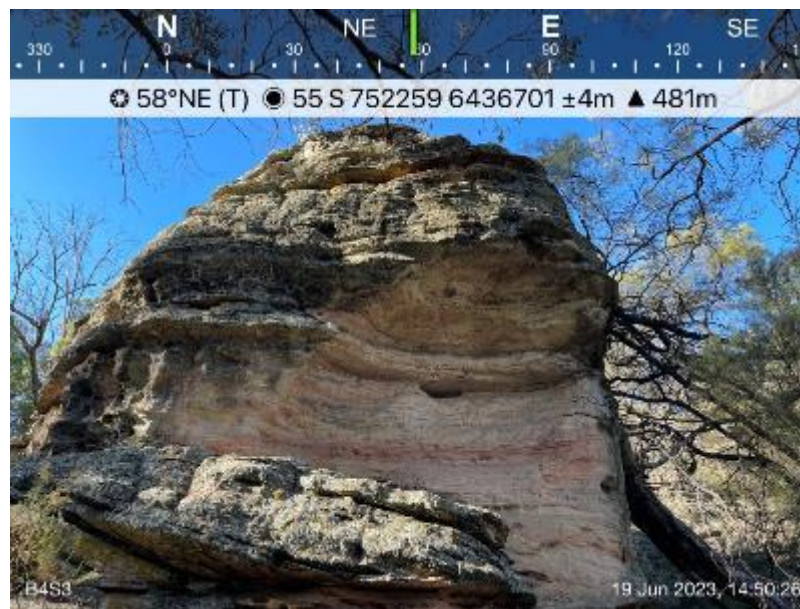
Cliff line Reference B4_S3: LW7 Post-Mining Inspection – 19 June 2023
