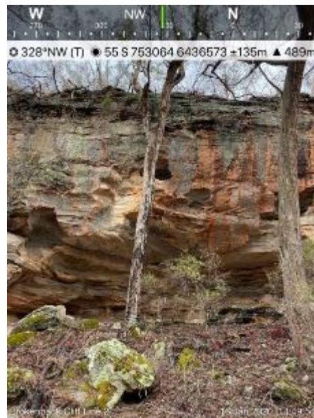
Cliff line Reference B2_S3: LW6 Post-Mining Inspection – 28 October 2021
