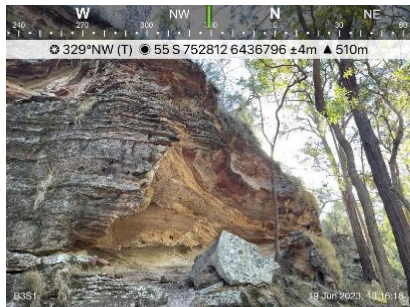
Cliff line Reference B3-S1 & Heritage Site Ulan ID#917: LW7 Post-Mining Inspection – 19 June 2023
