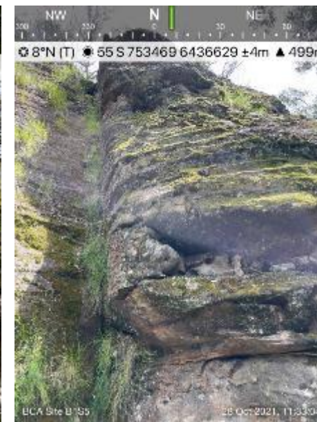
Cliff line Reference B1_S5: LW5 Post-Mining Inspection – 28 October 2021
