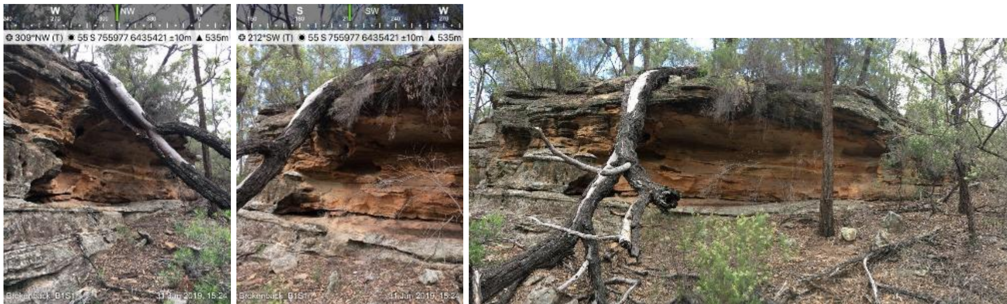
Cliff line Reference: B1_S1: LW5 Post-Mining Inspection – 16 January 2020
