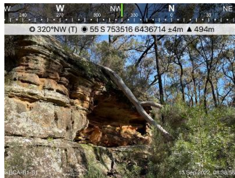
Cliff line Reference: B1_S1: LW6 Post-Mining Inspection – 13 September 2022
