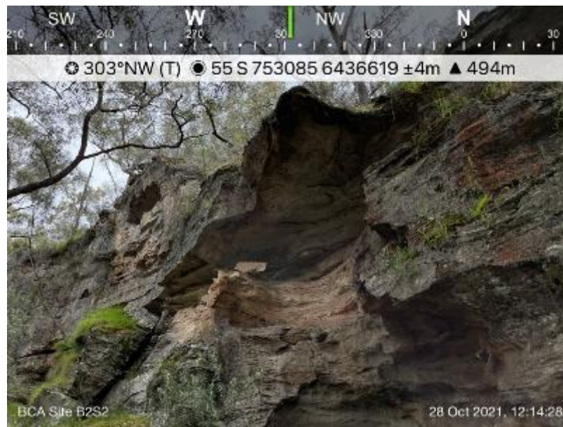
Cliff line Reference B2_S2: LW6 Post-Mining Inspection – 28 October 2021
