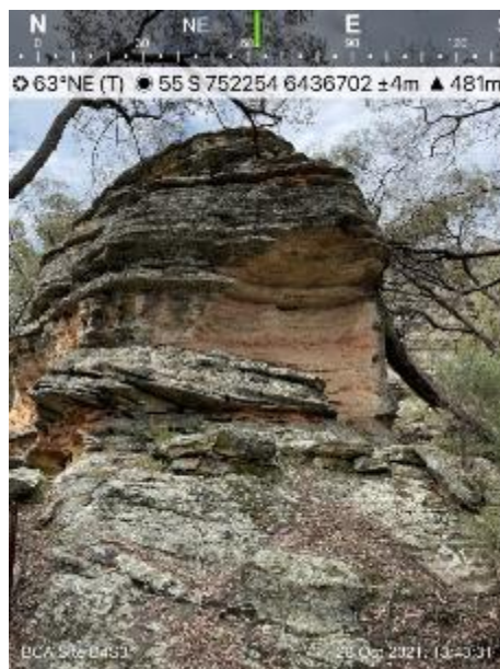
Cliff line Reference B4_S3: LW5 Post-Mining Inspection – 28 October 2021
