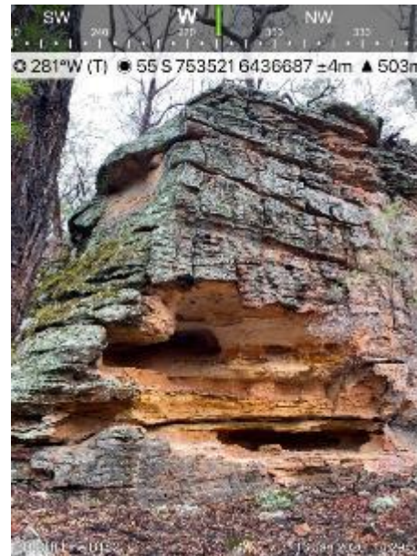
Cliff line Reference: B1_S2: LW6 Post-Mining Inspection – 28 October 2021
