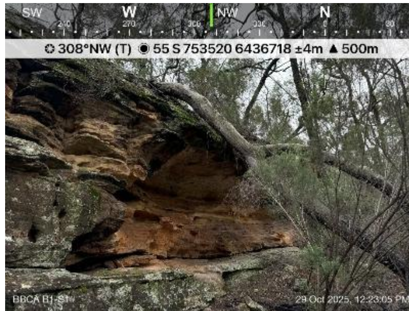
Cliff line Reference: B1_S1: LW8B Post Mining Inspection – 29 October 2025
