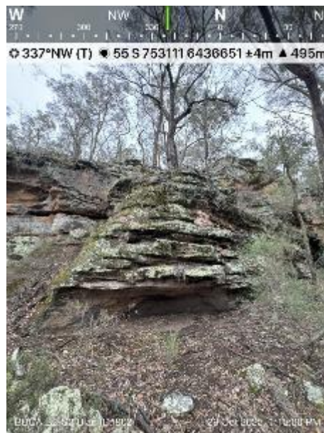
Cliff line Reference B2_S2 & Heritage Site Ulan ID#902: LW8B Post Mining Inspection – 29 October 2025
