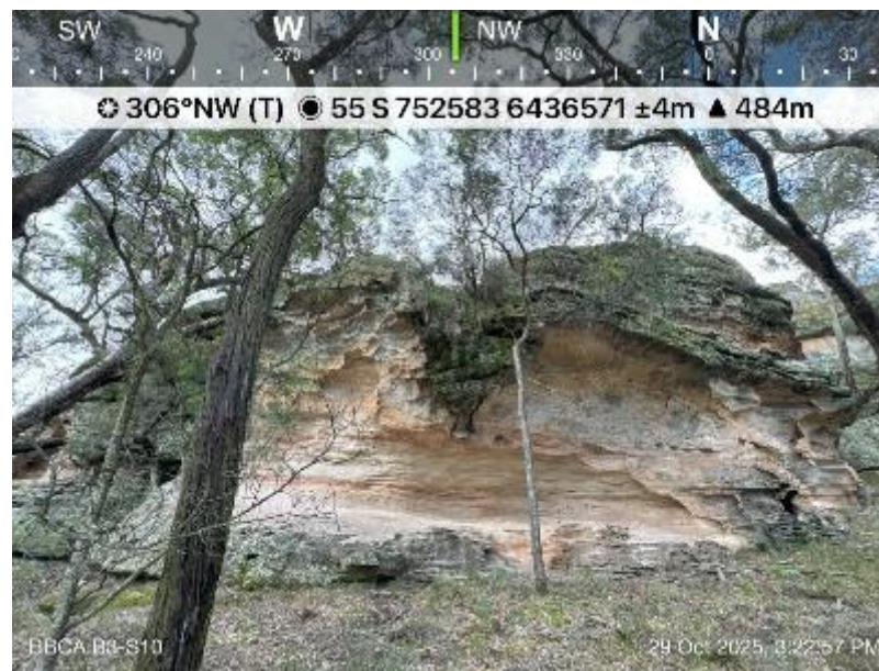
Cliff line Reference B3_S10: LW8B Post Mining Inspection – 29 October 2025
