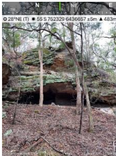
Cliff line Reference B4_S2: LW5 Post-Mining Inspection – 28 October 2021
