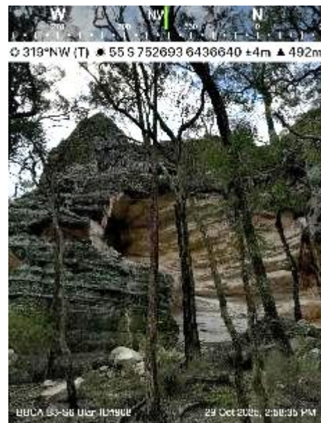
Cliff line Reference B3_S6: LW8B Post Mining Inspection – 29 October 2025
