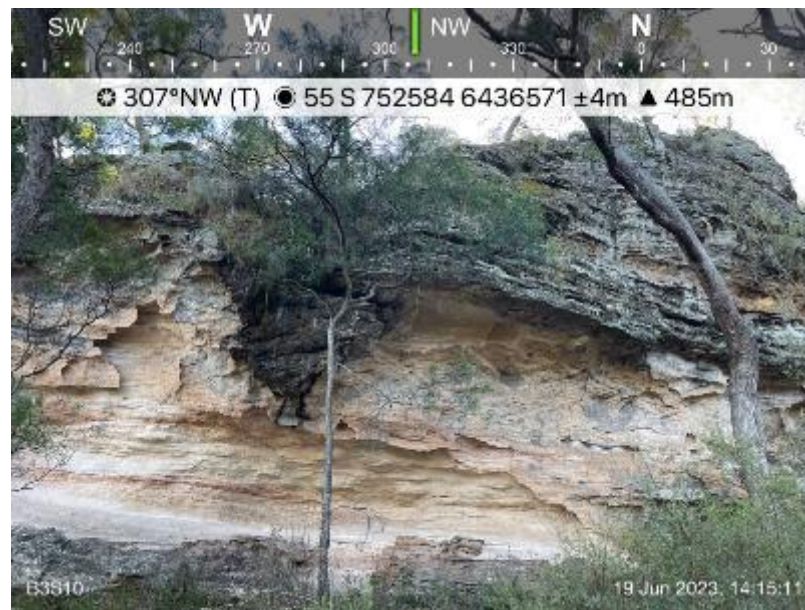
Cliff line Reference B3_S10: LW7 Post-Mining Inspection – 19 June 2023
