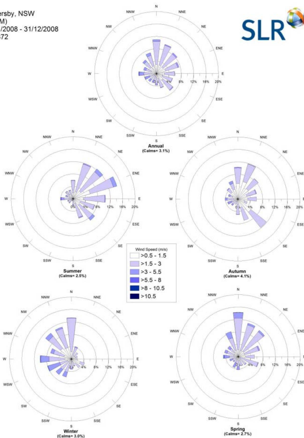
Figure 3: TAPM Predicted Annual and Seasonal Wind Roses, CCSQ 2008
