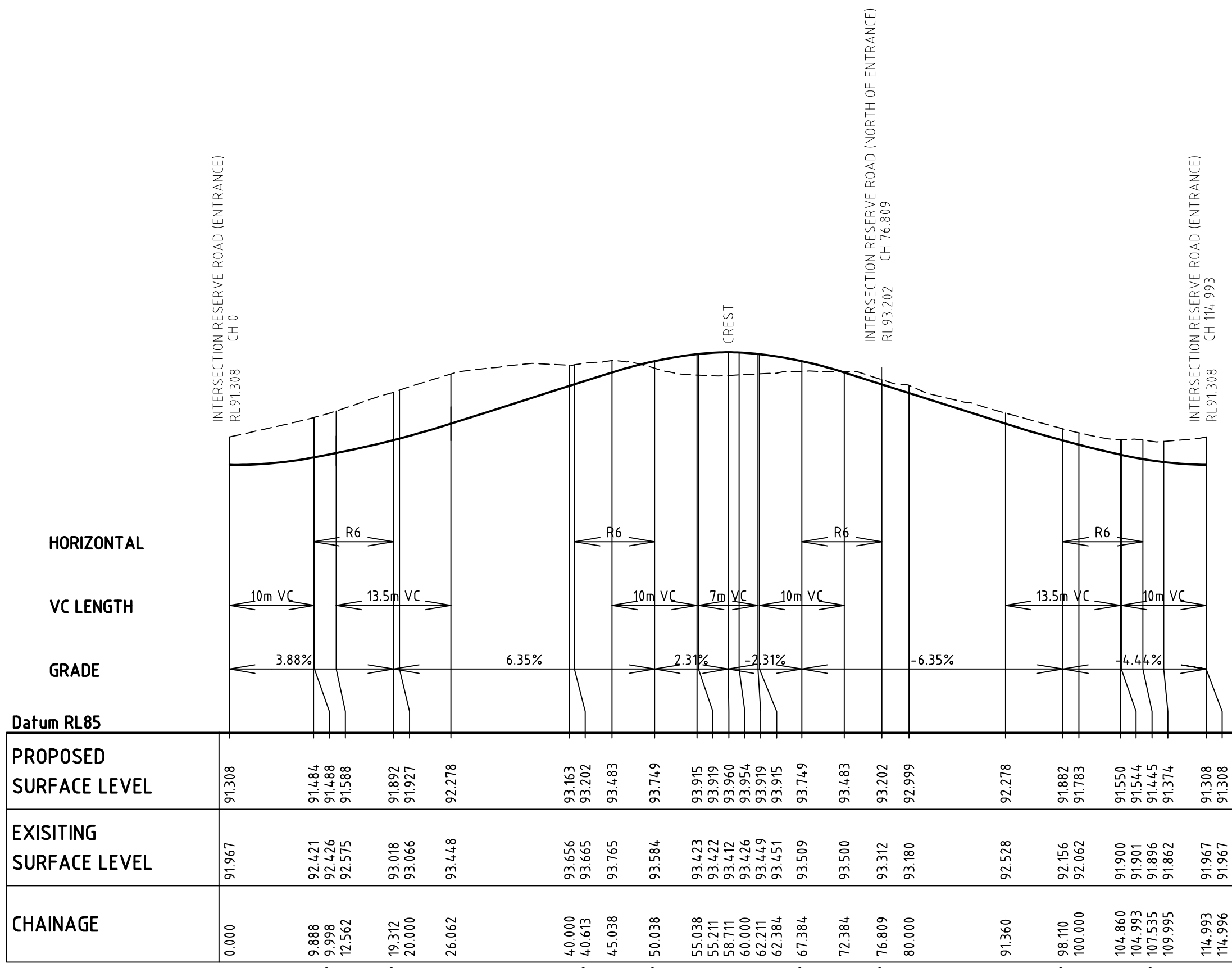
RESERVE ROAD (ENTRANCE LOOP) LONGITUDINAL SECTION
