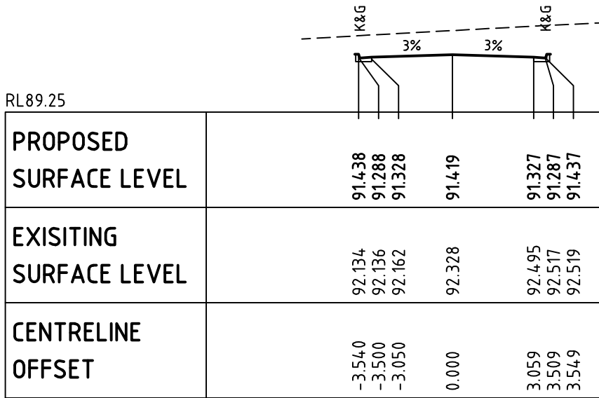
CH 8 1:200 (TYPICAL)
