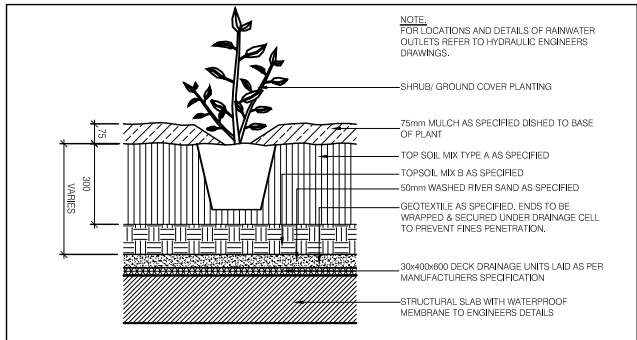
4 MASS PLANTING ON STRUCTURAL SLAB SECTION 1:10
