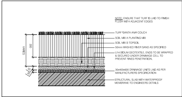
2 TURF ON STRUCTURAL SLAB SECTION 1:10
