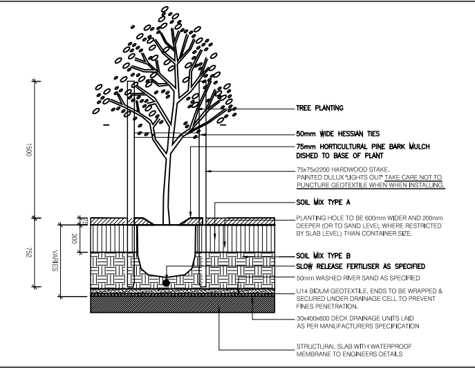
7 TREE PLANTING ON STRUCTURE SECTION 1:20
