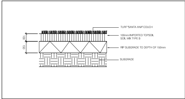
1 TURF ON NATURAL GROUND SECTION 1:10
