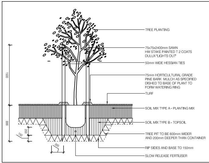
5 TREE PLANTING IN TURF SECTION 1:20
