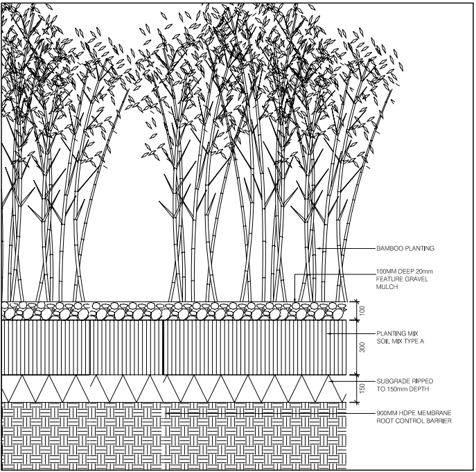
9 RHIZOME ROOT CONTROL BARRIER SECTION 1:10
