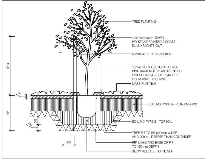
6 TREE IN MASS PLANTING SECTION 1:20
