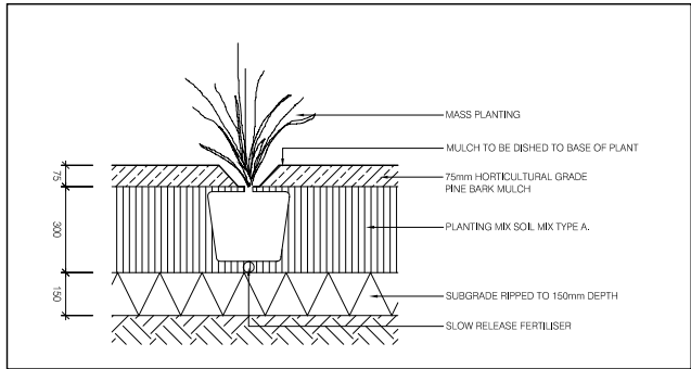
3 MASS PLANTING ON NATURAL GROUND SECTION 1:10
