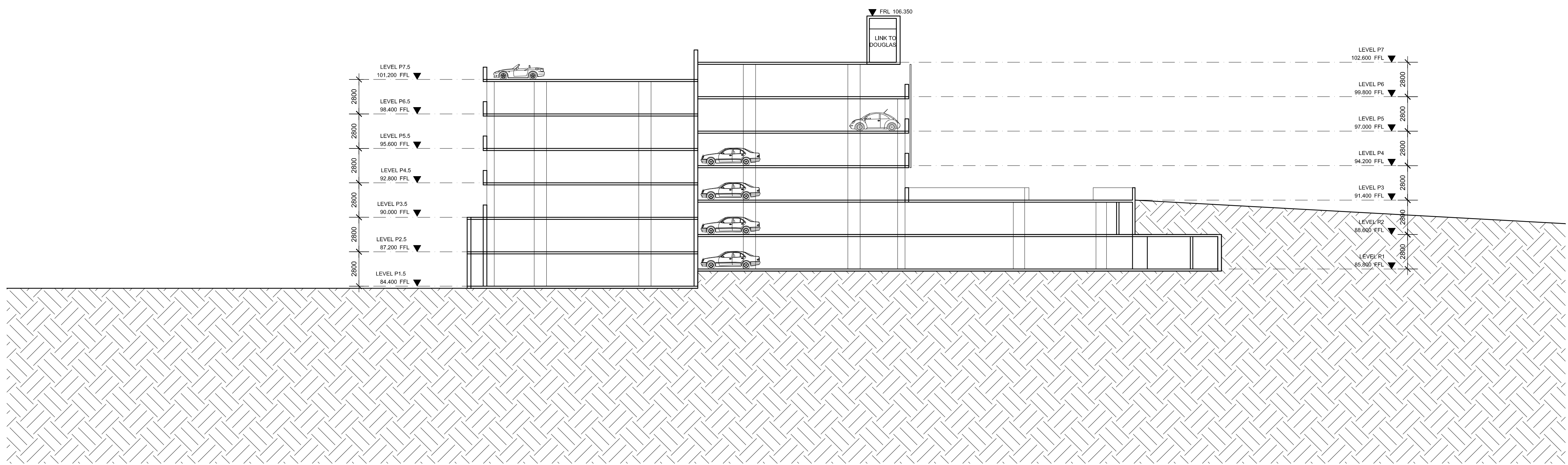
CROSS SECTION
