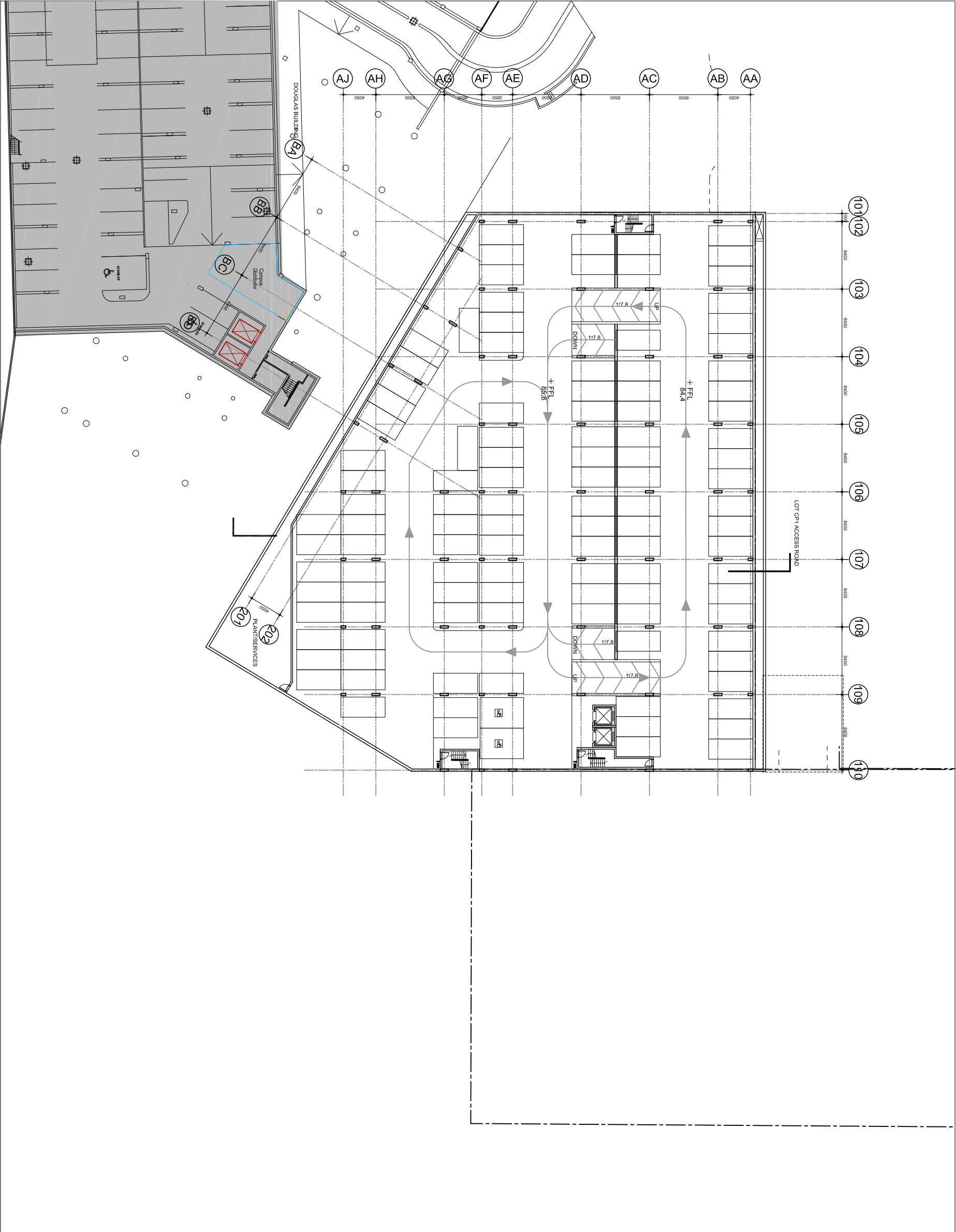
WESTERN CARPARK - LEVEL P1 (FFL 85.8)
