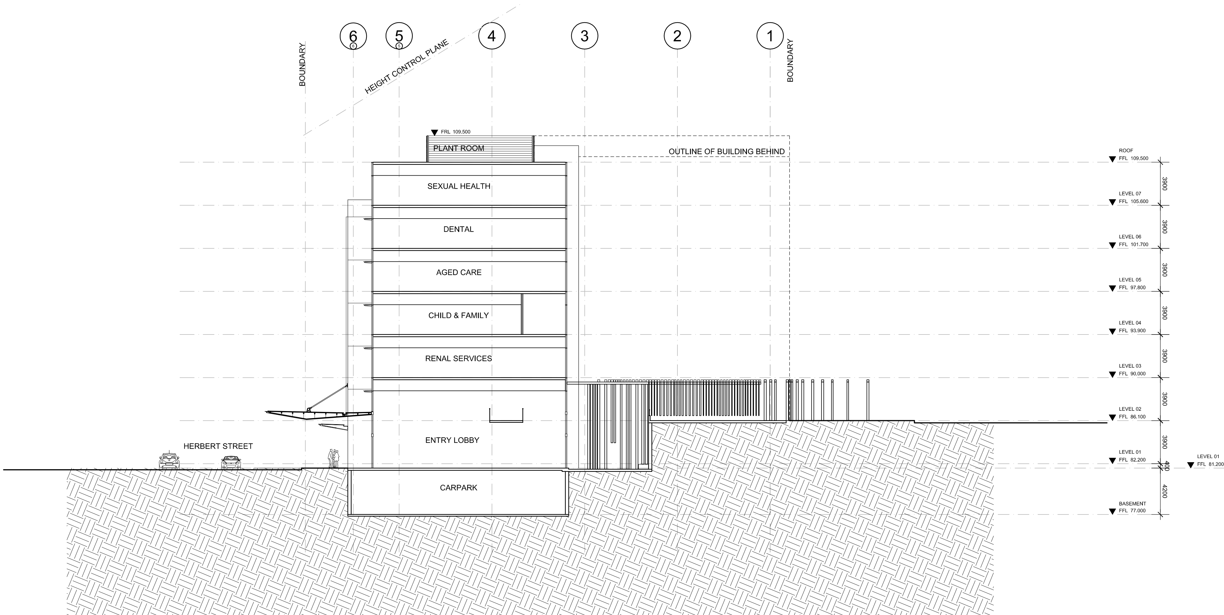
EAST WEST SECTION
