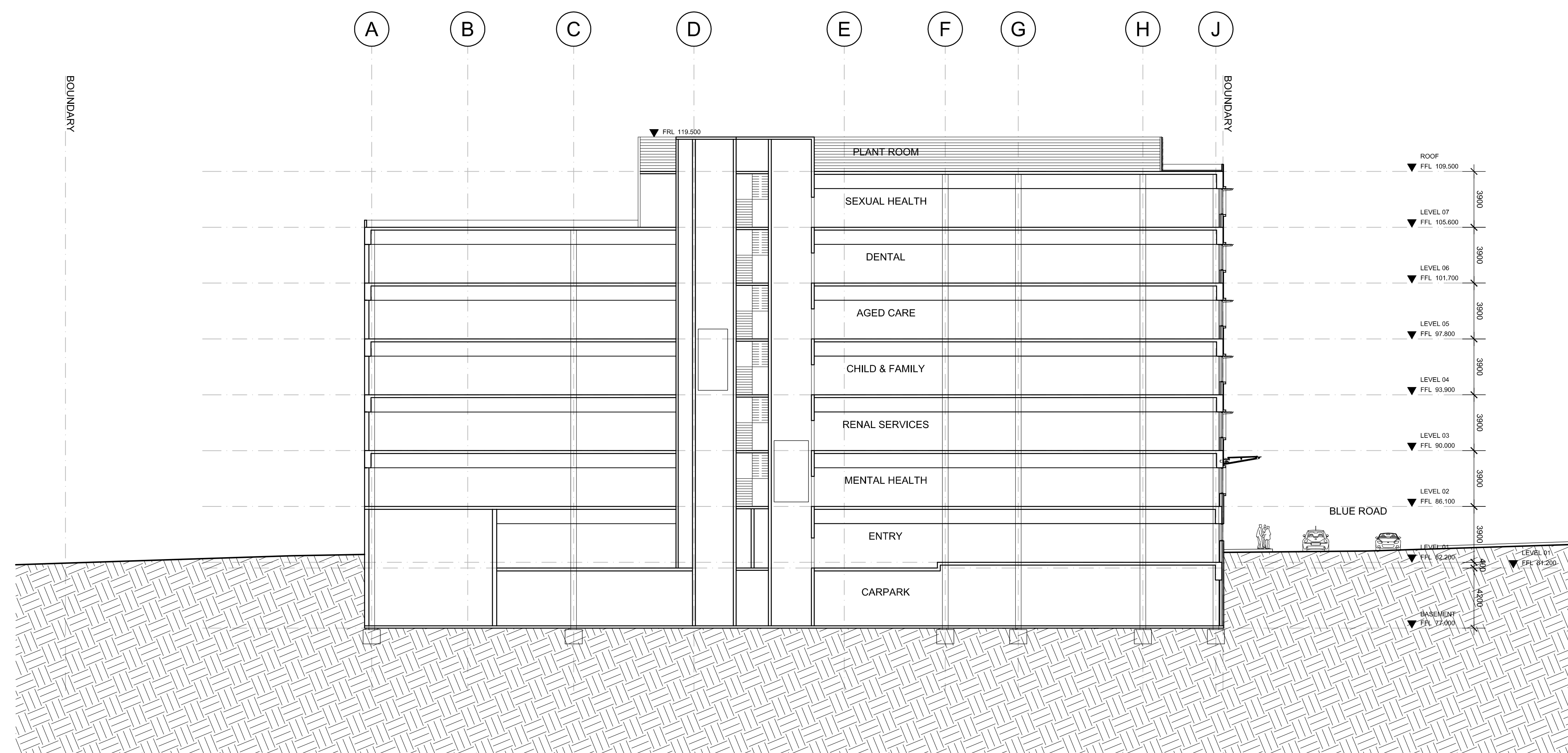
NORTH SOUTH SECTION
