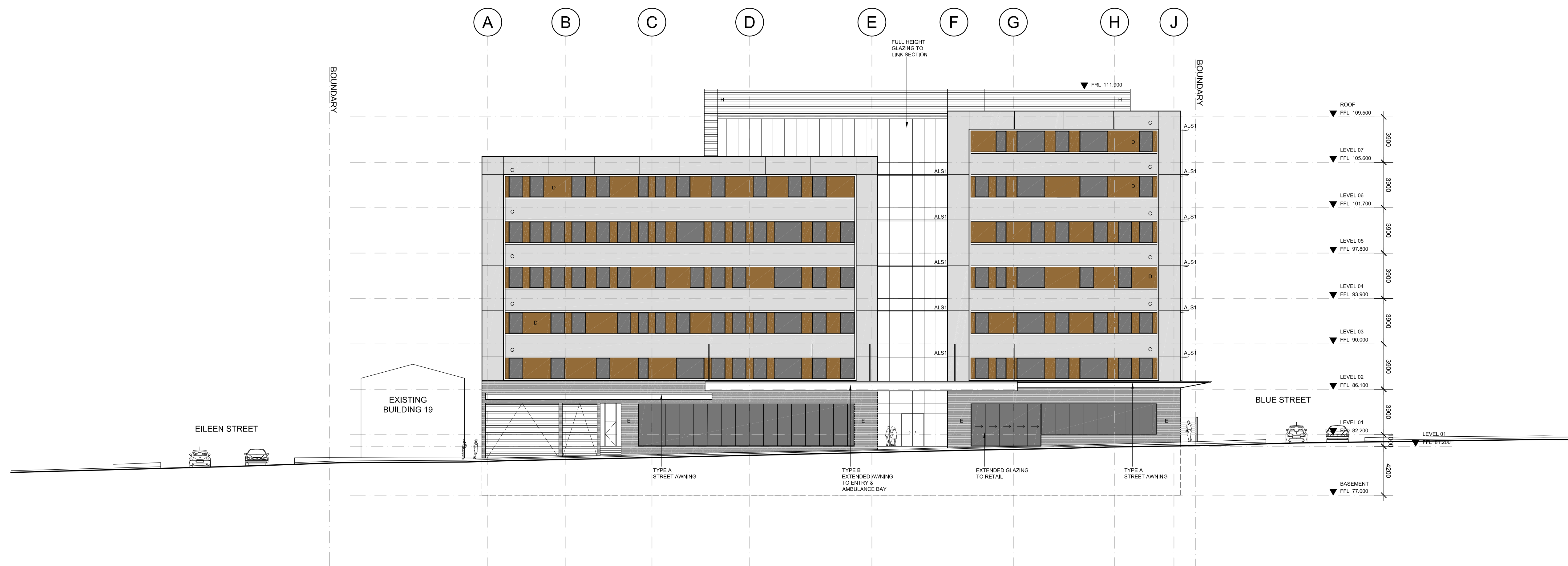
EAST ELEVATION (HERBERT STREET) 1:200
