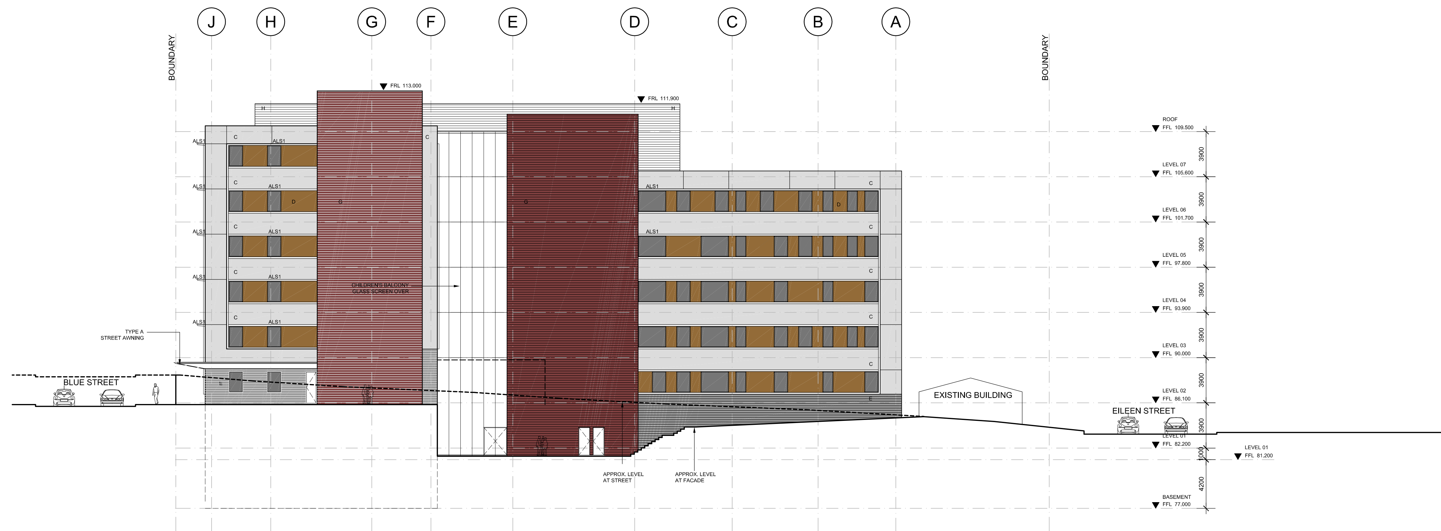
WEST ELEVATION (RED ROAD) 1:200
