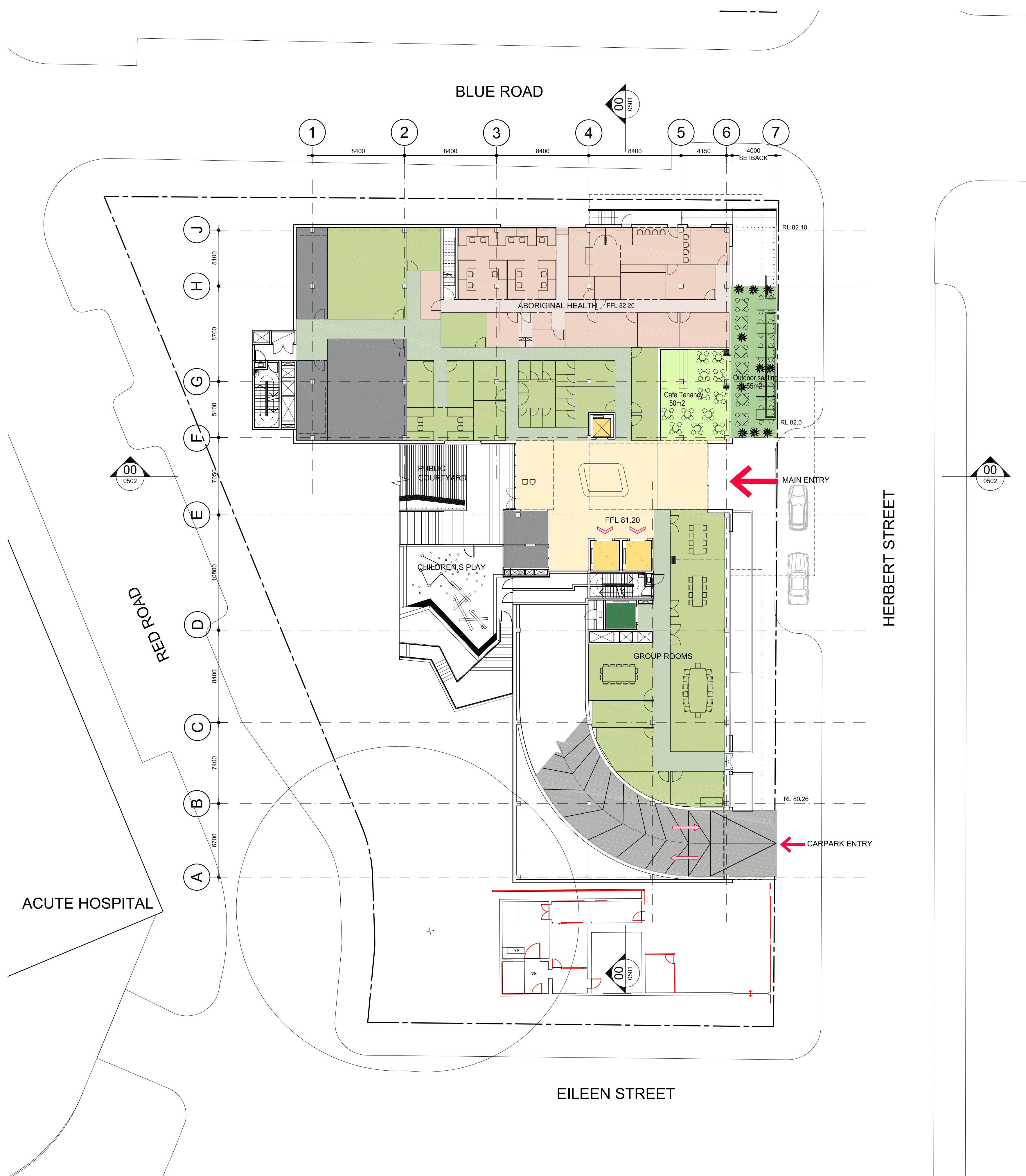
LEVEL 1 GROUND FLOOR PLAN 1:200 FFL 81.20
