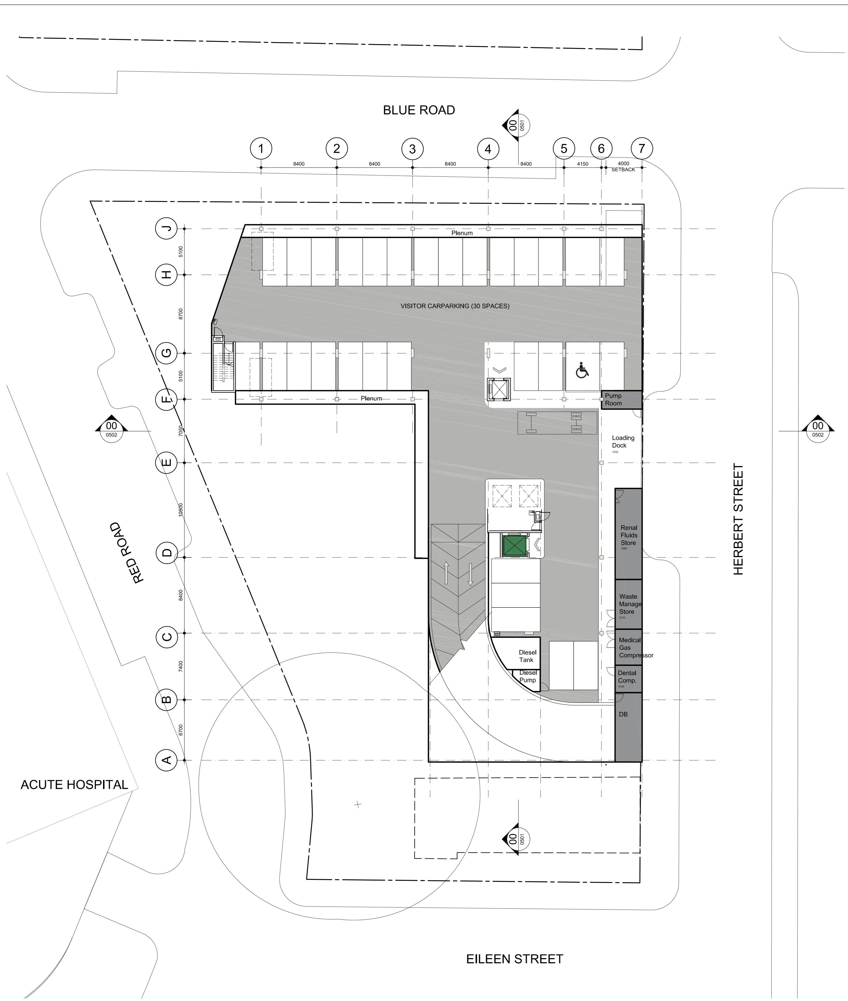
BASEMENT FLOOR PLAN 1:200 FFL 75.20
