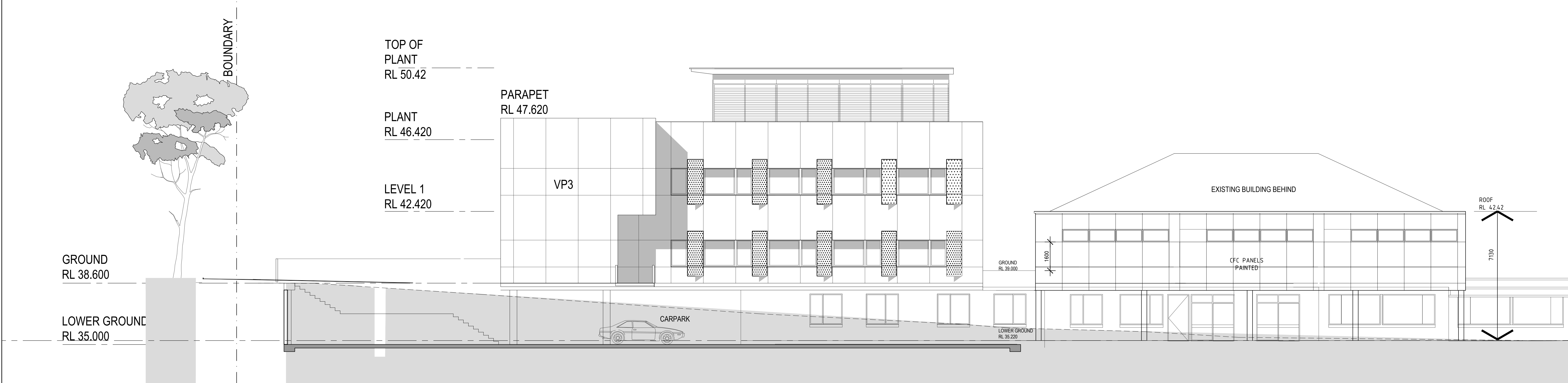
ELEVATION - EAST
