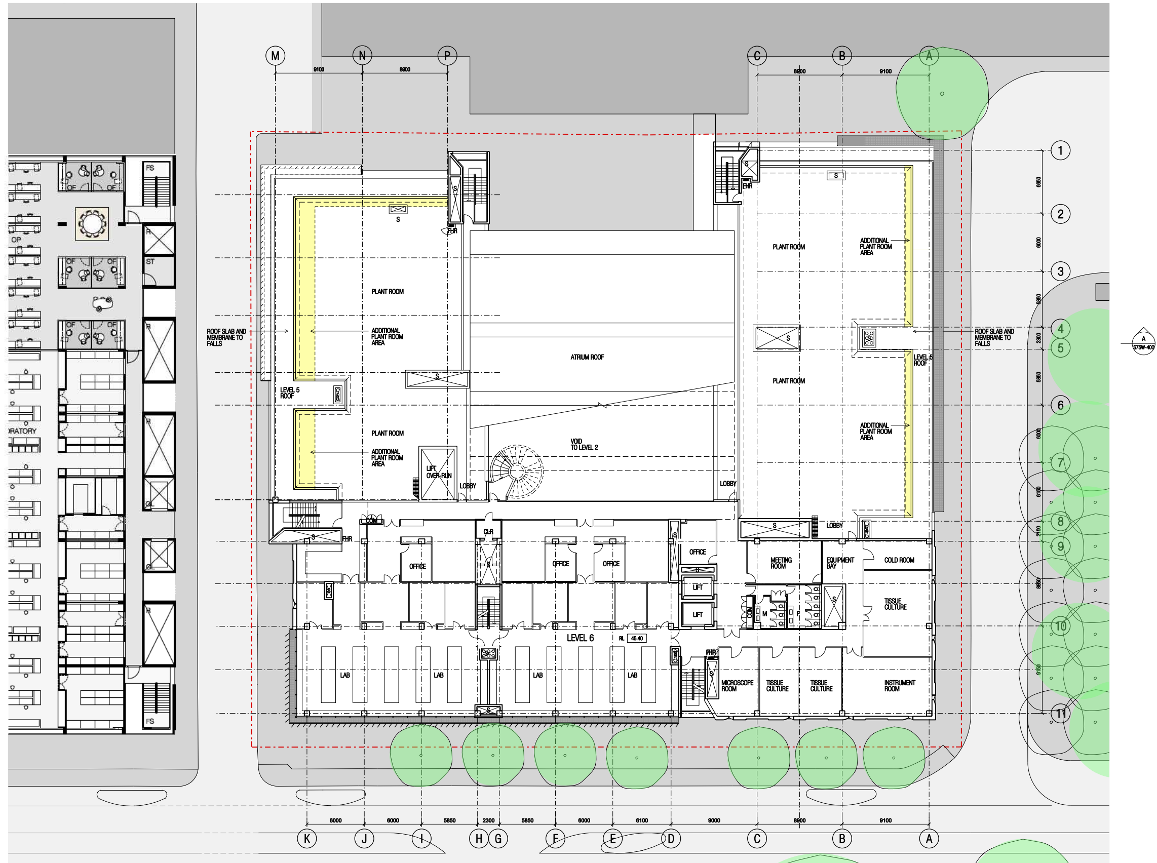
1 LEVEL 6 (RL 45.40) SCALE 1:200
