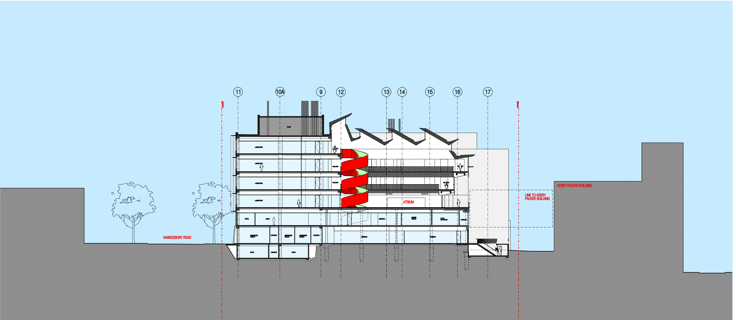
1 SECTION BB SCALE 1:200
