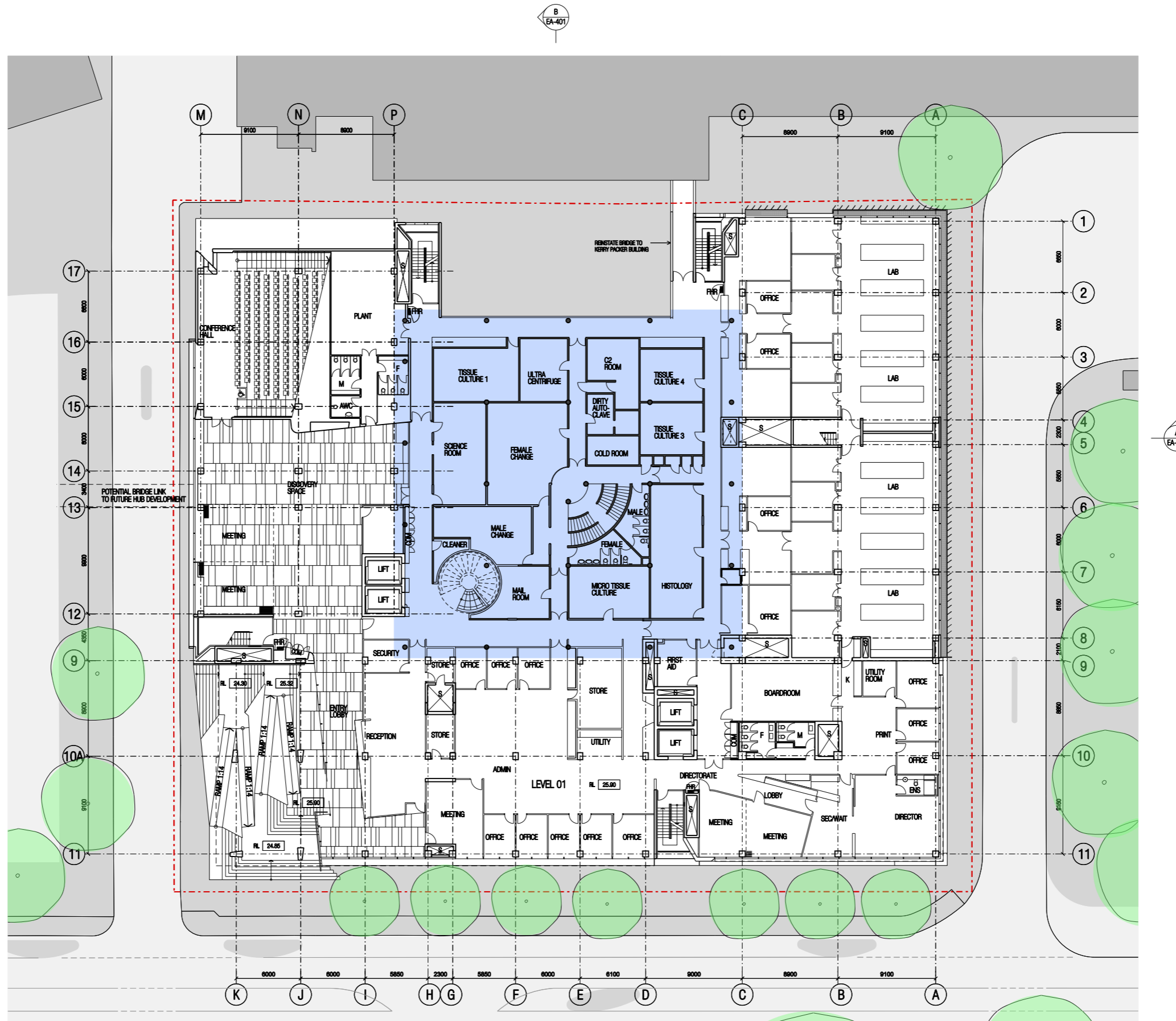
1 LEVEL 1 (RL 25.90) SCALE 1:200
