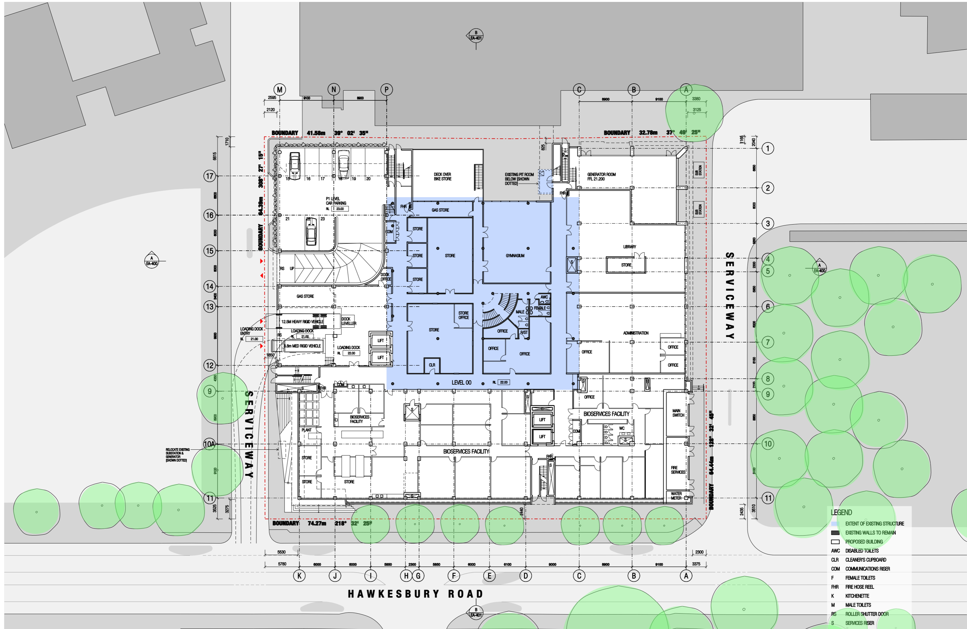
1 LEVEL 0 - SITE PLAN (RL 22.00) SCALE 1:200
