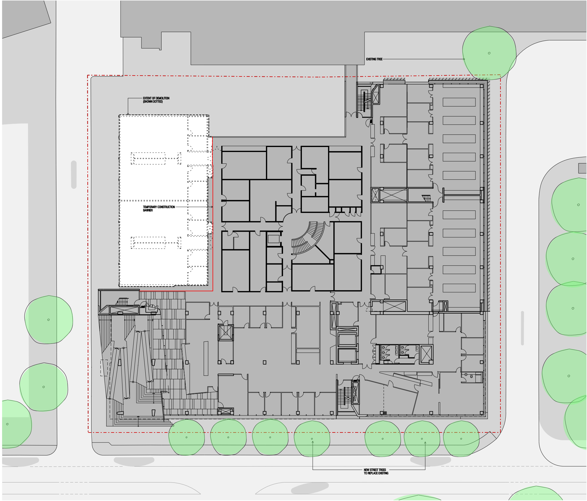
1 STAGE 4 DEMOLITION PLAN - FIRST FLOOR SCALE 1:200
