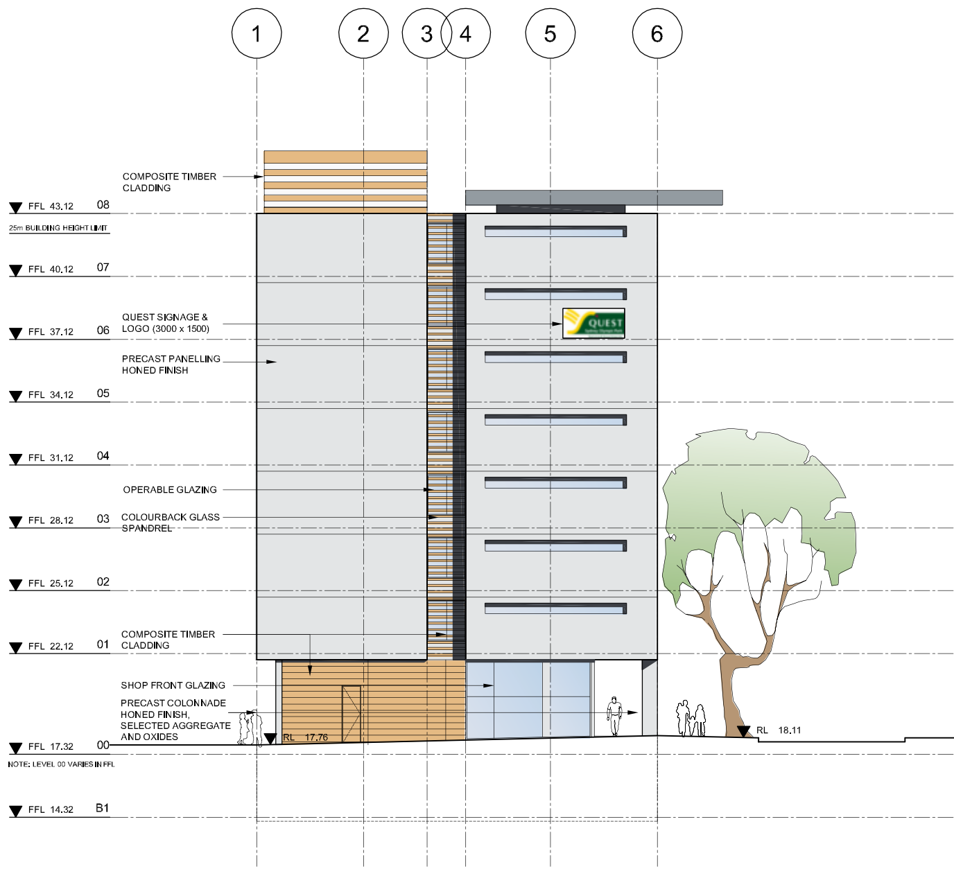
01 SOUTH ELEVATION 1:250
