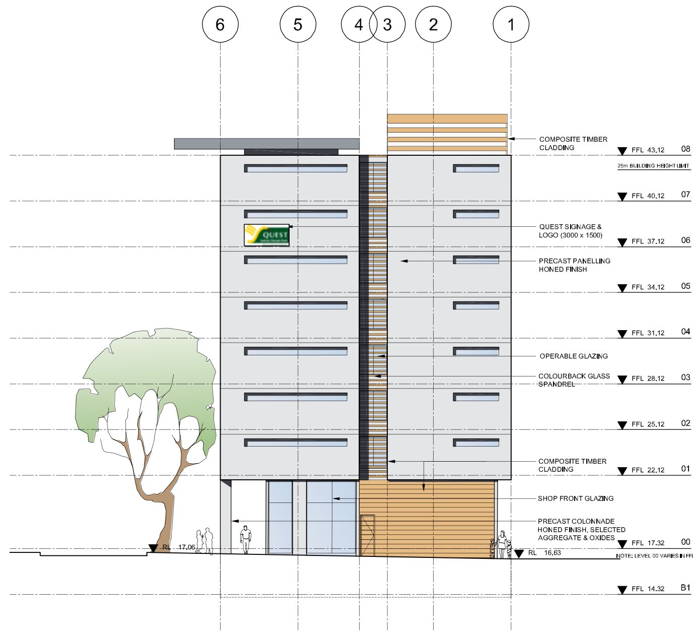
02 NORTH ELEVATION 1:250
