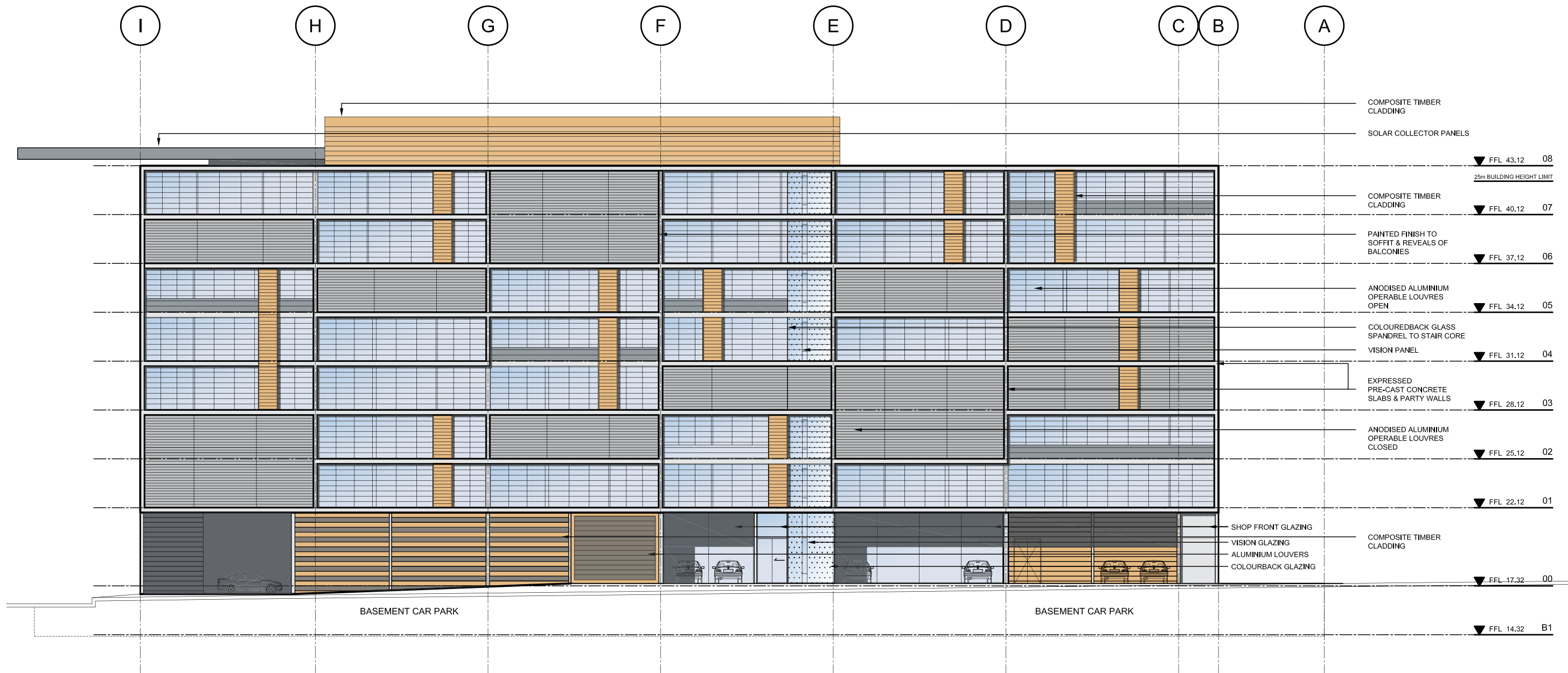
01 WEST ELEVATION 1:250
