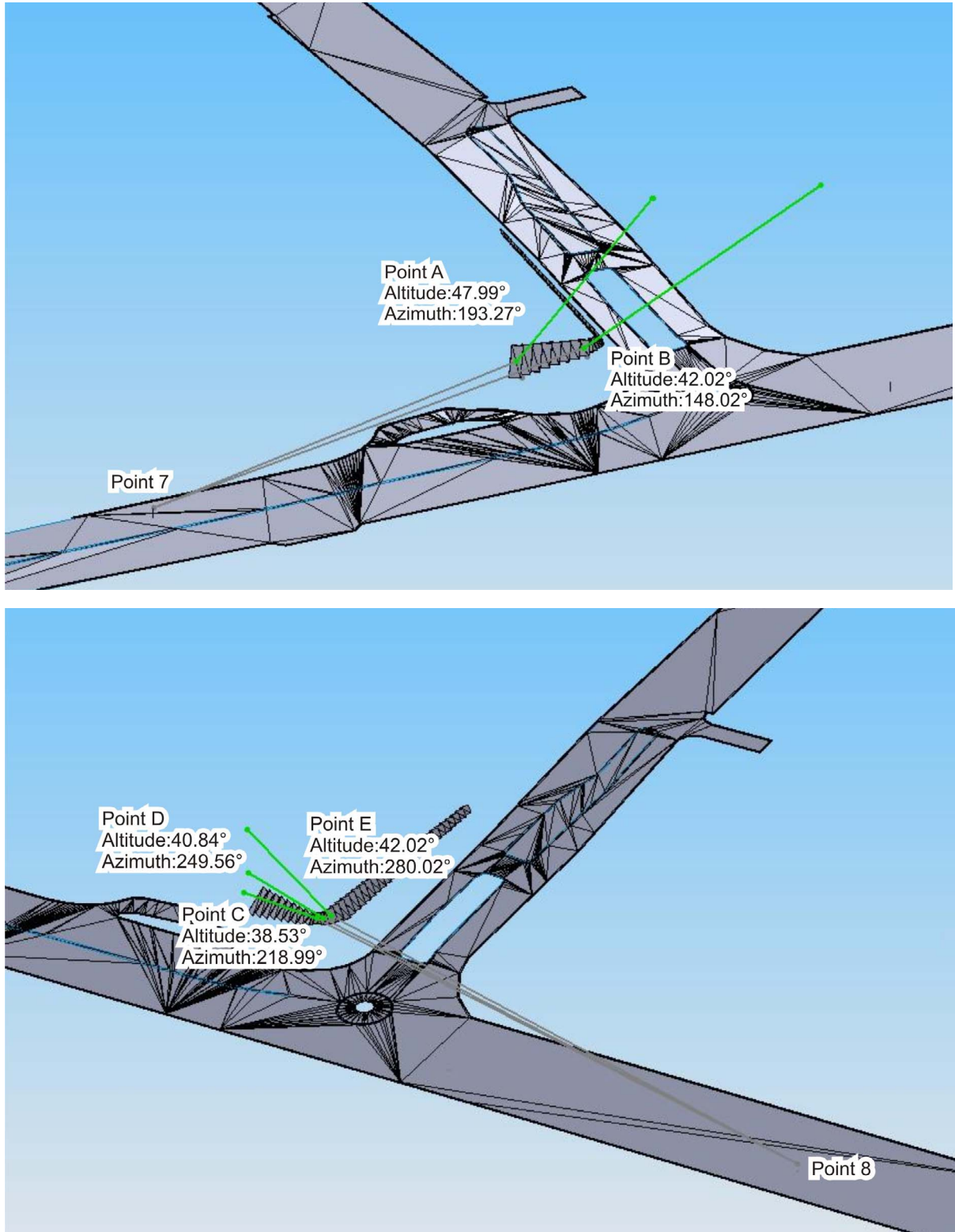
Figure 4: Solar Reflections to Study Points 7 and 8 from the Inclined Aspects
