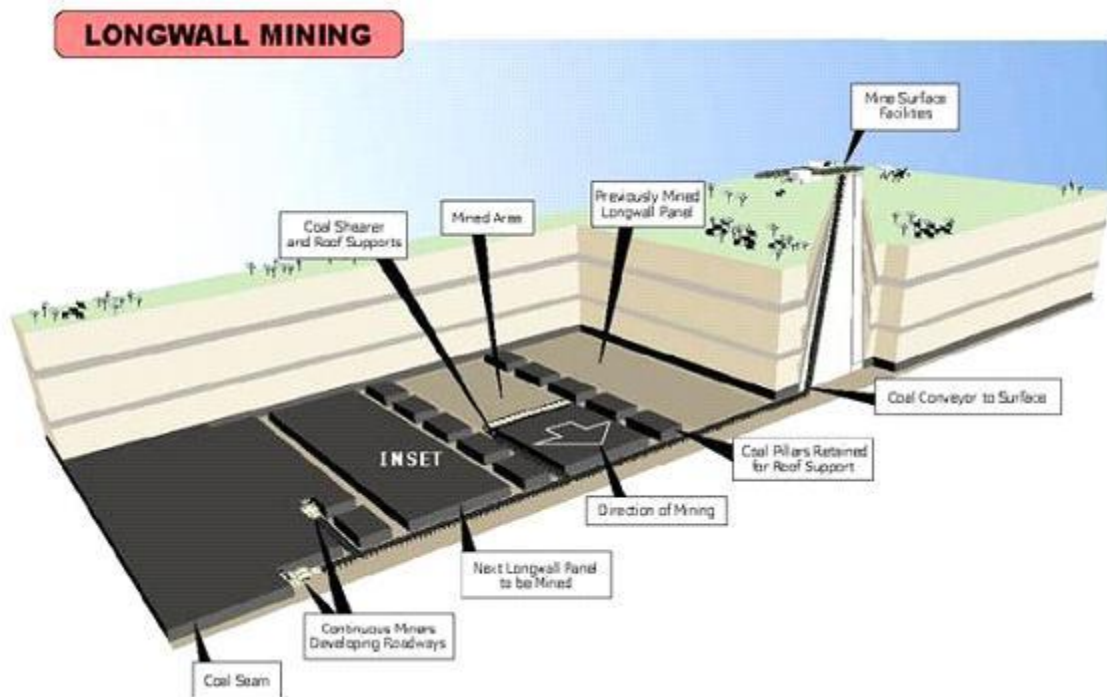
Fig 2.1 Illustration of Longwall Mining
