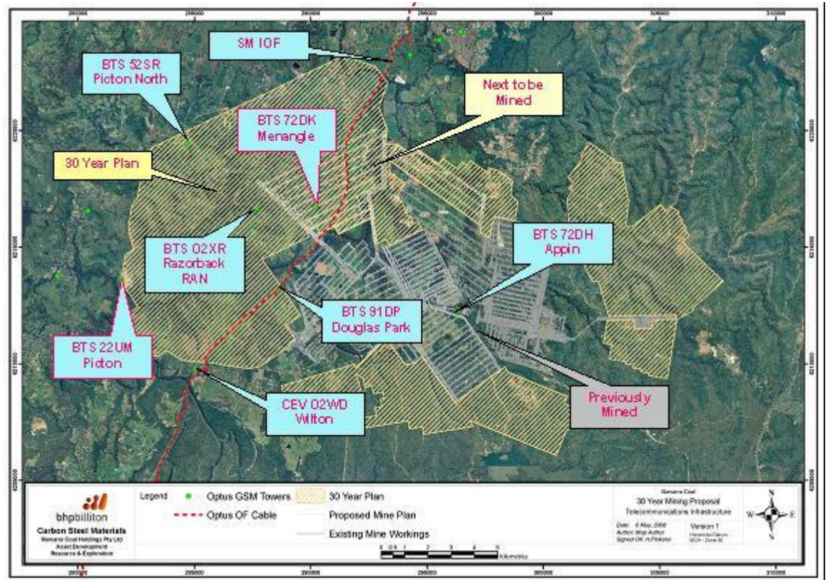
Fig 3.1.1 Impacted area showing Sydney Melbourne 1 IOF, Mobile phone sites, and CEV
