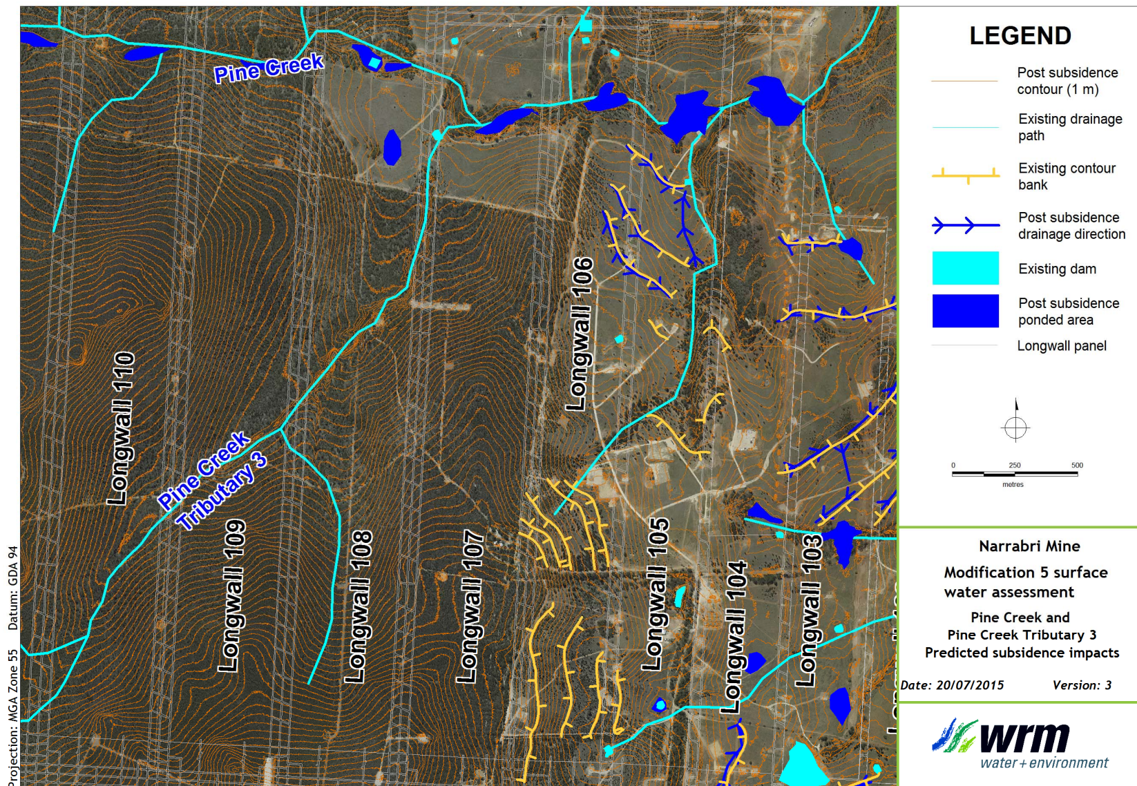
Figure 7.1 - Predicted subsidence impacts, Pine Creek and Pine Creek Trib. 3
