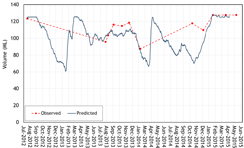
Figure A.1 - Observed and predicted volume in Dam A1, July 2012 to April 2015
