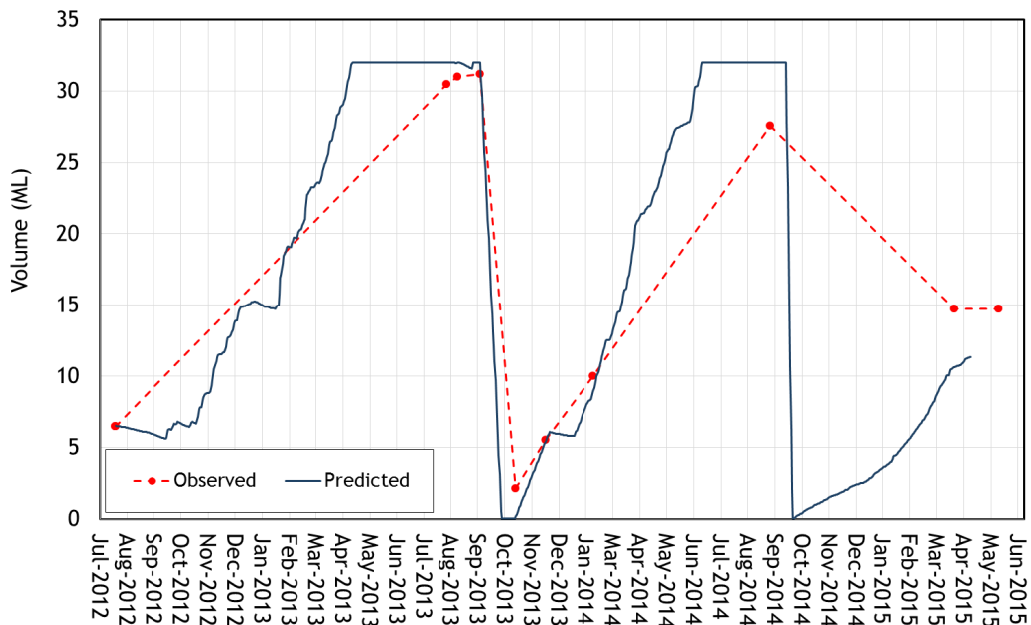
Figure A.5 - Observed and predicted volume in Dam A3, July 2012 to April 2015
