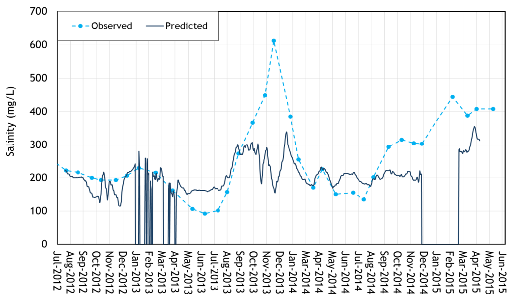
Figure A.8 - Observed and predicted salinity in Dam B1, July 2012 to April 2015
