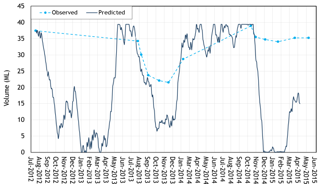
Figure A.7 - Observed and predicted volume in Dam B1, July 2012 to April 2015
