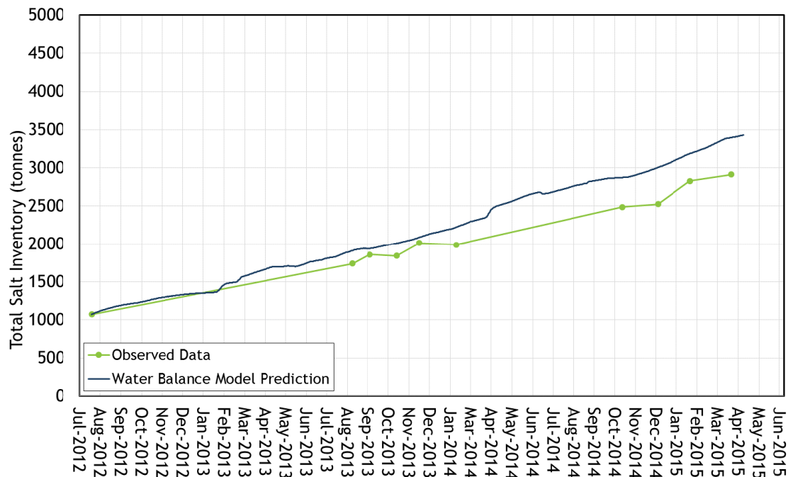
Figure 6.2 - Water balance model calibration results, total site salt inventory
