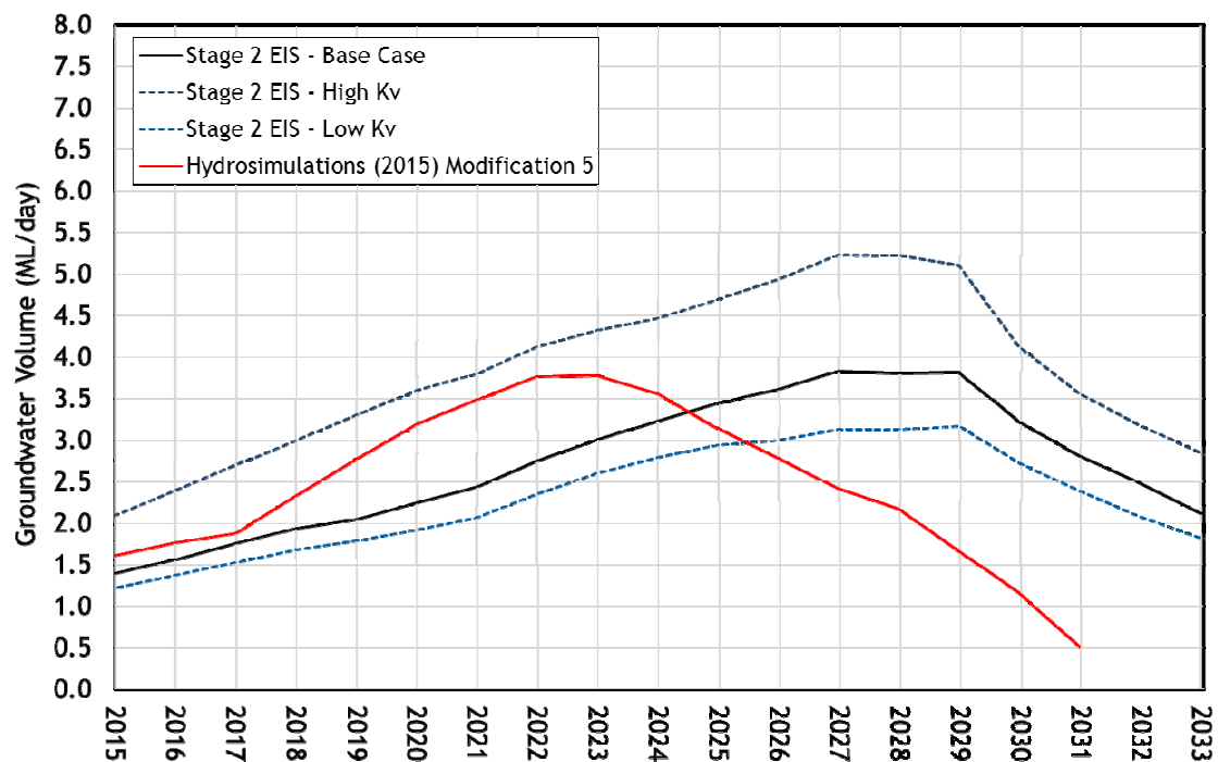
Figure 5.2 - Comparison of Hydrosimulations (2015) predicted Modification groundwater inflows and Aquaterra (2009) predicted groundwater inflows
