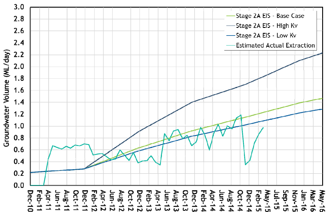
Figure 4.7 - Comparison of Aquaterra (2009) Stage 2 Environmental Impact Statement (EIS) groundwater inflow predictions and estimation of actual groundwater inflows
