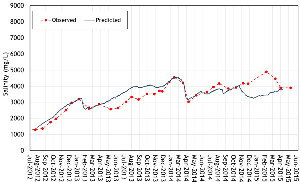
Figure A.2 - Observed and predicted salinity in Dam A1, July 2012 to April 2015
