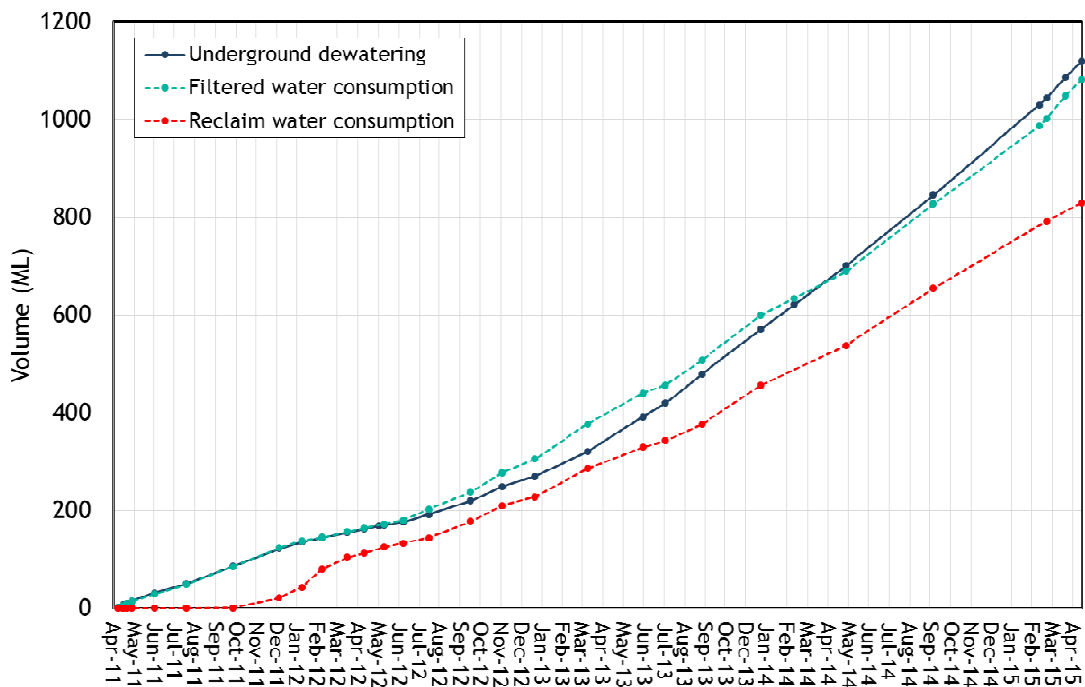
Figure 4.6 - Historical water consumption and underground dewatering, April 2011 to April 2015
