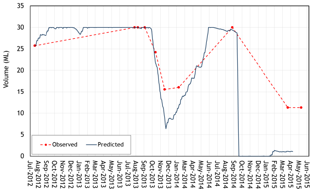
Figure A.3 - Observed and predicted volume in Dam A2, July 2012 to April 2015
