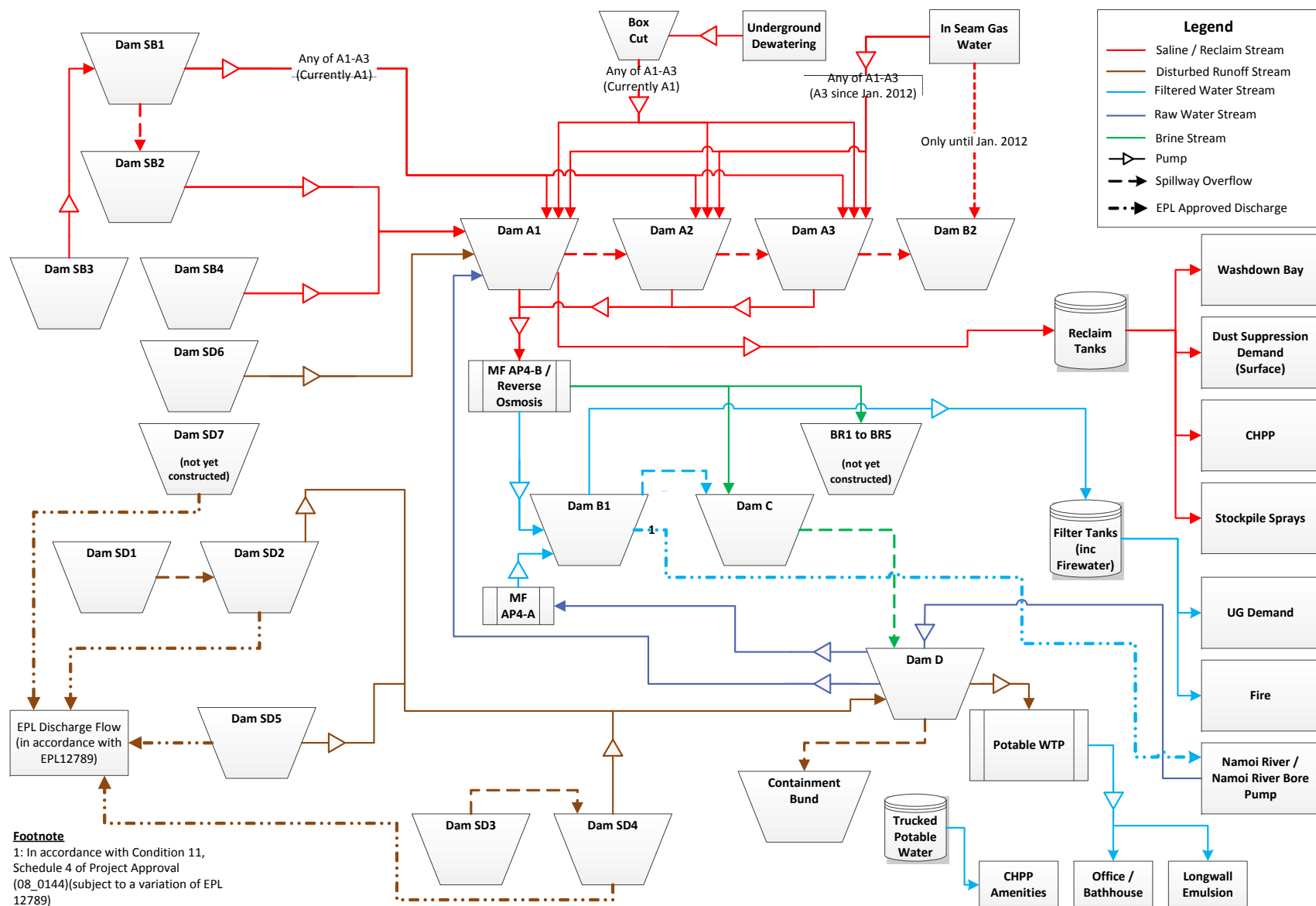
Figure 4.4 - Existing/approved site water management system schematic
