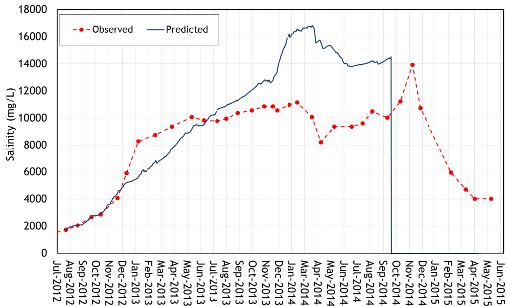
Figure A.4 - Observed and predicted salinity in Dam A2, July 2012 to April 2015
