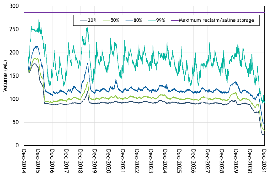
Figure 6.4 - Predicted storage inventory in the saline/reclaim dams A1, A2 A3, SB1, SB2, SB3 and SB4
