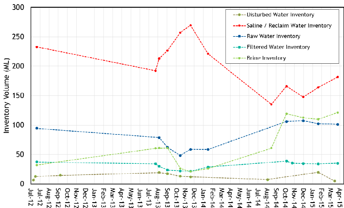
Figure 4.5 - Historical behaviour of site water inventory, July 2012 to April 2015
