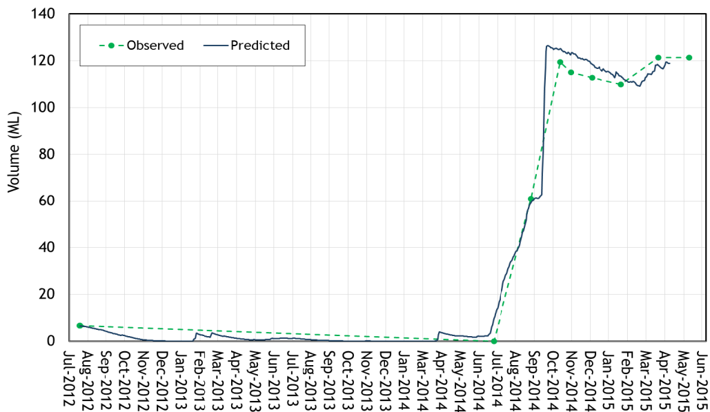
Figure A.11 - Observed and predicted volume in Dam C, July 2012 to April 2015
