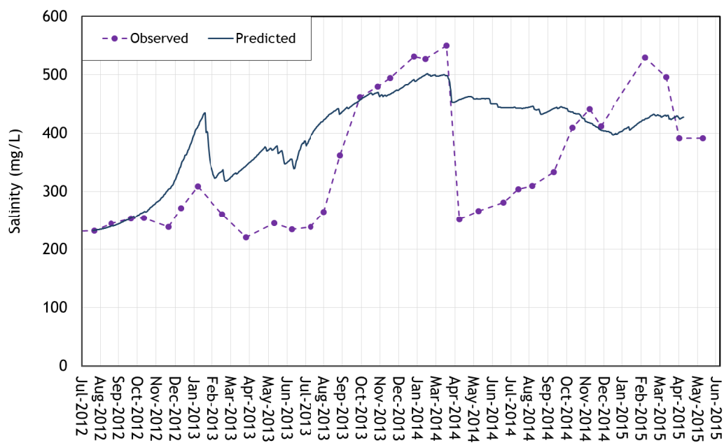
Figure A.14 - Observed and predicted salinity in Dam D, July 2012 to April 2015
