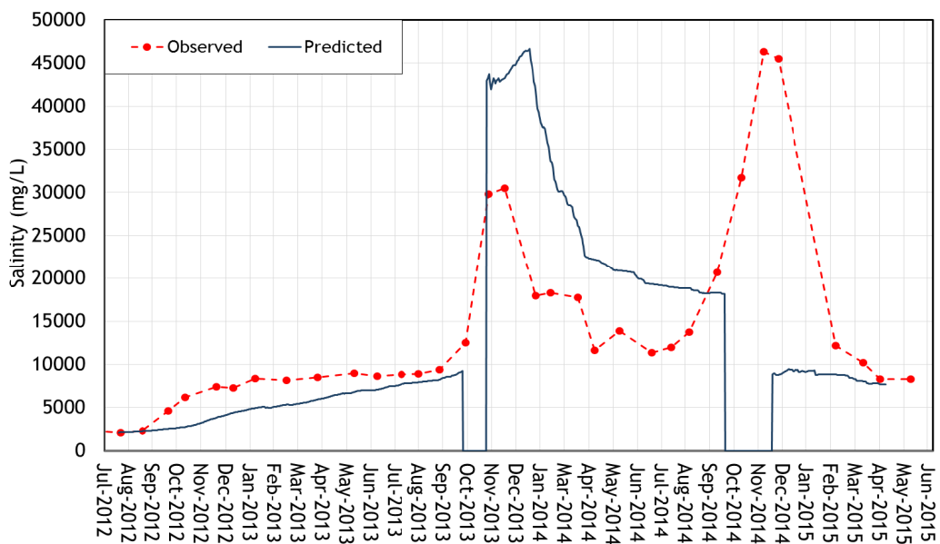
Figure A.6 - Observed and predicted salinity in Dam A3, July 2012 to April 2015
