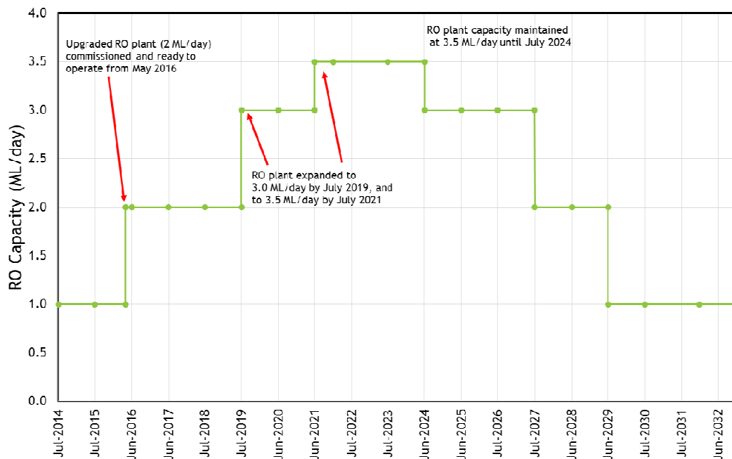
Figure 6.3 - Proposed RO plant capacity
