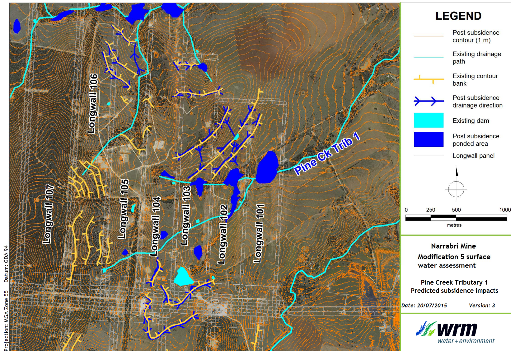
Figure 7.2 - Predicted subsidence impacts, Pine Creek Trib. 1
