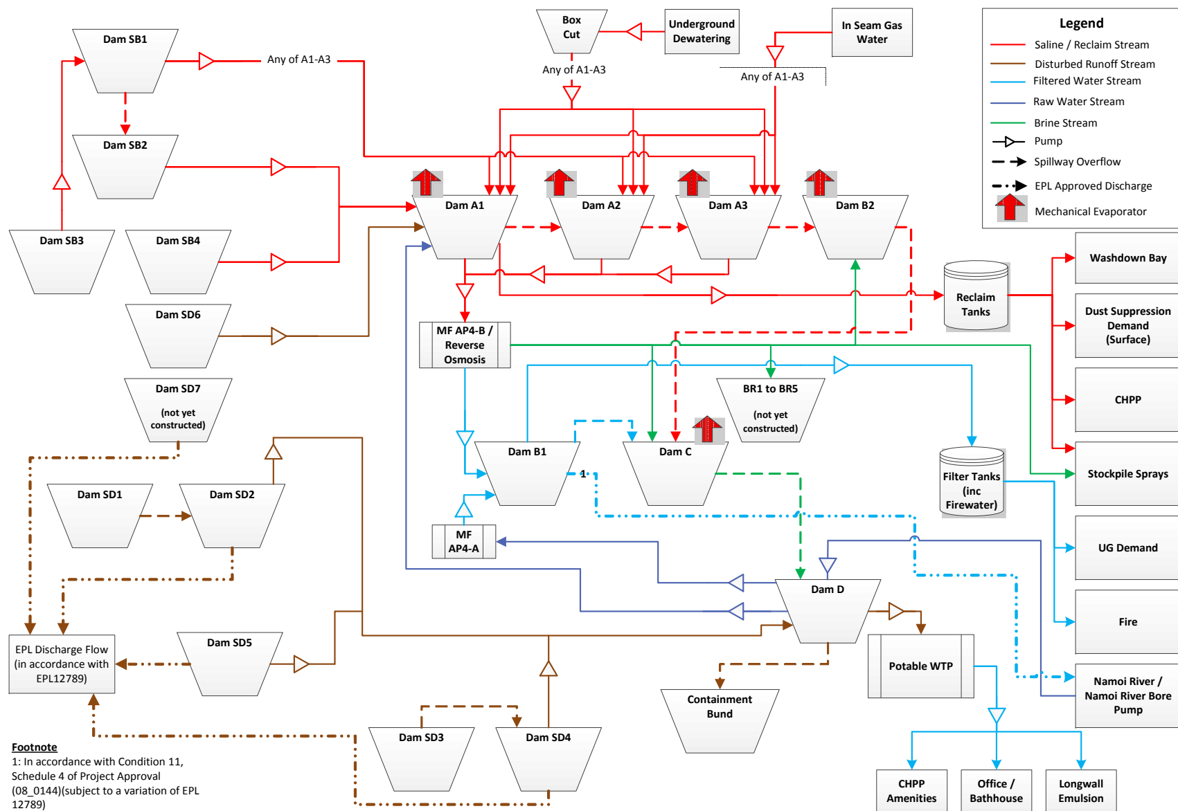
Figure 5.1 - Modified water management system schematic
