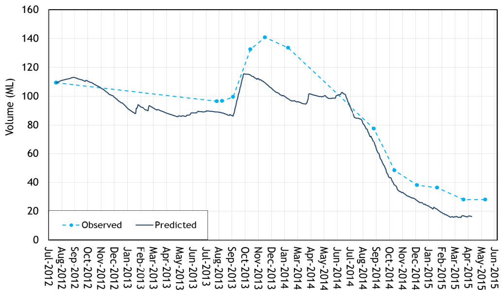
Figure A.9 - Observed and predicted volume in Dam B2, July 2012 to April 2015
