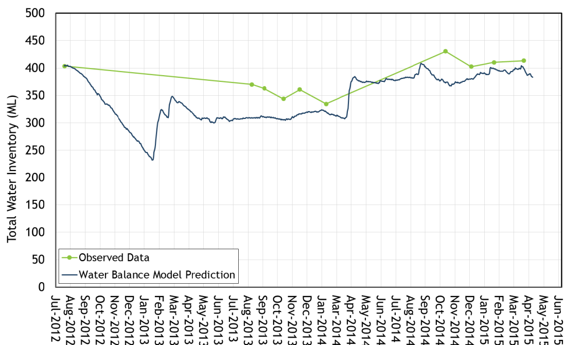
Figure 6.1 - Water balance model calibration results, total site water inventory
