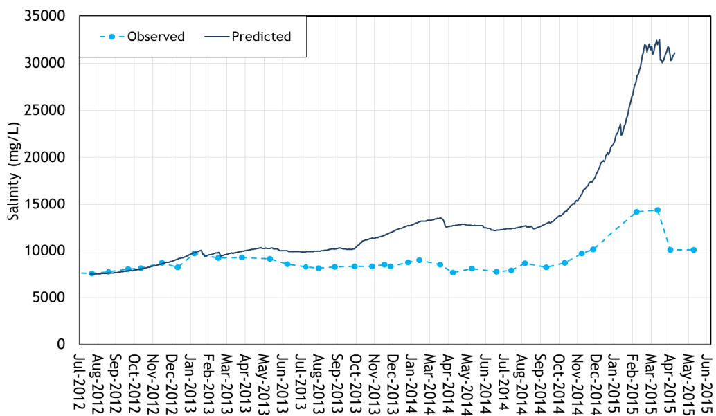
Figure A.10 - Observed and predicted salinity in Dam B2, July 2012 to April 2015
