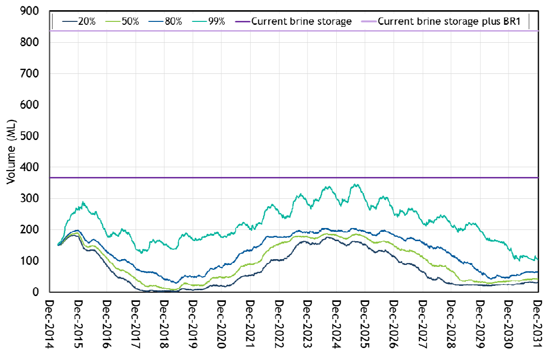
Figure 6.5 - Predicted storage inventory in the brine storage dams B2, C and BR1 (not yet constructed)
