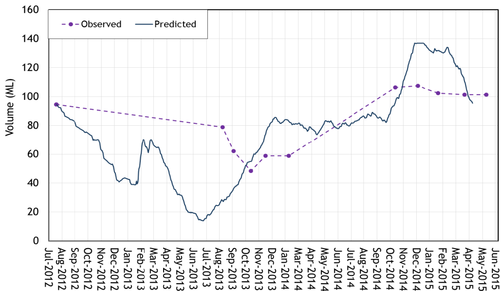
Figure A.13 - Observed and predicted volume in Dam D, July 2012 to April 2015
