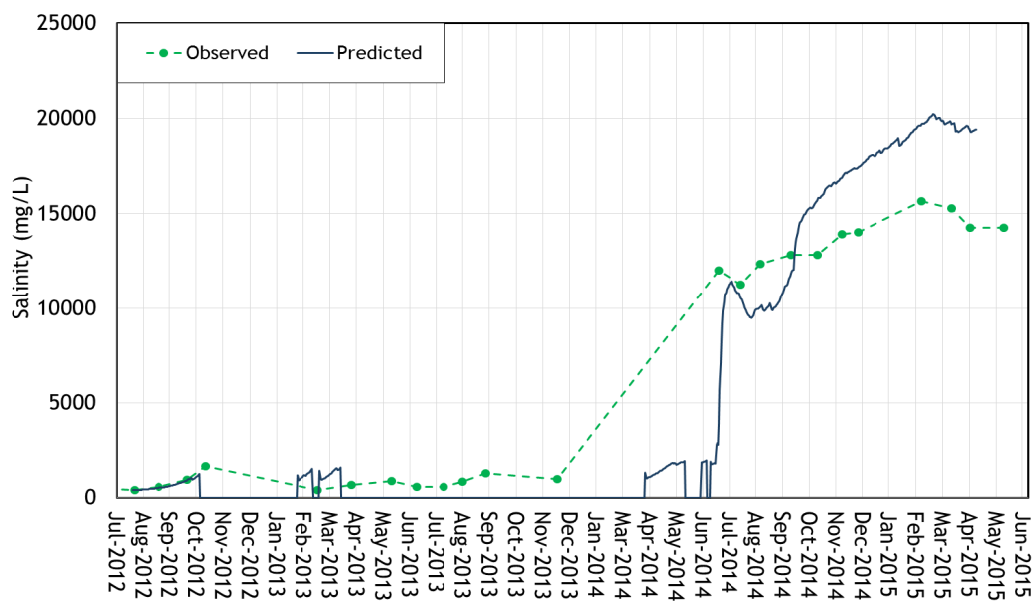
Figure A.12 - Observed and predicted salinity in Dam C, July 2012 to April 2015
