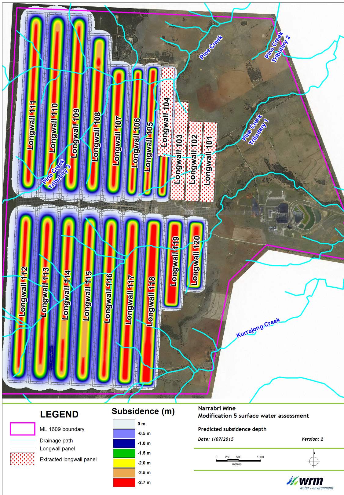
Figure 5.3 - Predicted Modification subsidence depths (Source: Ditton Geotechnical Services, 2015)
