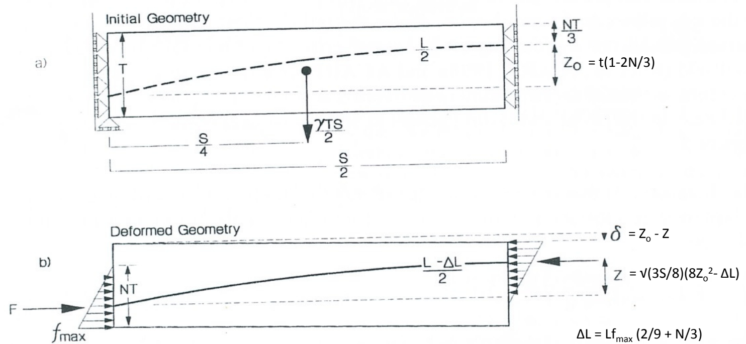
Fig. 5. Voussoir beam (half-span shown) and nomenclature.
